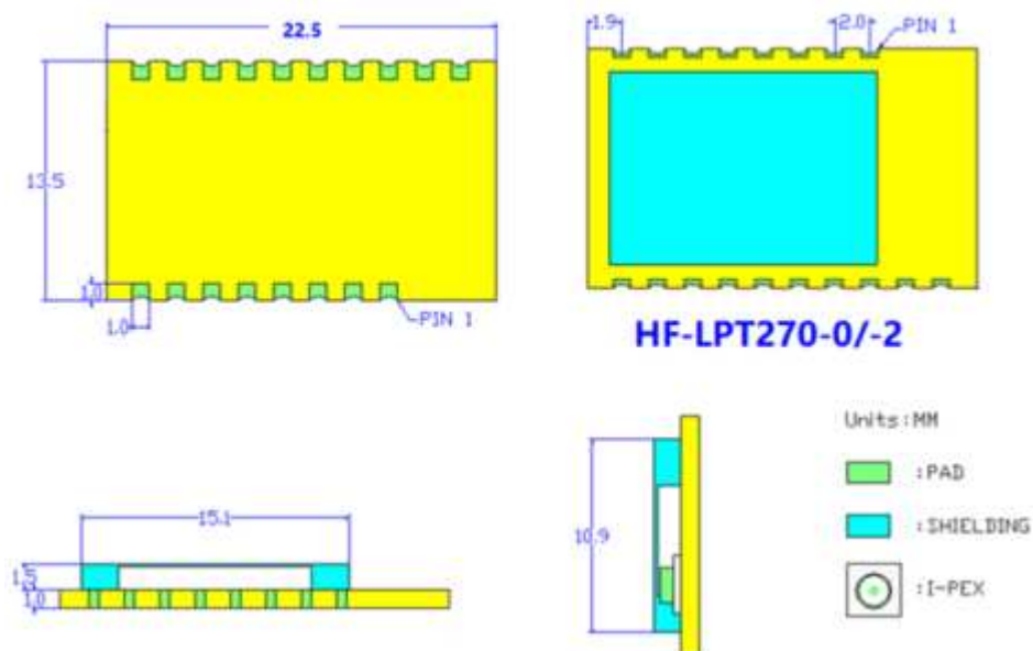
Figure 3. HF-LPT270-0(F) Mechanical Dimension
