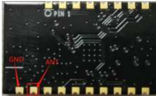
Figure 2. HF-LPT270-0(F)-2 Antenna PAD Out
