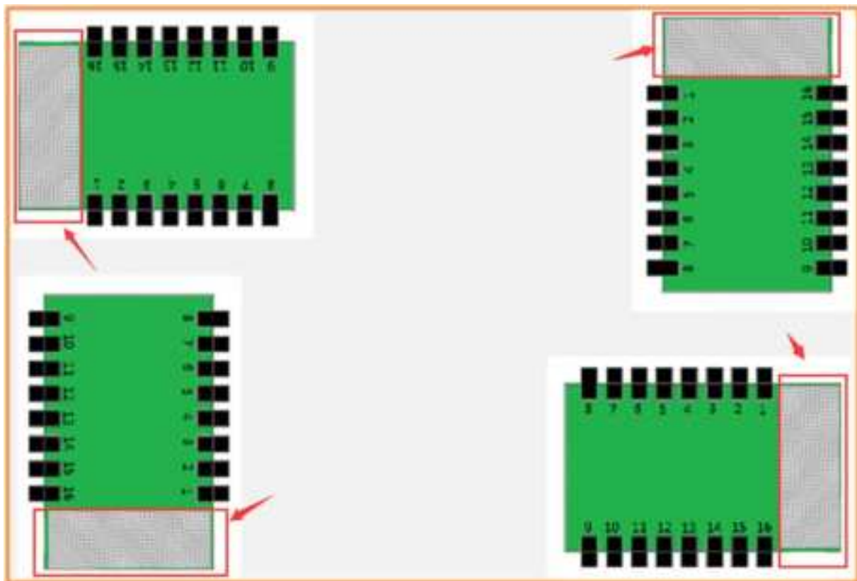
Figure 4. Suggested Module Placement Region
