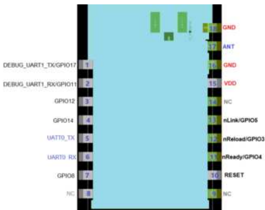
Figure 1. HF-LPT270-0(F) Pins Map
