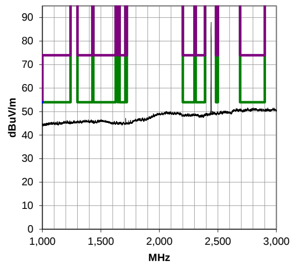
1000-3000 MHz, Run 43
