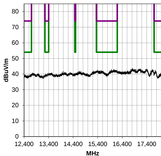
12400-18000 MHz, Run 46
