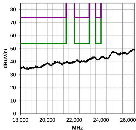
18000-26500 MHz, Run 37
