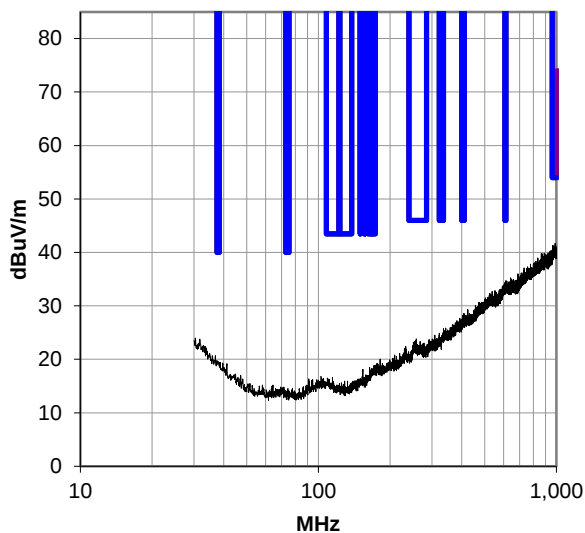
30-1000 MHz, Run 60
