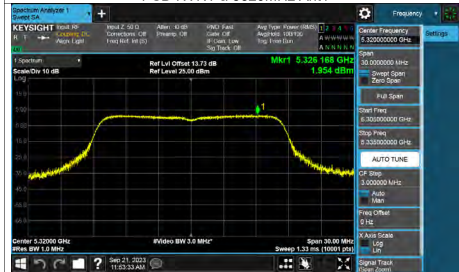
PSD NVNT a 5320MHz Ant1
