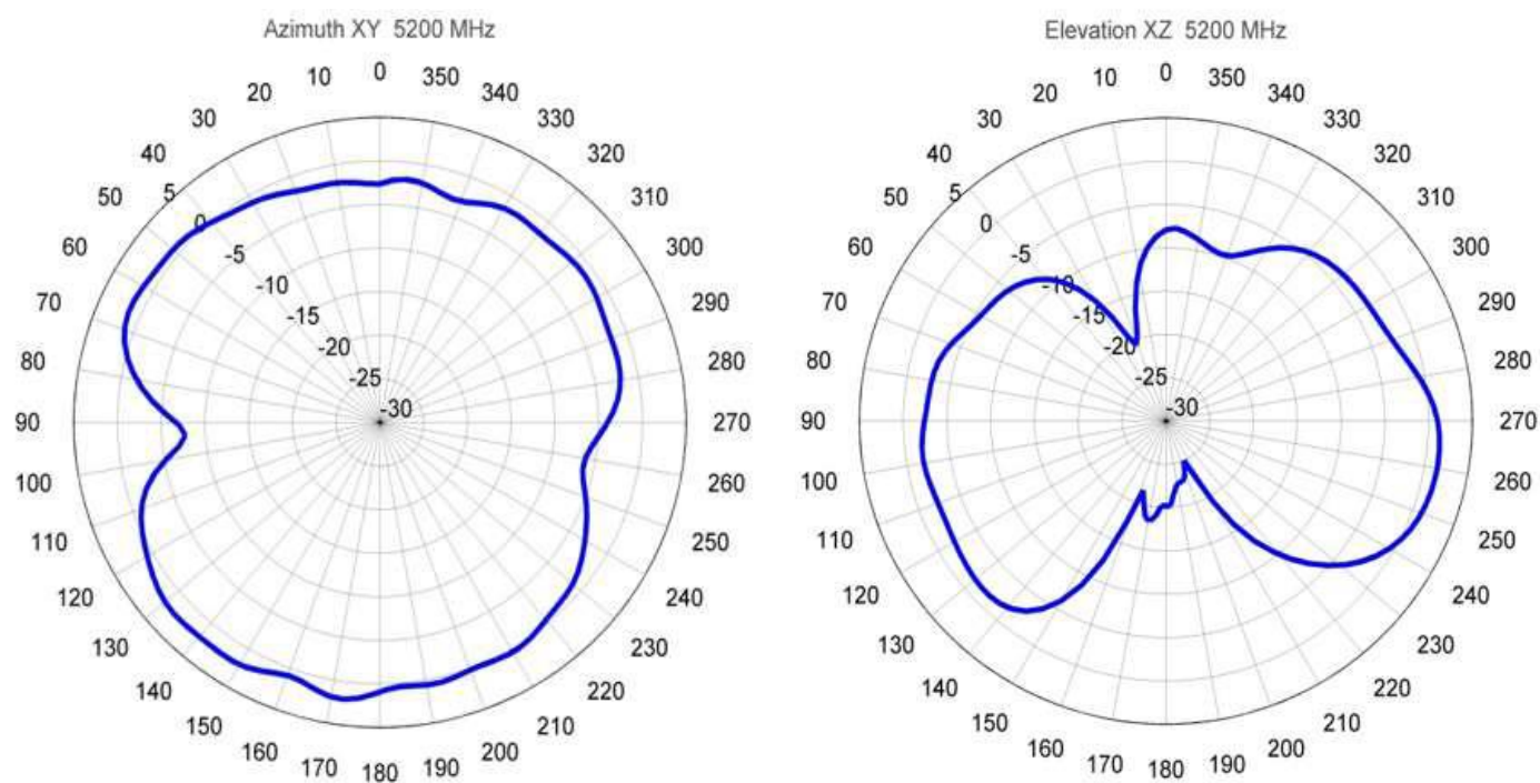
Figure 4: Model N03SGABA Radiation Patterns at 5.2 GHz
