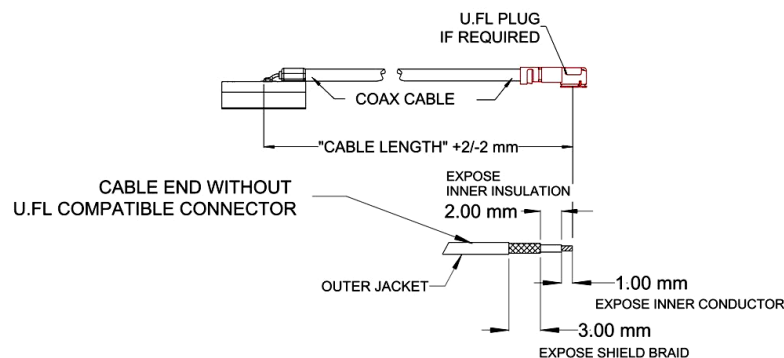
Figure 7: N03SGABA with connector or stripped cable
