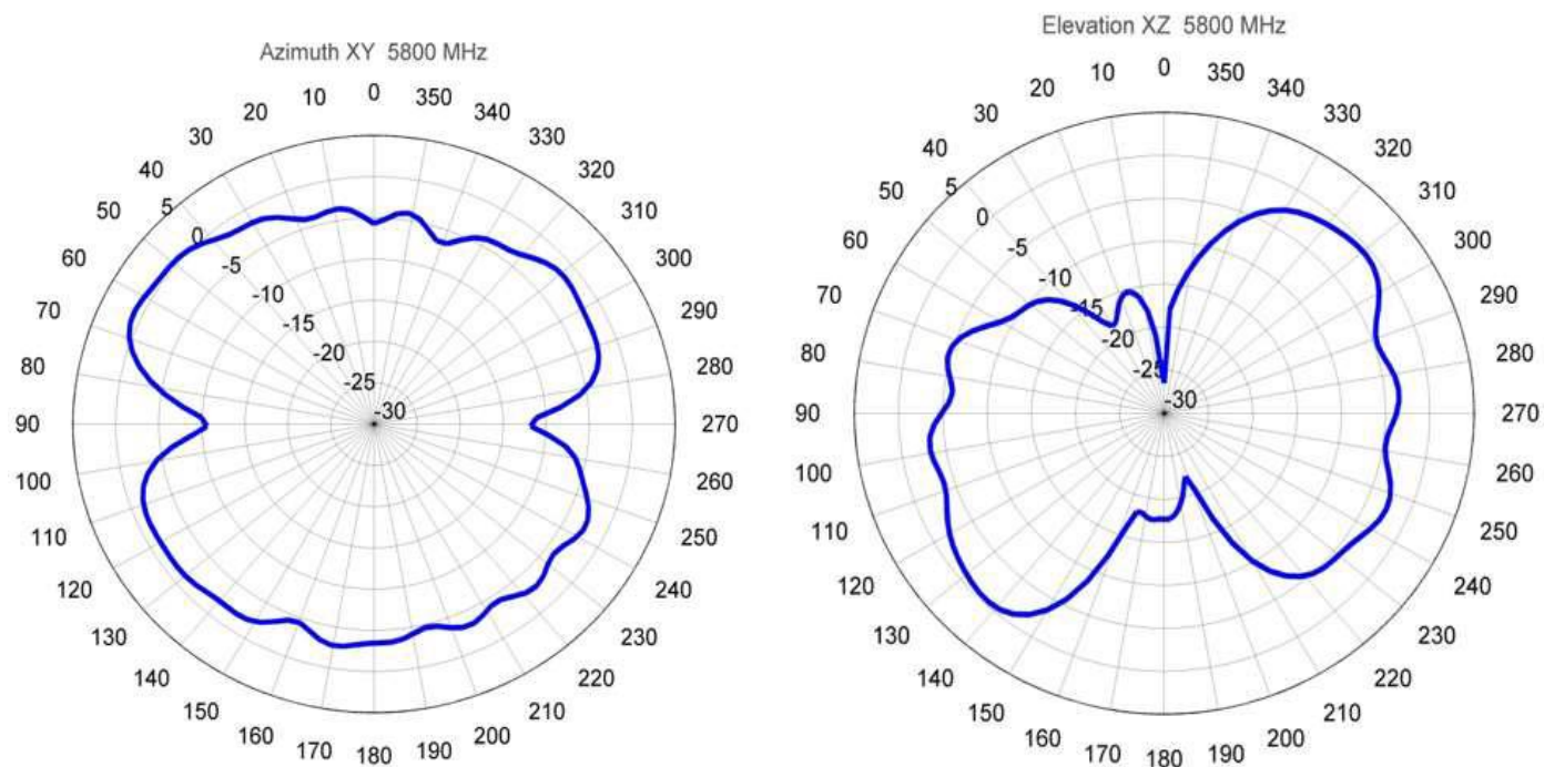
Figure 5: Model N03SGABA Radiation Patterns at 5.8 GHz
