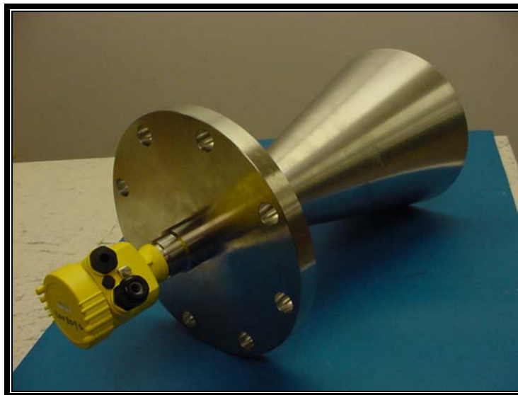
Photograph 25: EUT with 21.0 dBi Horn Antenna
