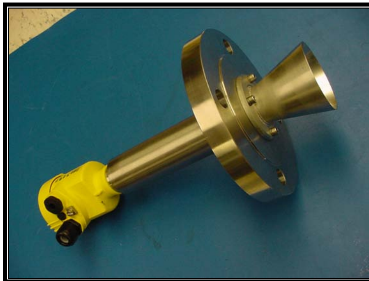
Photograph 23: EUT with 10.0 dBi Horn Antenna
