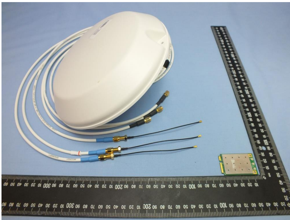
EUT with 2dBi Omni antenna
