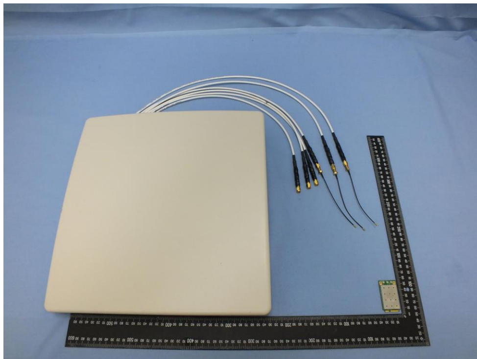
EUT with 5.5dBi Panel antenna
