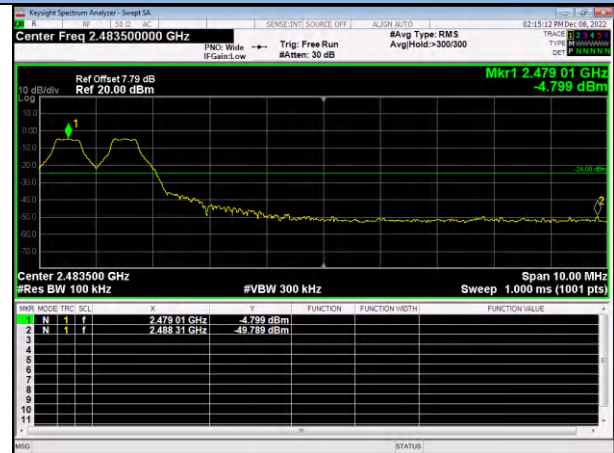
GFSK / Hopping
