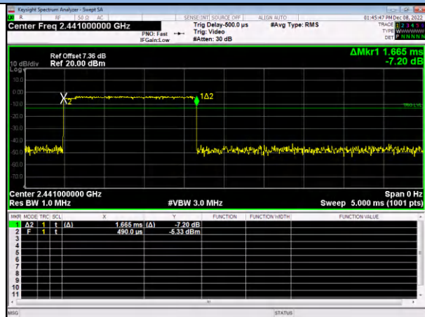
π/4-DQPSK / 2-DH3
