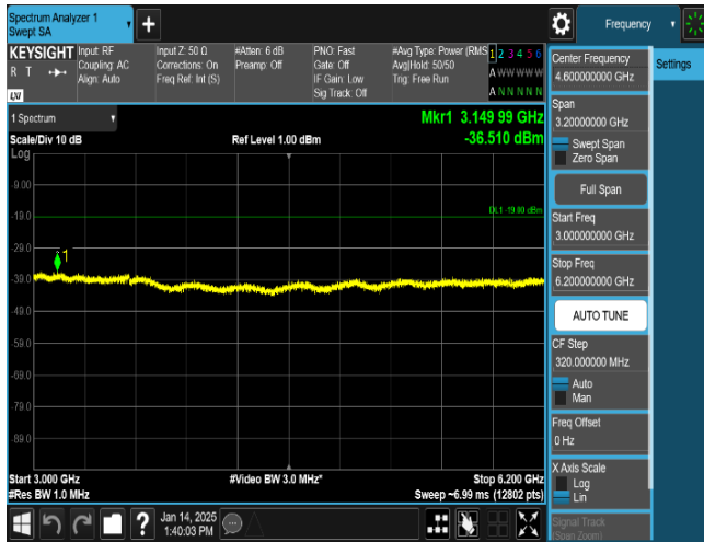
Plot 8-73. Conducted Spurious Emission Plot 3 GHz to 6.2 GHz (LTE_B66_1C_5M_QPSK - High Channel, Port 3)
