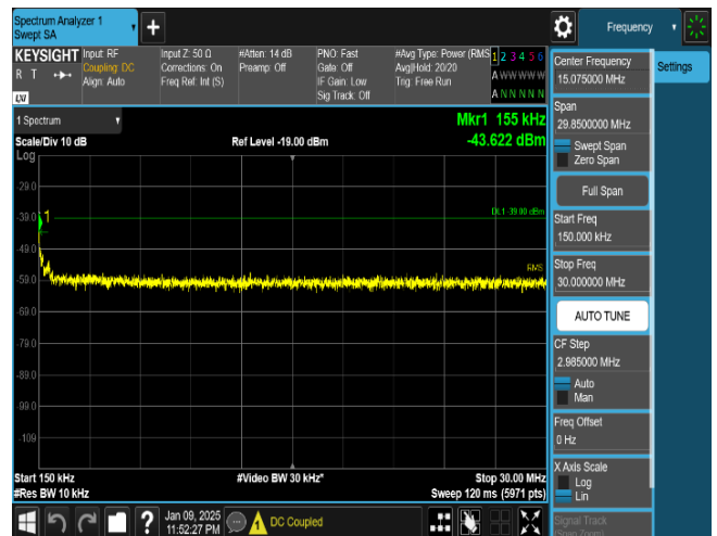
Plot 8-77. Conducted Spurious Emission Plot 150 kHz to 30 MHz (LTE_B66_1C_10M_256QAM - High Channel, Port 0)
