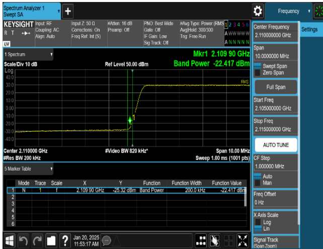
Plot 8-57. Band Edge Emission Summary Data Plot (NR_n66_1C_20M_256QAM - Low Edge, Port 3)
