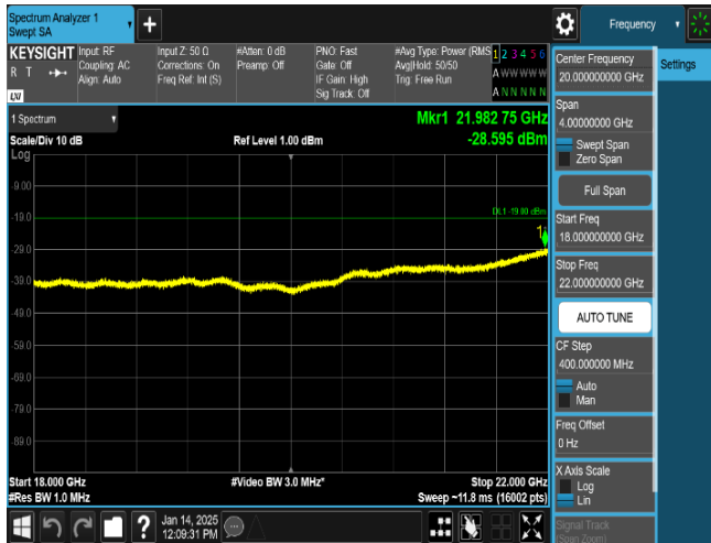
Plot 8-84. Conducted Spurious Emission Plot 18 GHz to 22 GHz
