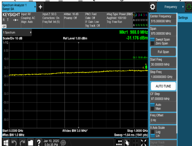
Plot 8-87. Conducted Spurious Emission Plot 30 MHz to 1 GHz
