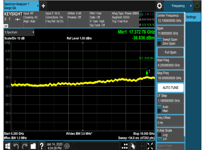
Plot 8-83. Conducted Spurious Emission Plot 6.2 GHz to 18 GHz (LTE_B66_1C_10M_256QAM - High Channel, Port 0)
