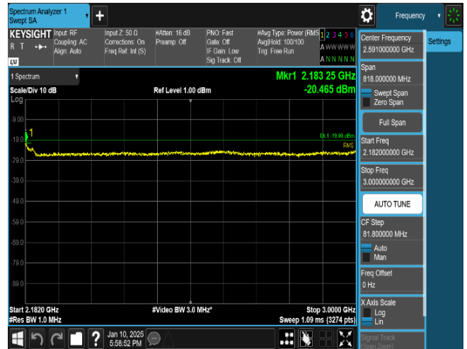
Plot 8-90. Conducted Spurious Emission Plot 2.182 GHz to 3 GHz (LTE_B66_1C_15M_16QAM - High Channel, Port 0)
