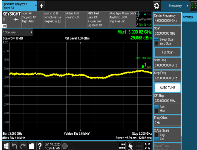
Plot 8-82. Conducted Spurious Emission Plot 3 GHz to 6.2 GHz (LTE_B66_1C_10M_256QAM - High Channel, Port 0)
