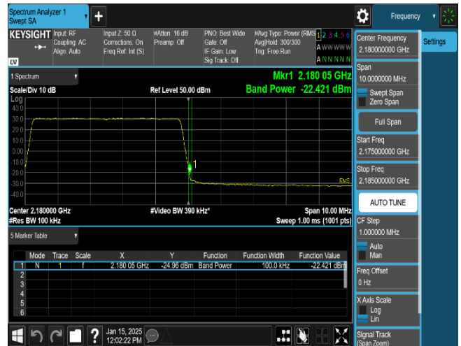
Plot 8-60. Band Edge Emission Summary Data Plot (LTE_B66_2C_5M+5M_QPSK - High Edge, Port 0)
