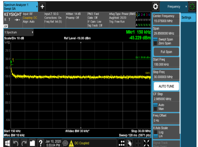
Plot 8-86. Conducted Spurious Emission Plot 150 kHz to 30 MHz
