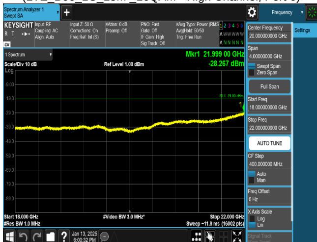
Plot 8-93. Conducted Spurious Emission Plot 18 GHz to 22 GHz (LTE_B66_1C_15M_16QAM - High Channel, Port 0)
