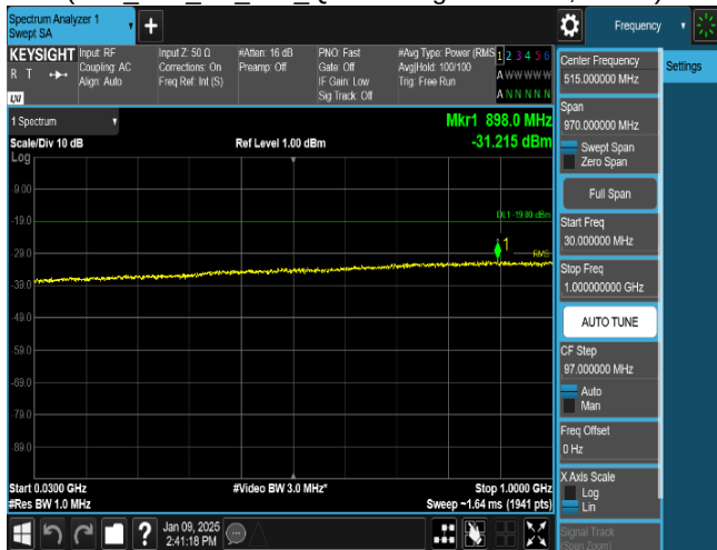
Plot 8-69. Conducted Spurious Emission Plot 30 MHz to 1 GHz (LTE_B66_1C_5M_QPSK - High Channel, Port 3)
