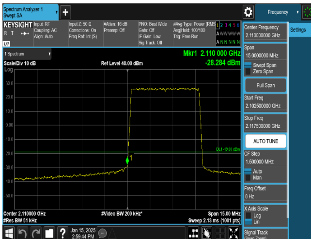
Plot 8-61. Band Edge Emission Summary Data Plot (LTE_B66_2NC_5M+5M_QPSK - Low Edge, Port 1)
