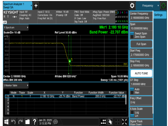
Plot 8-58. Band Edge Emission Summary Data Plot (NR_n66_1C_20M_256QAM - High Edge, Port 0)
