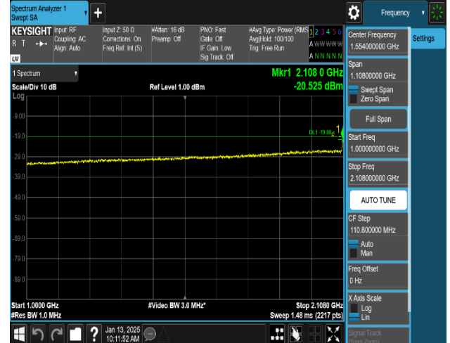
Plot 8-97. Conducted Spurious Emission Plot 1 GHz to 2.108 GHz
