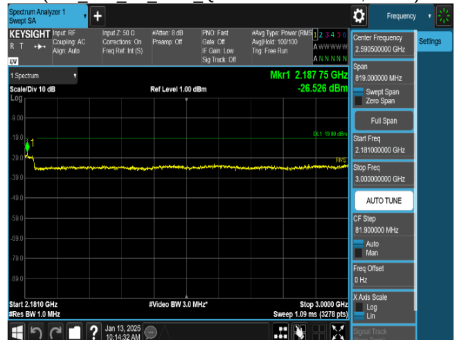
Plot 8-99. Conducted Spurious Emission Plot 2.181 GHz to 3 GHz
