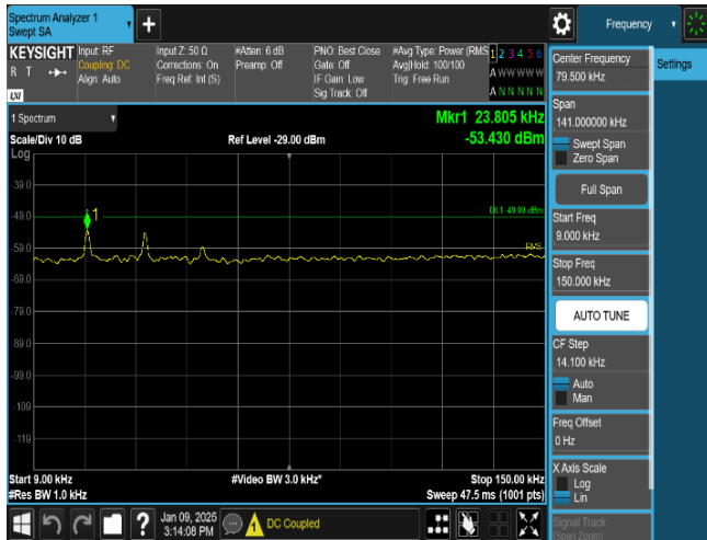
Plot 8-67. Conducted Spurious Emission Plot 9 kHz to 150 kHz (LTE_B66_1C_5M_QPSK - High Channel, Port 3)
