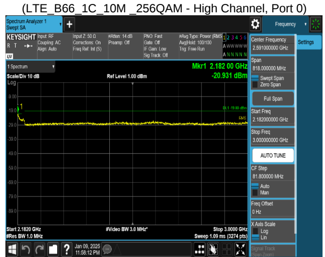
Plot 8-81. Conducted Spurious Emission Plot 2.182 GHz to 3 GHz (LTE_B66_1C_10M_256QAM - High Channel, Port 0)
