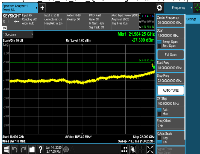
Plot 8-75. Conducted Spurious Emission Plot 18 GHz to 22 GHz (LTE_B66_1C_5M_QPSK - High Channel, Port 3)
