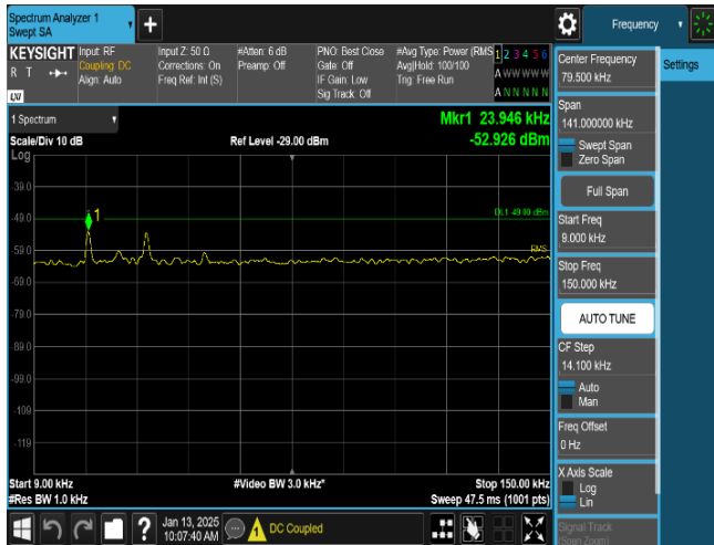
Plot 8-94. Conducted Spurious Emission Plot 9 kHz to 150 kHz
