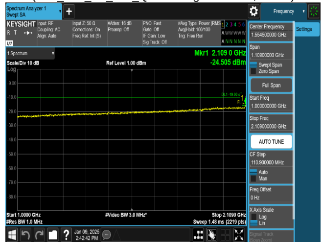
Plot 8-70. Conducted Spurious Emission Plot 1 GHz to 2.109 GHz (LTE_B66_1C_5M_QPSK - High Channel, Port 3)
