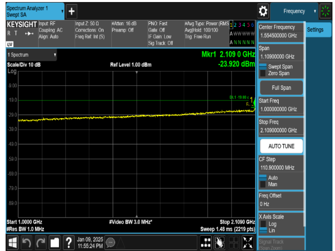
Plot 8-79. Conducted Spurious Emission Plot 1 GHz to 2.109 GHz
