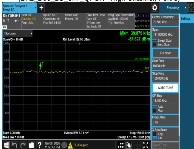
Plot 8-76. Conducted Spurious Emission Plot 9 kHz to 150 kHz (LTE_B66_1C_10M_256QAM - High Channel, Port 0)
