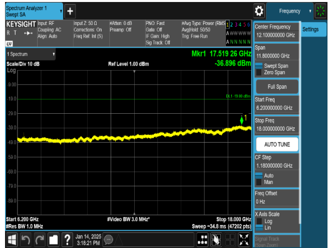
Plot 8-74. Conducted Spurious Emission Plot 6.2 GHz to 18 GHz (LTE_B66_1C_5M_QPSK - High Channel, Port 3)
