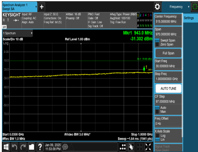
Plot 8-78. Conducted Spurious Emission Plot 30 MHz to 1 GHz
