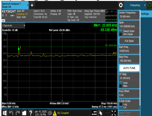
Plot 8-85. Conducted Spurious Emission Plot 9 kHz to 150 kHz
