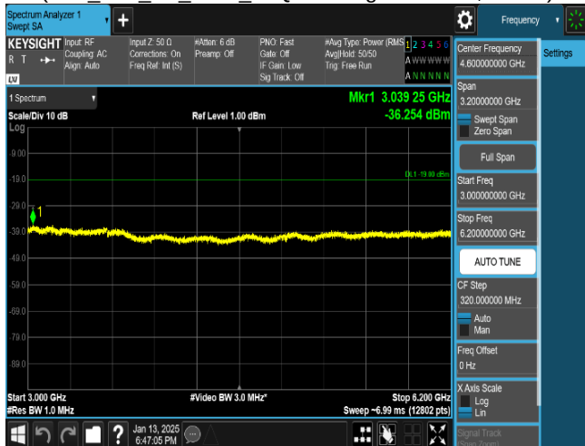
Plot 8-91. Conducted Spurious Emission Plot 3 GHz to 6.2 GHz (LTE_B66_1C_15M_16QAM - High Channel, Port 0)
