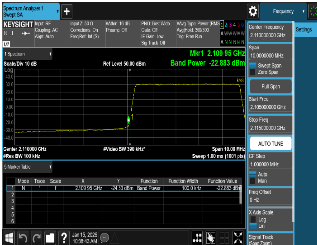
Plot 8-59. Band Edge Emission Summary Data Plot (LTE_B66_2C_5M+5M_QPSK - Low Edge, Port 1)
