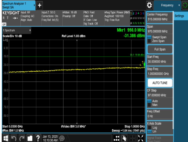
Plot 8-96. Conducted Spurious Emission Plot 30 MHz to 1 GHz
