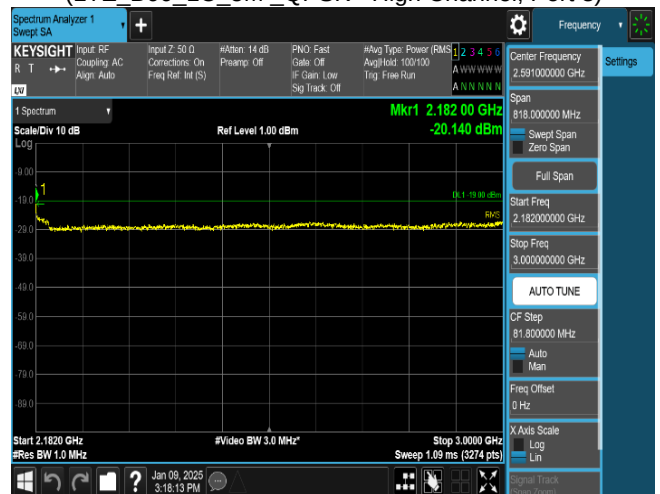
Plot 8-72. Conducted Spurious Emission Plot 2.182 GHz to 3 GHz (LTE_B66_1C_5M_QPSK - High Channel, Port 3)
