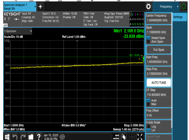
Plot 8-88. Conducted Spurious Emission Plot 1 GHz to 2.109 GHz
