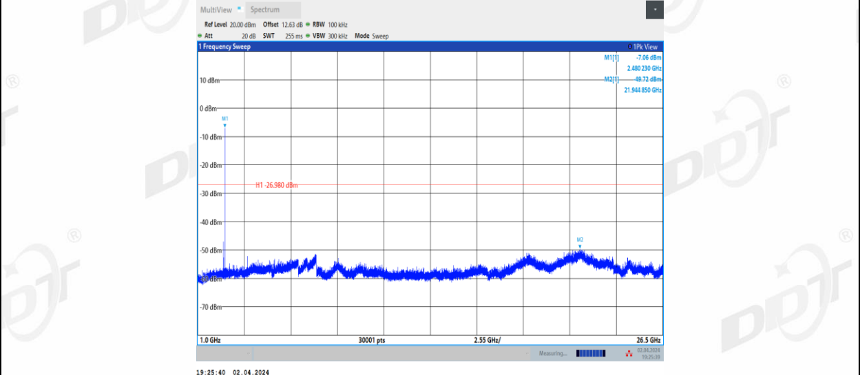
BLE_1M_Right side_2480_0~Reference
