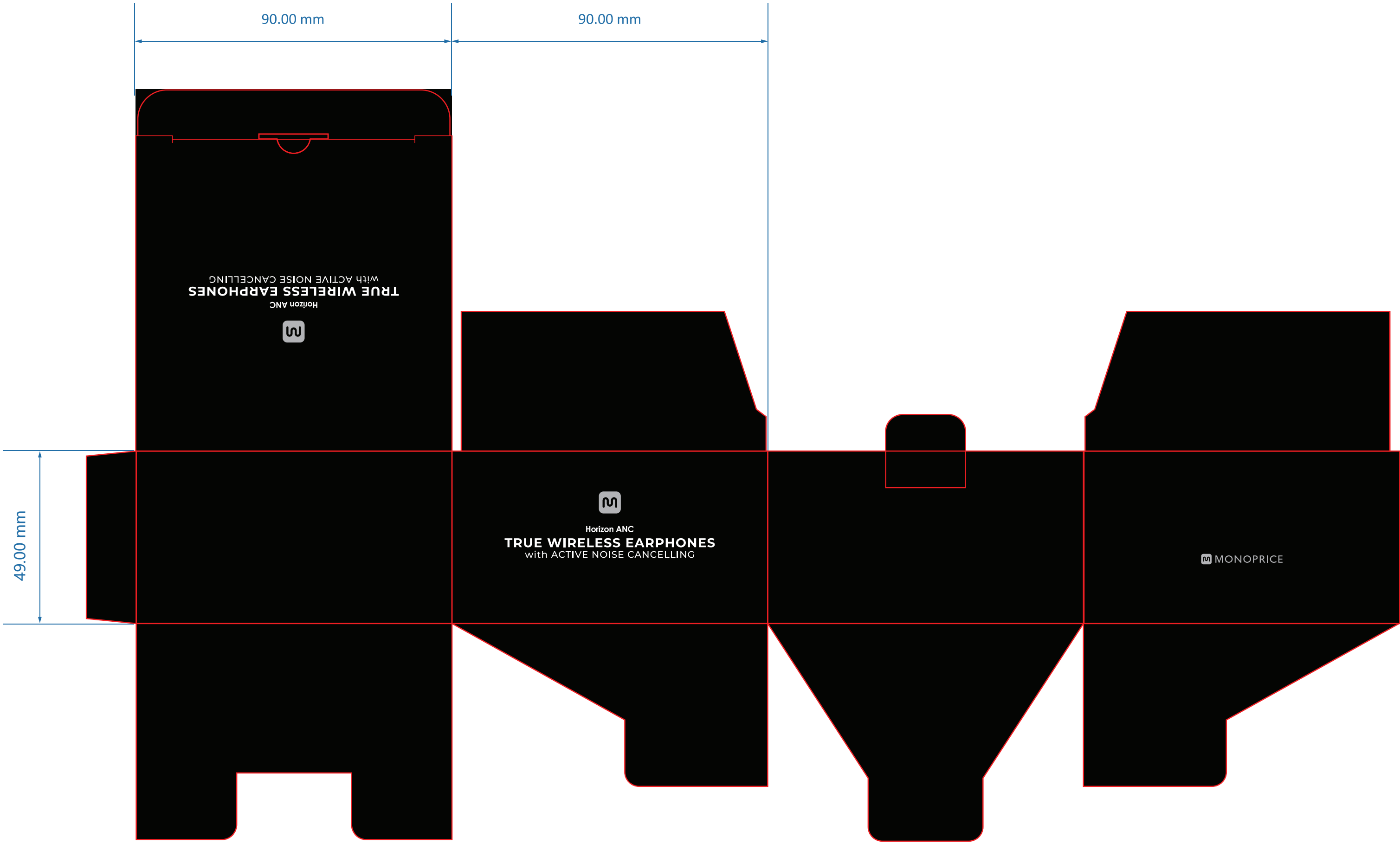
Folding box
