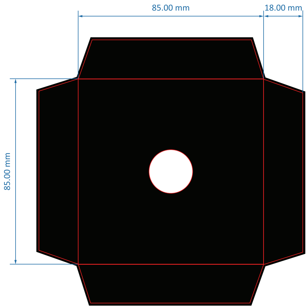
Inner box
