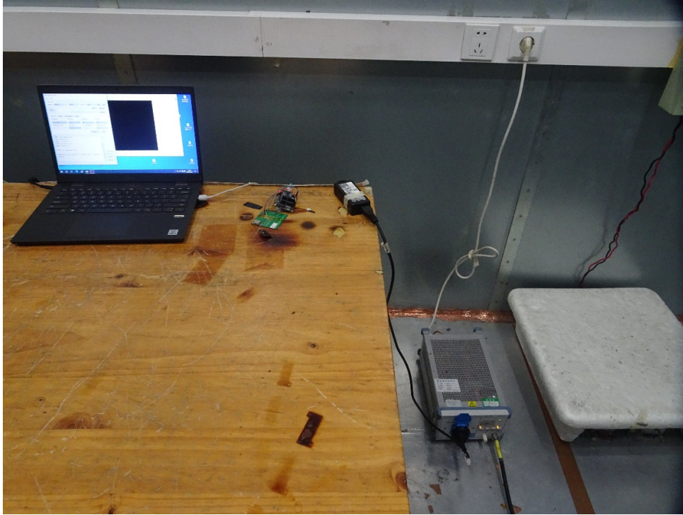
Picture 2 Conducted Emission Test Setup
