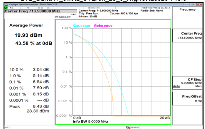
LTE_Band17_5MHz_64QAM_25_0_HighCH23825-713.5
