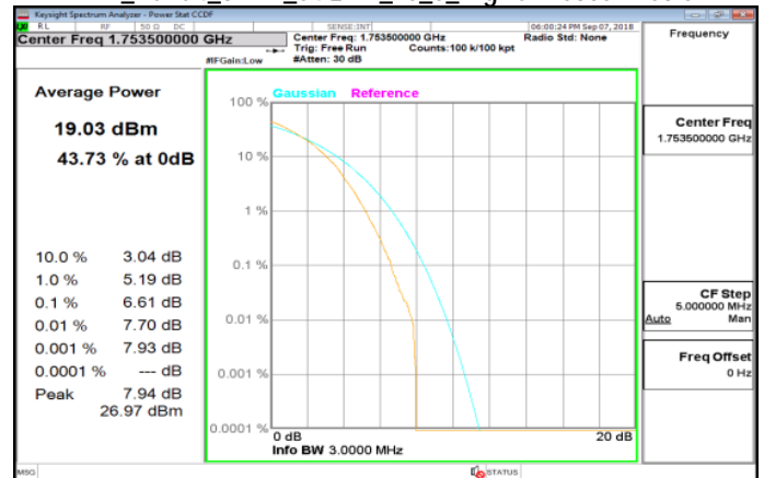
LTE_Band4_3MHz_64QAM_15_0_HighCH20385-1753.5
