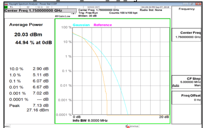
LTE_Band4_10MHz_64QAM_50_0_HighCH20350-1750
