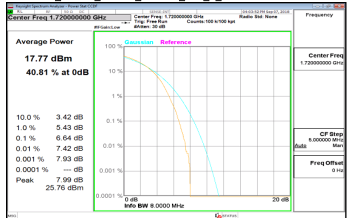
LTE_Band4_20MHz_64QAM_100_0_LowCH20050-1720
