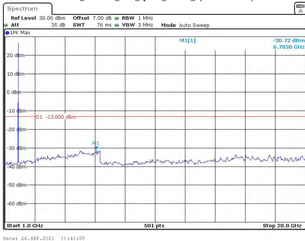
Band 2_1.4 MHz_Low_QPSK_RB6#0_2(1GHz-20GHz)
