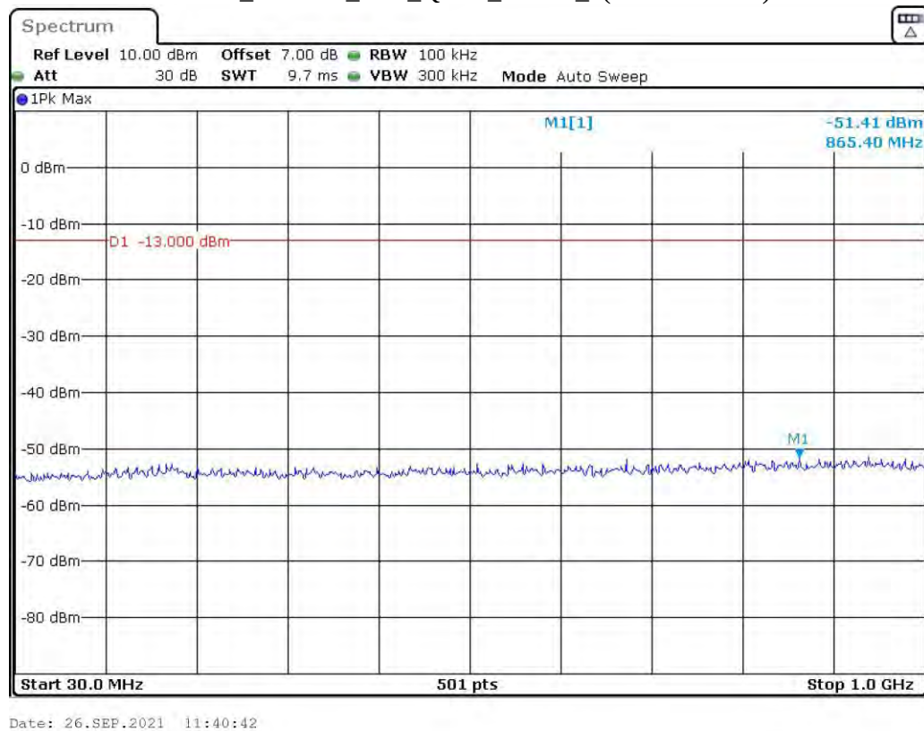
Band 2_1.4 MHz_Low_QPSK_RB6#0_1(30MHz-1GHz)
