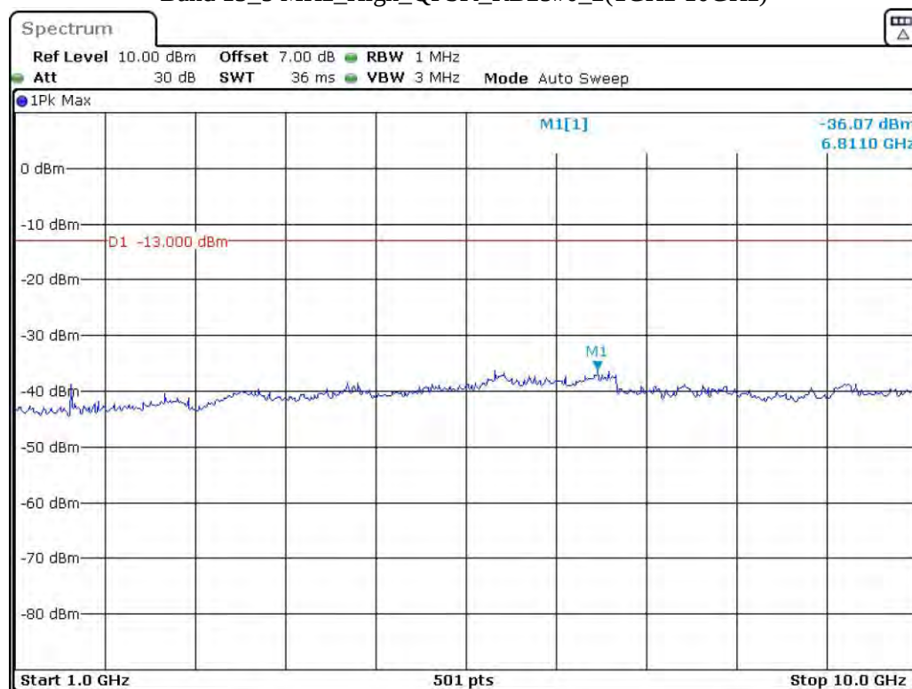
Band 13_5 MHz_High_QPSK_RB25#0_2(1GHz-10GHz)
