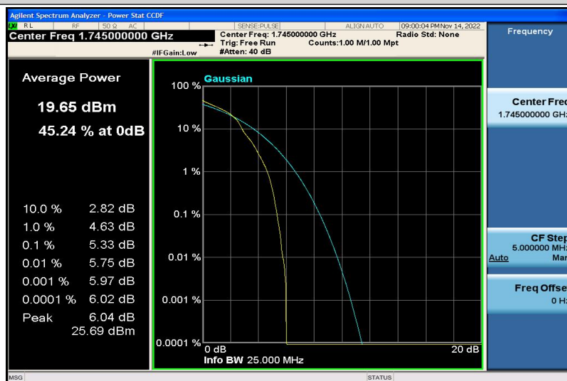
Band4-20MHz-16QAM-20300-1RB#0
