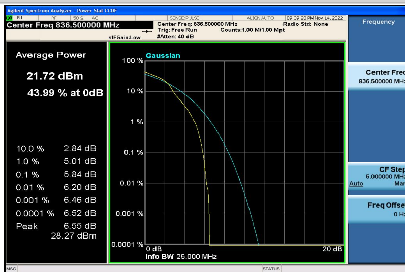
Band5-3MHz-16QAM-20525-1RB#0
