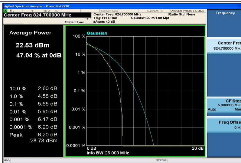
Band5-1.4MHz-QPSK-20407-1RB#0
