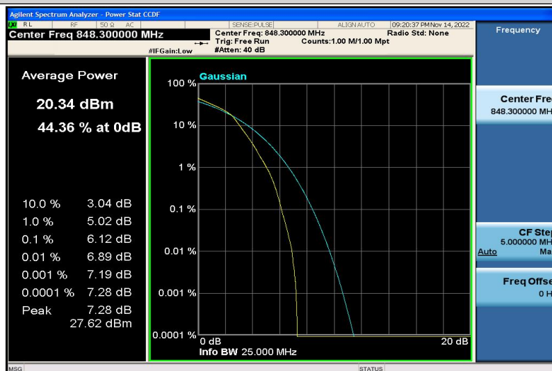
Band5-1.4MHz-16QAM-20643-6RB#0
