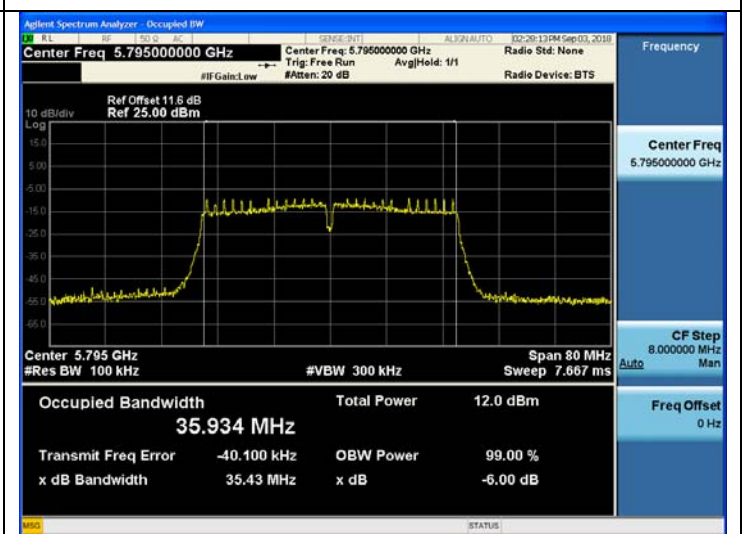
802.11ac_VHT40 UNII 3 BAND 6dB Bandwidth(CH.159)
