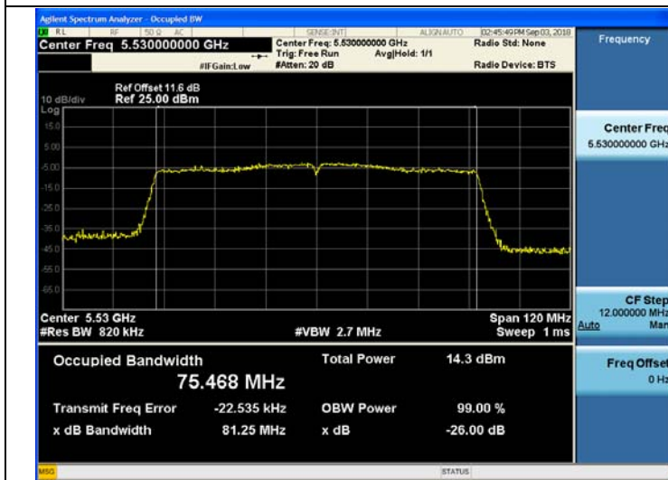
802.11ac_VHT80 UNII 2C BAND 26dB Bandwidth(CH 106)
