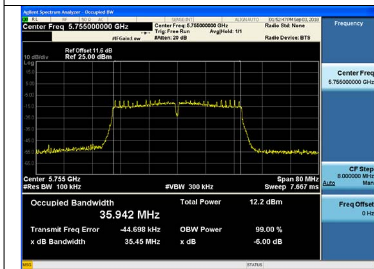
802.11n_40 MHz UNII 3 BAND 6dB Bandwidth (CH.151)
