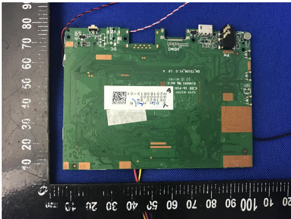
MAIN BOARD REAR VIEW (WITHOUT SHIELDING) (Innolux Screen)
