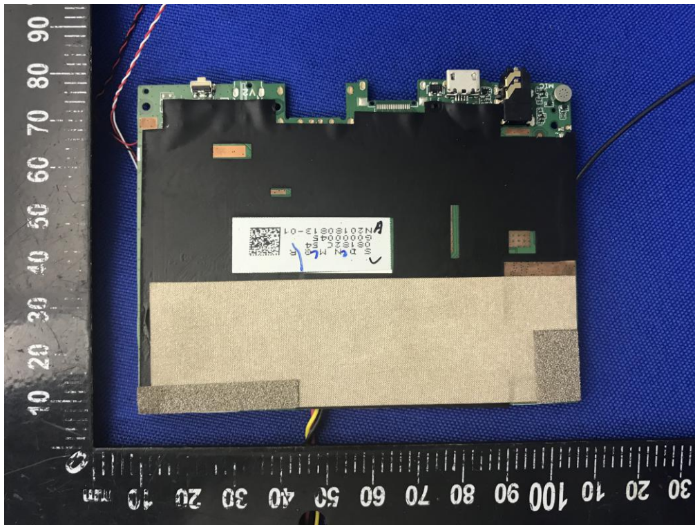
MAIN BOARD REAR VIEW (WITH SHIELDING) (BOE Screen)
