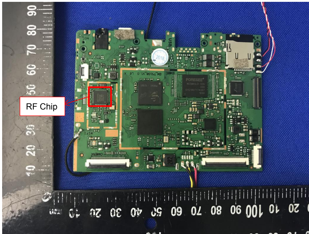
MAIN BOARD TOP VIEW (WITHOUT SHIELDING) (Innolux Screen)
