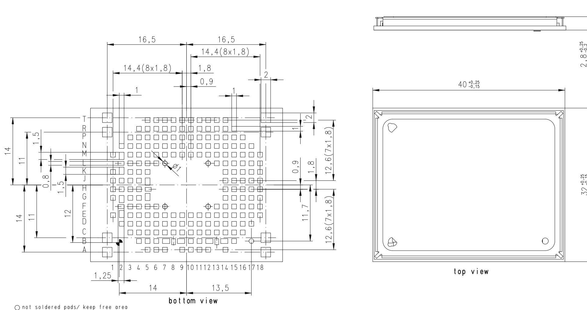
Figure 12: Dimensions of PLAS9-X (all dimensions in mm)
