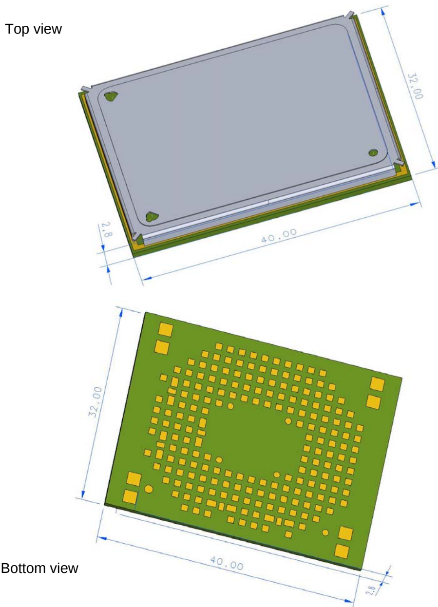
Figure 11: PLAS9-X – top and bottom view
