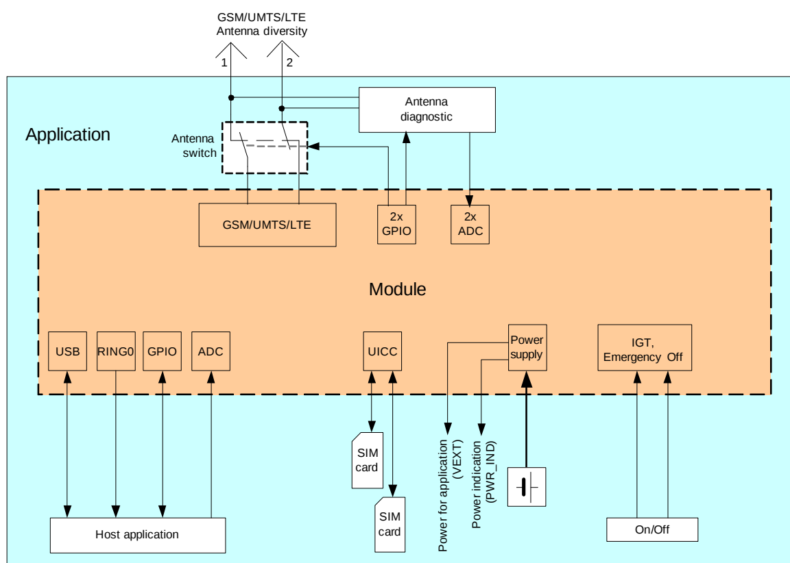
Figure 1: PLAS9-X system overview
