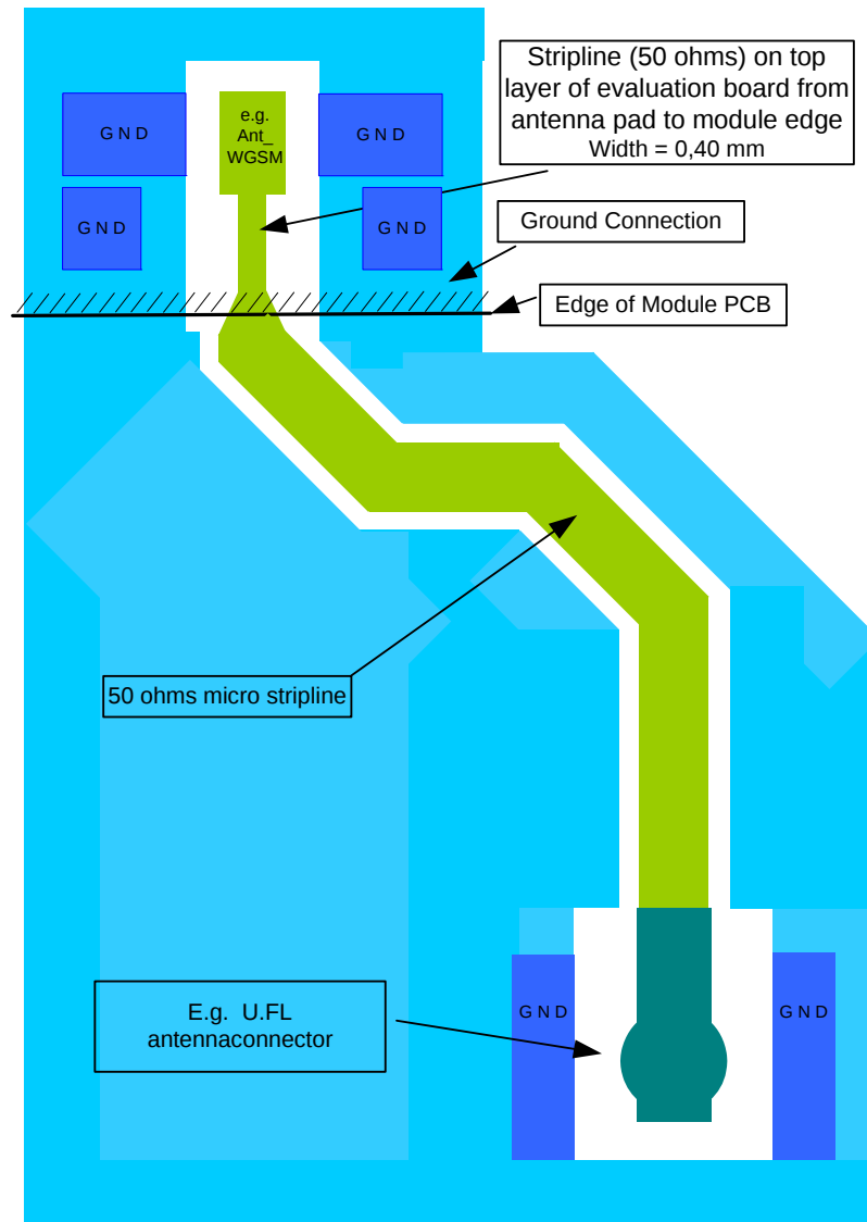
Figure 8: Routing to PLAS9-X evaluation module's RF connector
