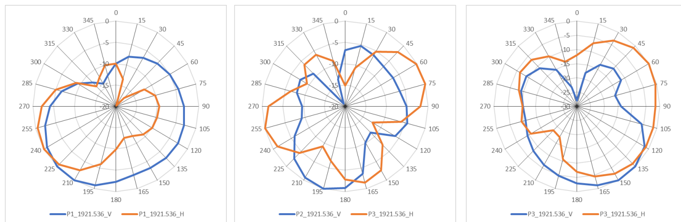
Figure 6: Radiation patterns 1921.536 MHz
