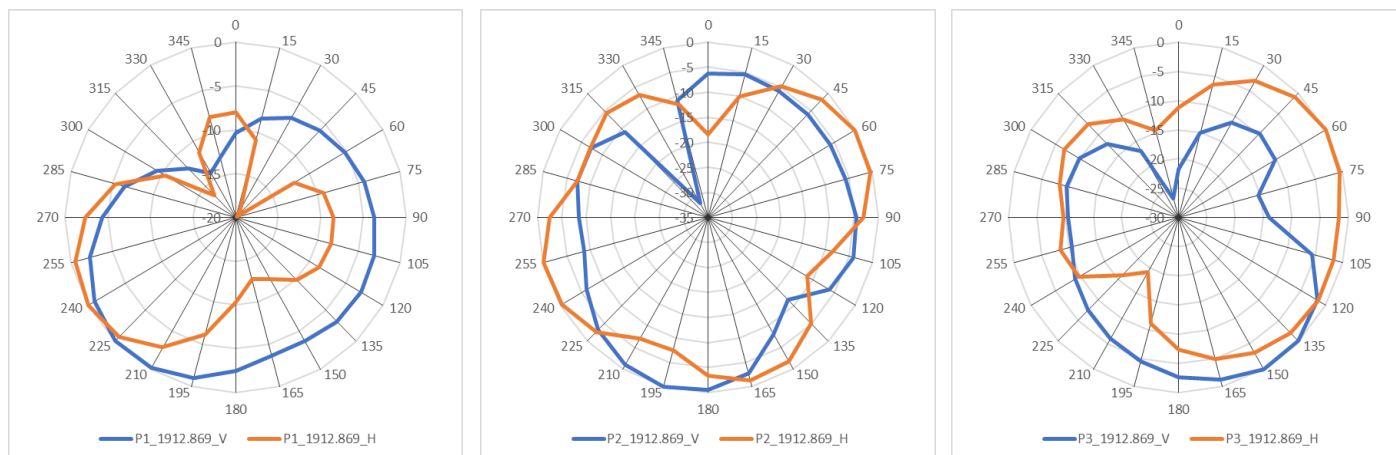
Figure 5: Radiation patterns 1912.869 MHz
