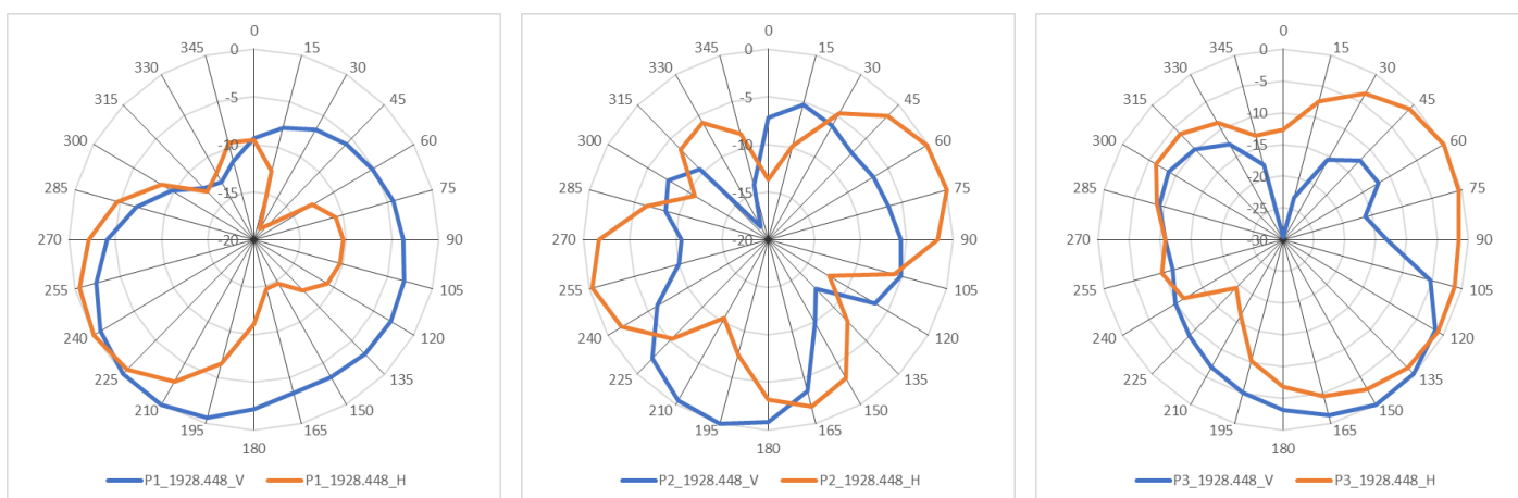
Figure 7: Radiation patterns 1928.448 MHz
