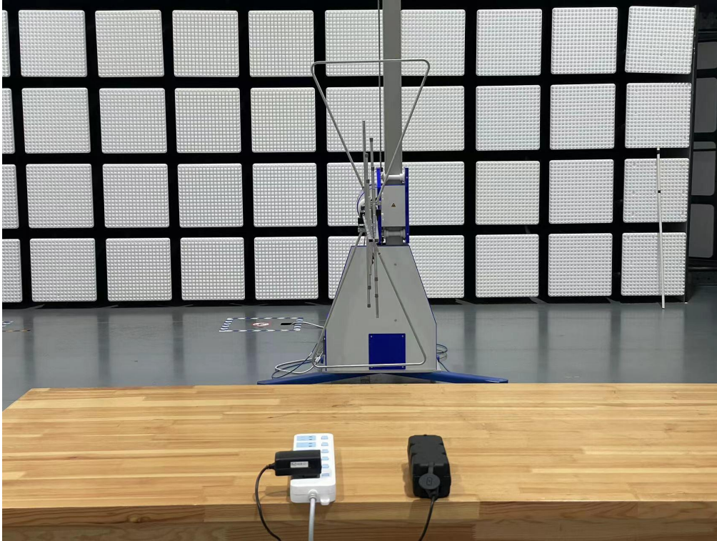
RE 30MHz-1GHz
