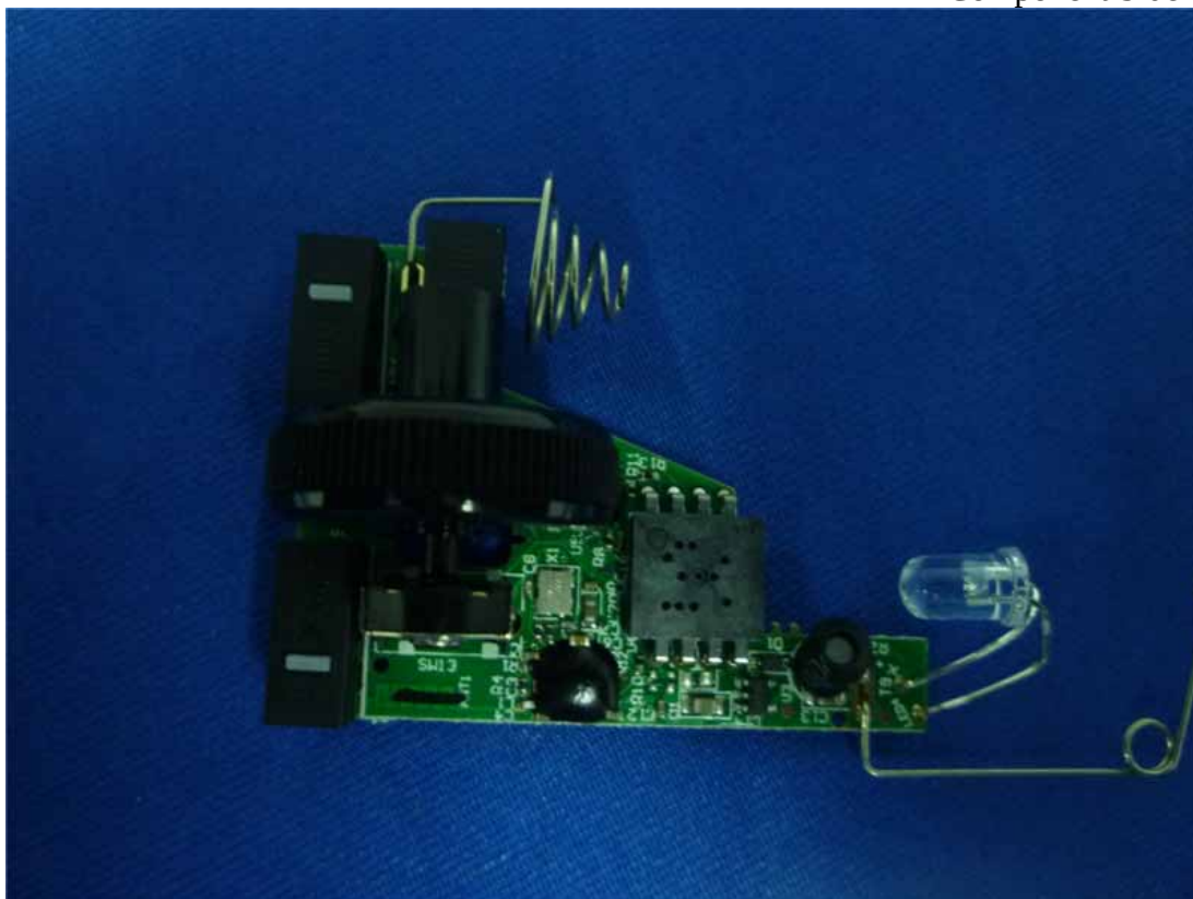
Figure 10 Component Side of the PCB
