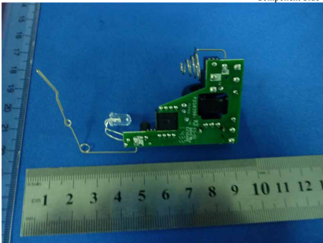
Figure 9 Component Side of the PCB
