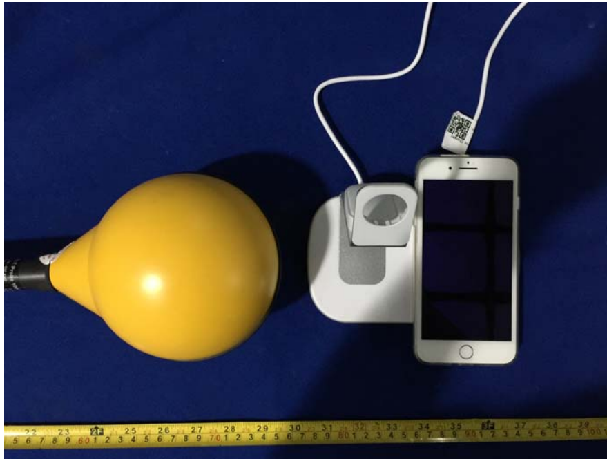
E-Field Strength View
