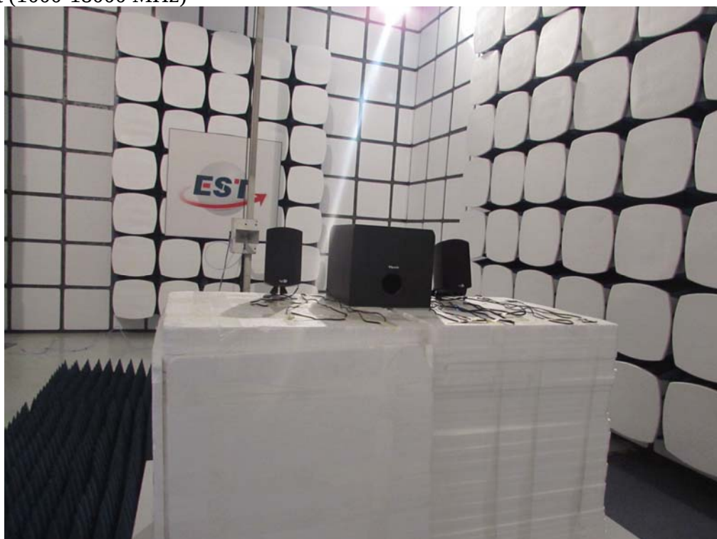
Radiated Test (1000-18000 MHz)
