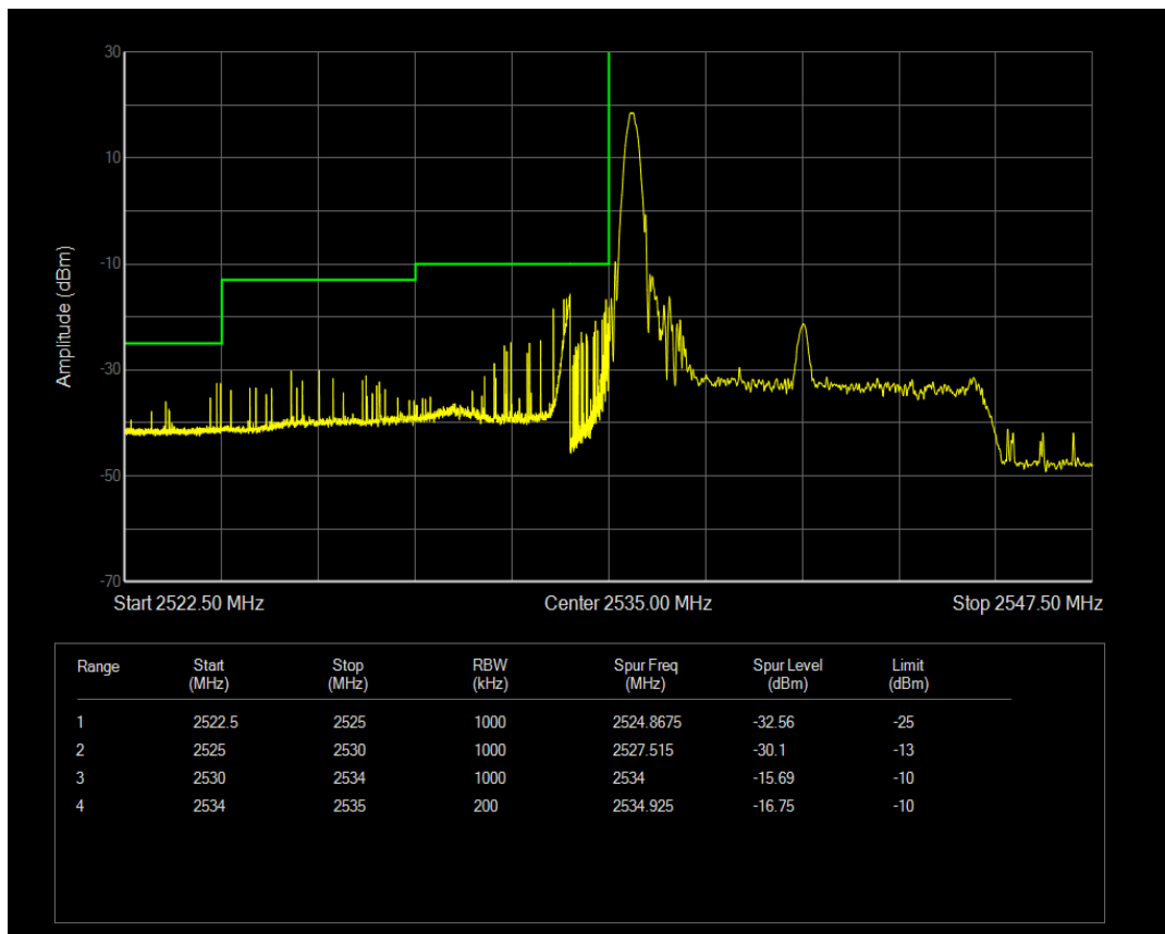
Band41(2535-2655) 16QAM BW=10MHz Channel=40090 RB Size=1 Position=#Max
