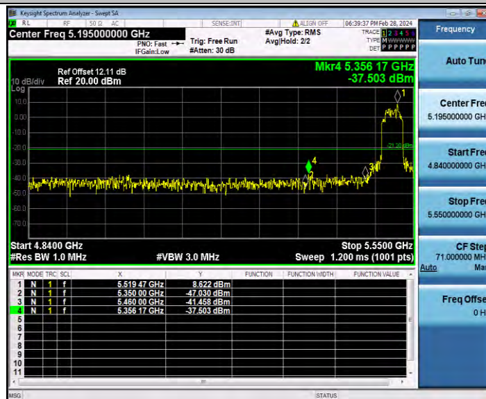
11AX40SISO_Ant1_Low_5510_Peak
