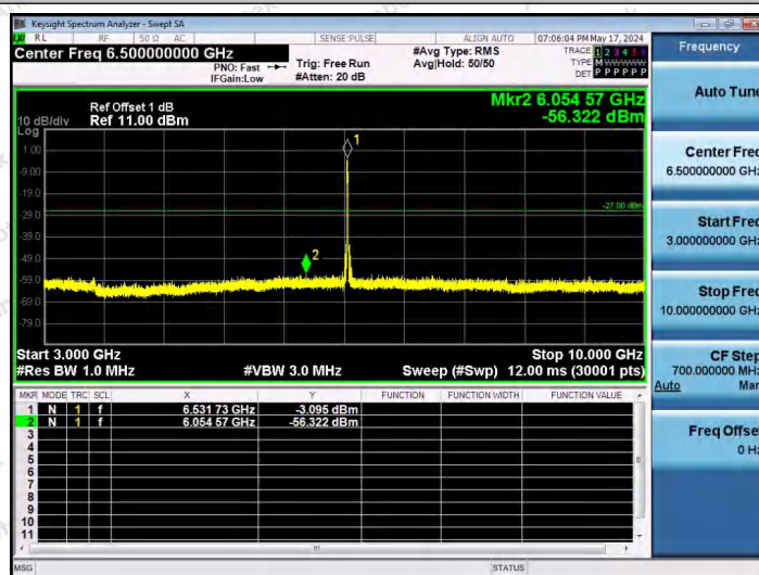
11AX20SISO-Ant1-6535-106Tone-RU53-3000~10000-PASS
