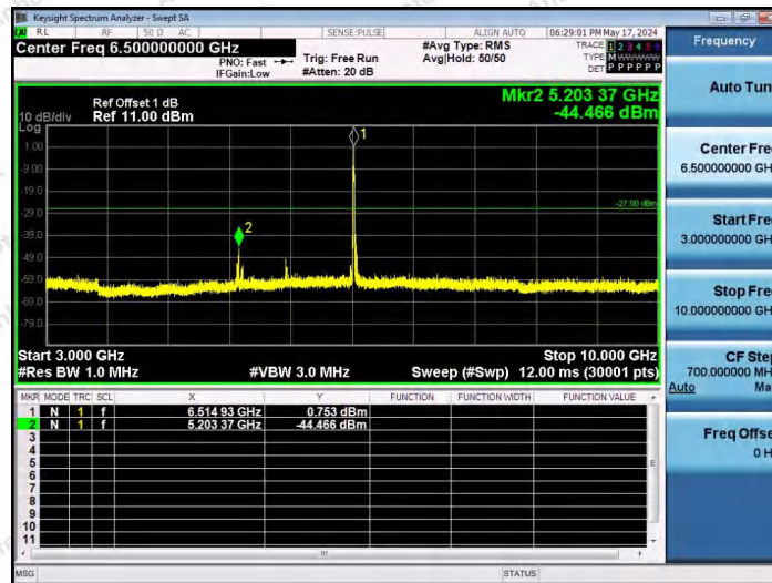
11AX20SISO-Ant1-6515-26Tone-RU4-3000~10000-PASS
