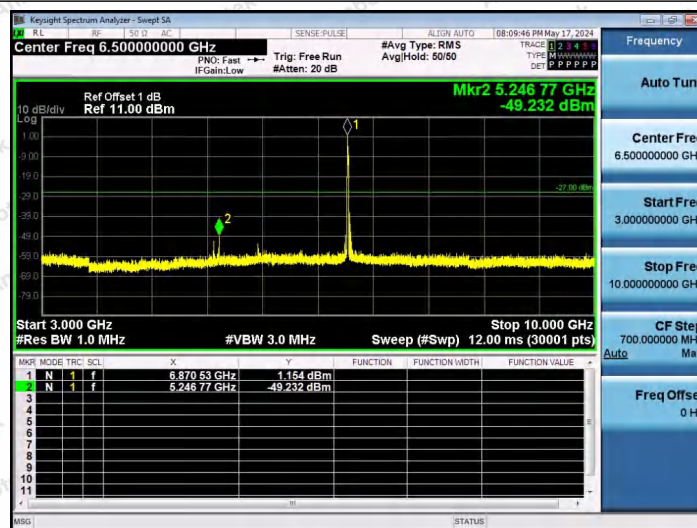
11AX20SISO-Ant1-6875-106Tone-RU53-3000~10000-PASS
