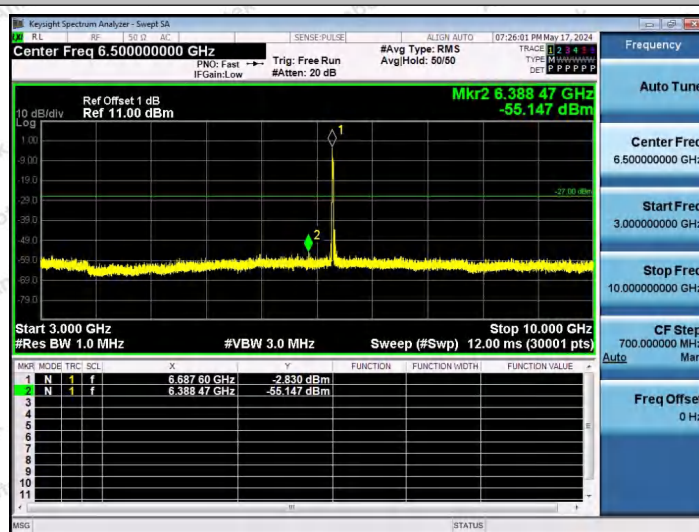
11AX20SISO-Ant1-6695-52Tone-RU37-3000~10000-PASS
