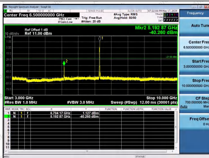
11AX20SISO-Ant1-6695-26Tone-RU8-3000~10000-PASS
