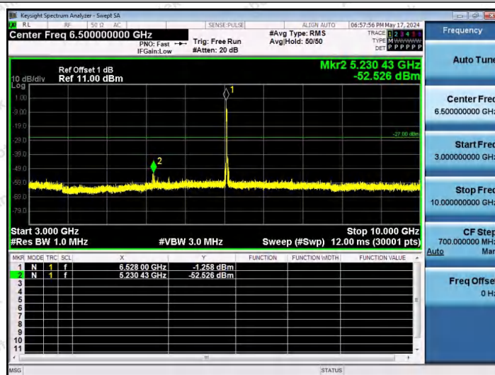
11AX20SISO-Ant1-6535-52Tone-RU37-3000~10000-PASS
