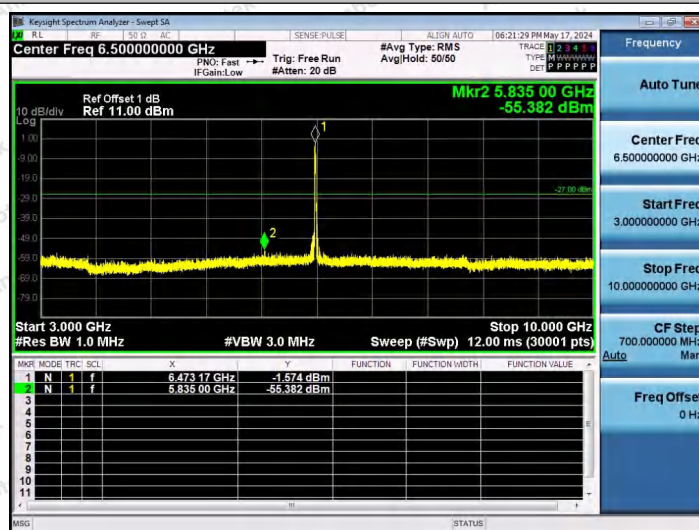
11AX20SISO-Ant1-6475-106Tone-RU53-3000~10000-PASS
