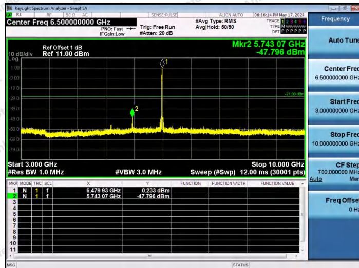
11AX20SISO-Ant1-6475-52Tone-RU39-3000~10000-PASS
