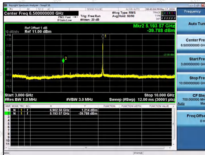
11AX20SISO-Ant1-6895-52Tone-RU40-3000~10000-PASS
