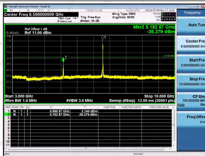
11AX20SISO-Ant1-6895-52Tone-RU37-3000~10000-PASS
