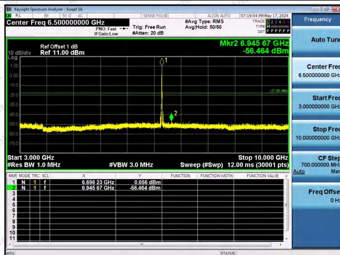
11AX20SISO-Ant1-6695-26Tone-RU4-3000~10000-PASS
