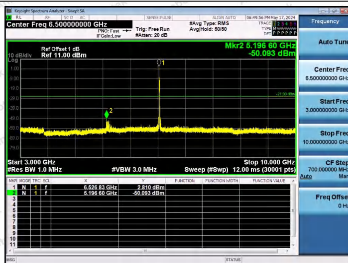
11AX20SISO-Ant1-6535-26Tone-RU0-3000~10000-PASS
