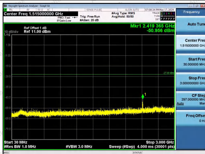
11AX20SISO-Ant1-6535-106Tone-RU54-30~3000-PASS
