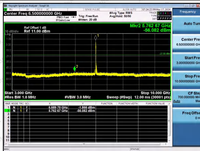
11AX20SISO-Ant1-6695-106Tone-RU53-3000~10000-PASS
