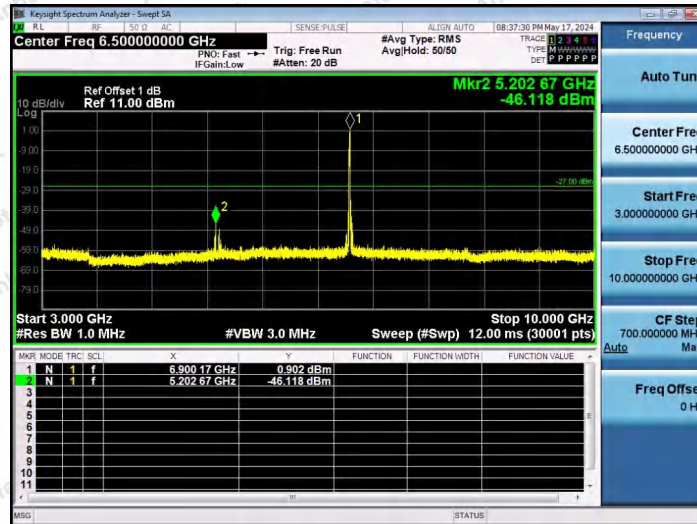
11AX20SISO-Ant1-6895-52Tone-RU39-3000~10000-PASS
