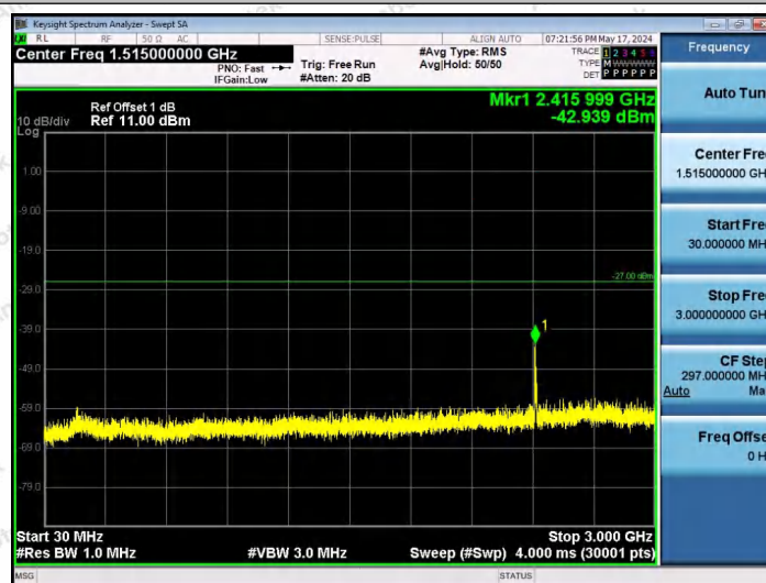
11AX20SISO-Ant1-6695-26Tone-RU8-30~3000-PASS
