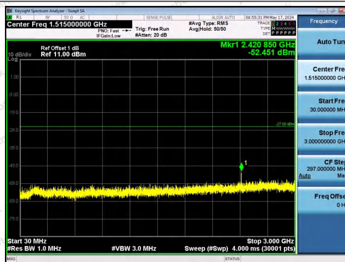
11AX20SISO-Ant1-6535-26Tone-RU8-30~3000-PASS
