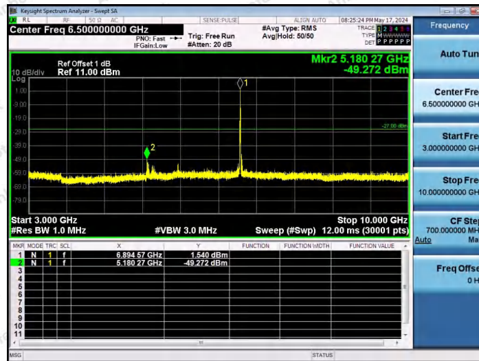
11AX20SISO-Ant1-6895-26Tone-RU4-3000~10000-PASS
