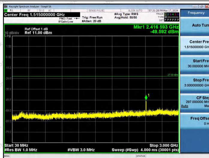
11AX20SISO-Ant1-6695-52Tone-RU40-30~3000-PASS
