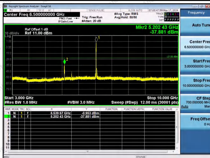
11AX20SISO-Ant1-6535-52Tone-RU39-3000~10000-PASS
