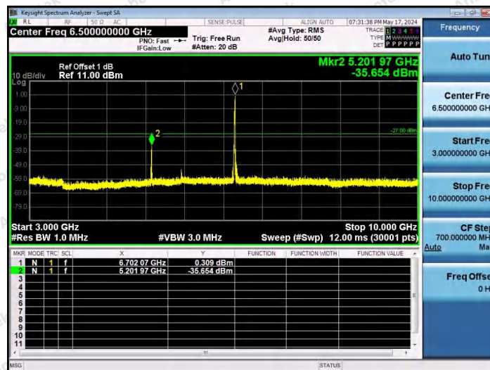
11AX20SISO-Ant1-6695-52Tone-RU40-3000~10000-PASS
