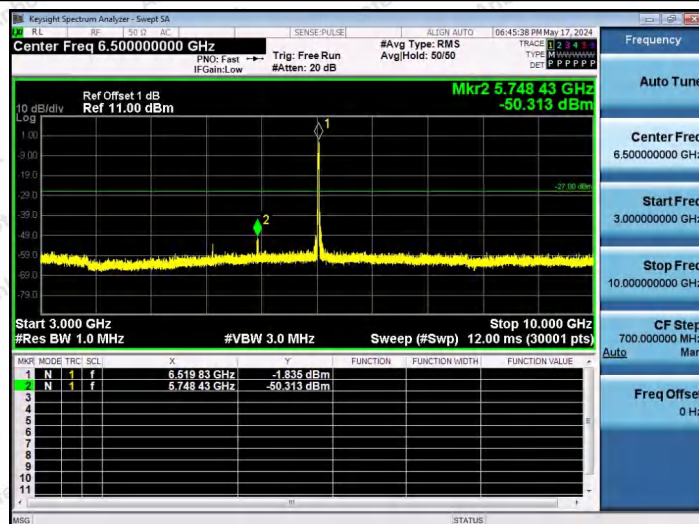
11AX20SISO-Ant1-6515-106Tone-RU54-3000~10000-PASS
