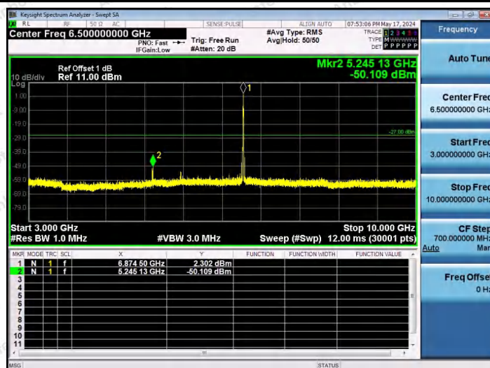
11AX20SISO-Ant1-6875-26Tone-RU4-3000~10000-PASS
