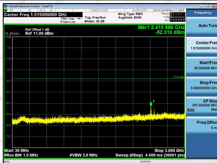
11AX20SISO-Ant1-6515-106Tone-RU54-30~3000-PASS
