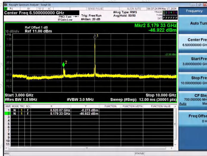
11AX20SISO-Ant1-6515-52Tone-RU39-3000~10000-PASS
