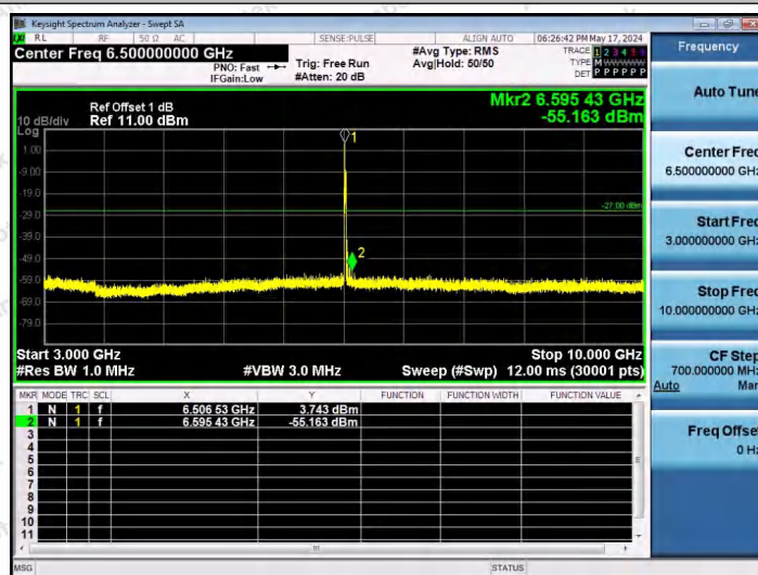
11AX20SISO-Ant1-6515-26Tone-RU0-3000~10000-PASS
