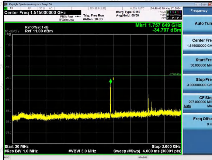
11AX20SISO-Ant1-6535-26Tone-RU0-30~3000-PASS
