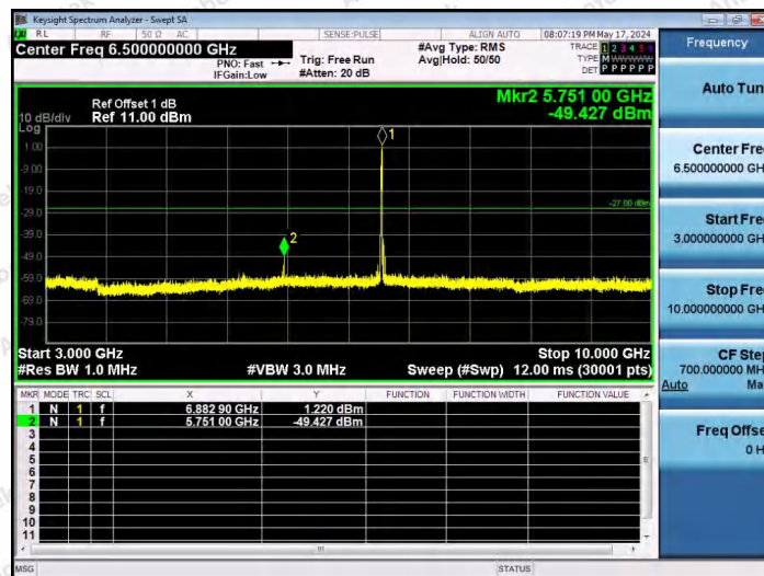
11AX20SISO-Ant1-6875-52Tone-RU40-3000~10000-PASS
