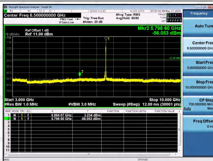
11AX20SISO-Ant1-6875-26Tone-RU8-3000~10000-PASS
