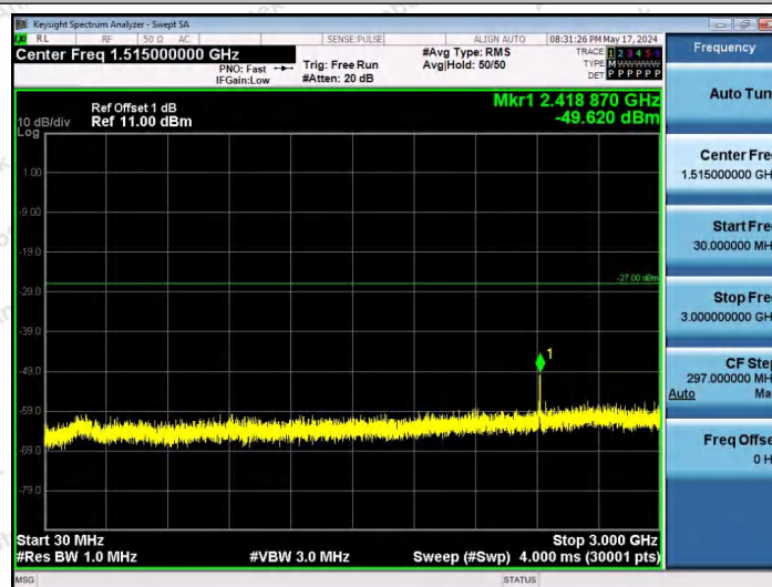
11AX20SISO-Ant1-6895-26Tone-RU8-30~3000-PASS
