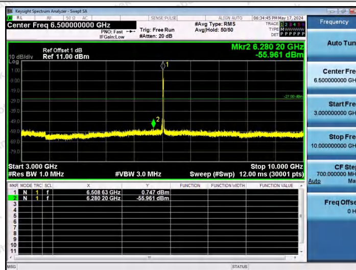
11AX20SISO-Ant1-6515-52Tone-RU37-3000~10000-PASS
