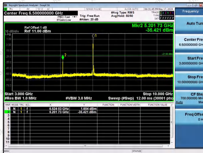
11AX20SISO-Ant1-6515-26Tone-RU8-3000~10000-PASS
