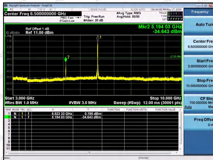
11AX20SISO-Ant1-6515-52Tone-RU40-3000~10000-PASS
