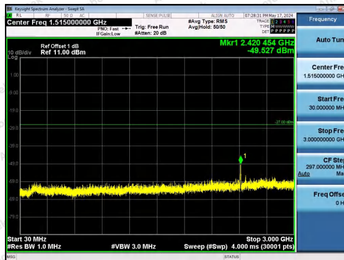
11AX20SISO-Ant1-6695-52Tone-RU39-30~3000-PASS
