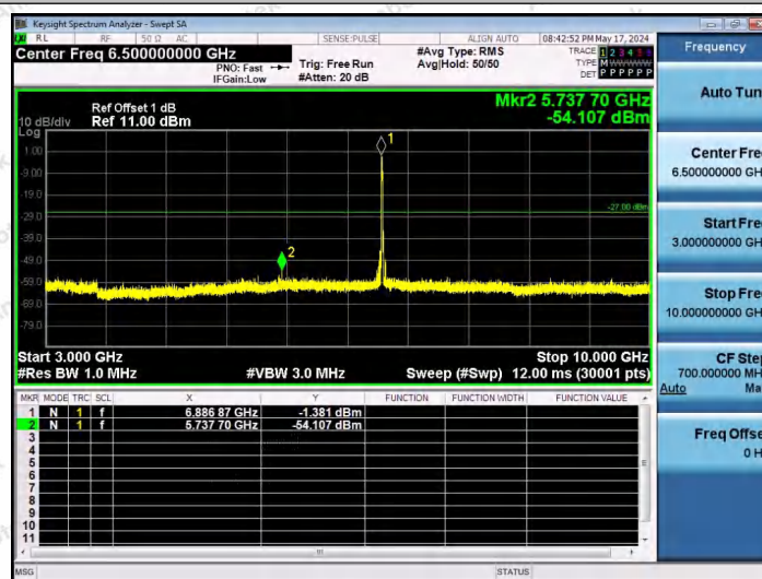
11AX20SISO-Ant1-6895-106Tone-RU53-3000~10000-PASS
