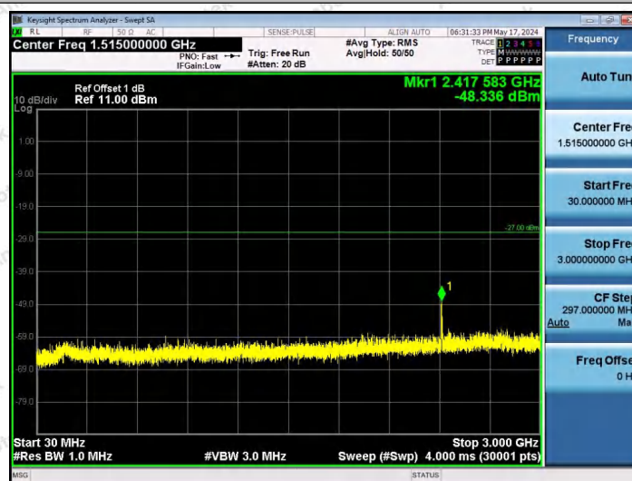
11AX20SISO-Ant1-6515-26Tone-RU8-30~3000-PASS
