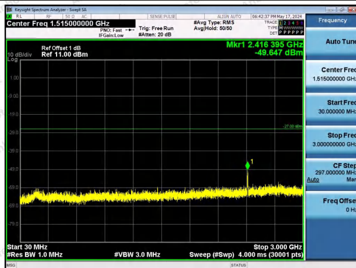
11AX20SISO-Ant1-6515-106Tone-RU53-30~3000-PASS
