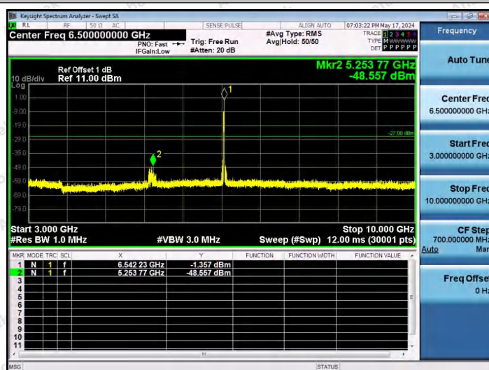
11AX20SISO-Ant1-6535-52Tone-RU40-3000~10000-PASS
