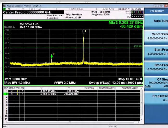
11AX20SISO-Ant1-6875-52Tone-RU37-3000~10000-PASS
