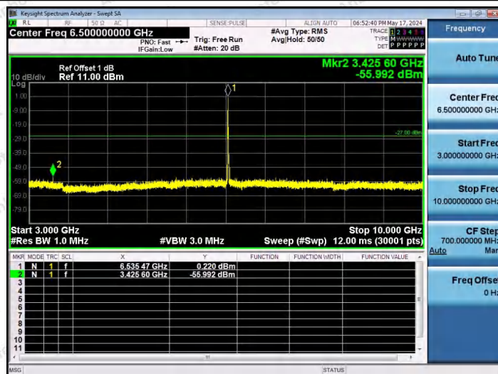
11AX20SISO-Ant1-6535-26Tone-RU4-3000~10000-PASS
