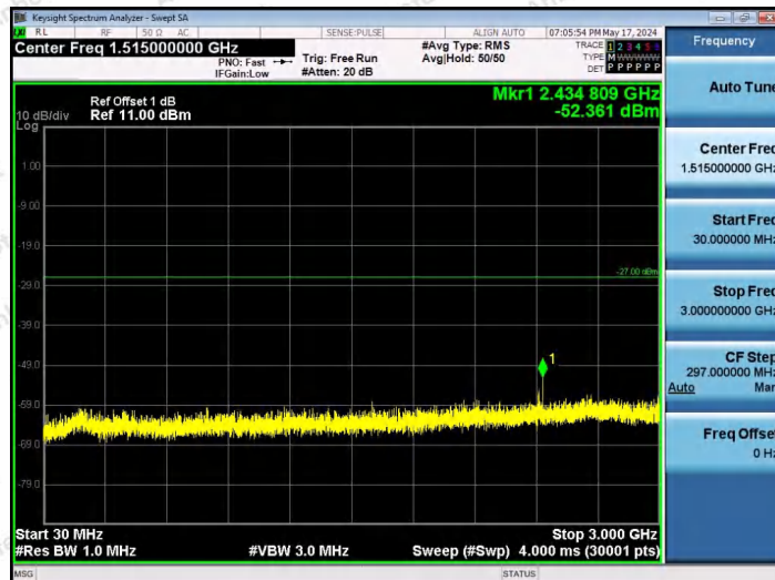
11AX20SISO-Ant1-6535-106Tone-RU53-30~3000-PASS
