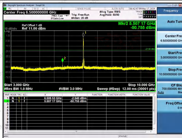
11AX20SISO-Ant1-6515-106Tone-RU53-3000~10000-PASS
