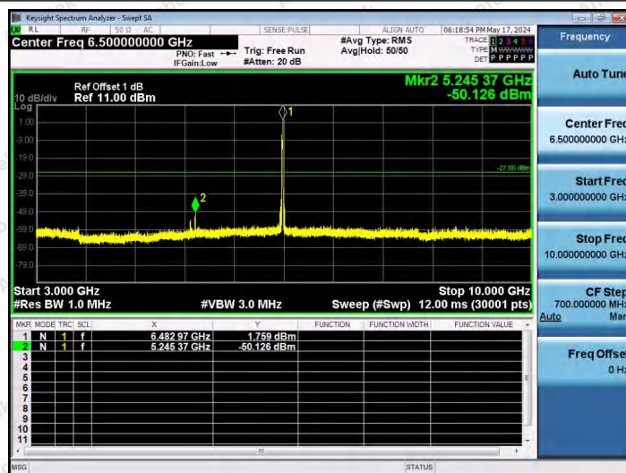
11AX20SISO-Ant1-6475-52Tone-RU40-3000~10000-PASS
