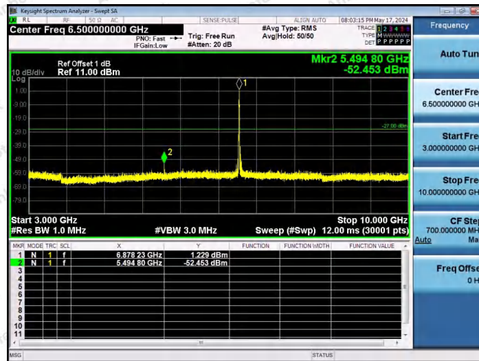
11AX20SISO-Ant1-6875-52Tone-RU39-3000~10000-PASS
