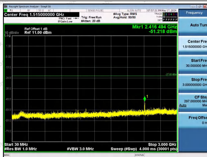
11AX20SISO-Ant1-6875-26Tone-RU8-30~3000-PASS
