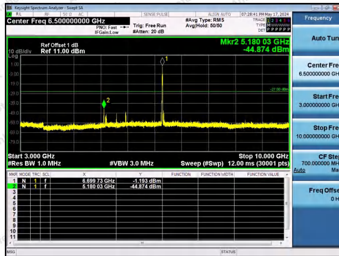
11AX20SISO-Ant1-6695-52Tone-RU39-3000~10000-PASS
