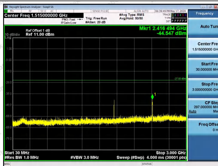
11AX20SISO-Ant1-6515-52Tone-RU40-30~3000-PASS
