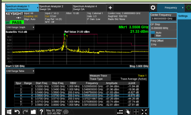
Middle Channel_1RB_Low
