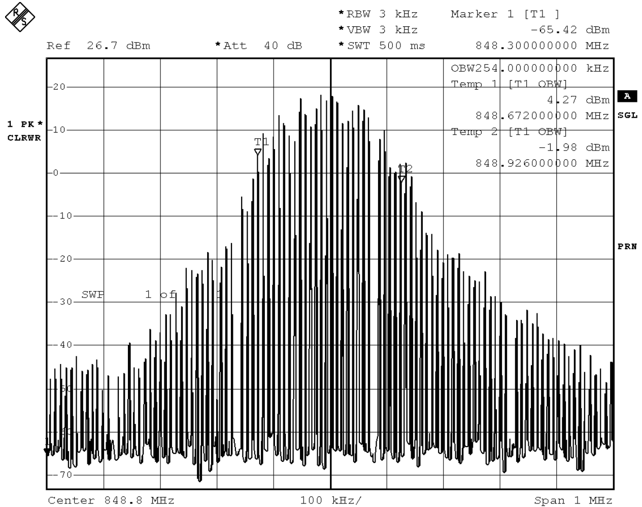
Figure 5-3: Occupied Bandwidth – GSM800 Channel 251
