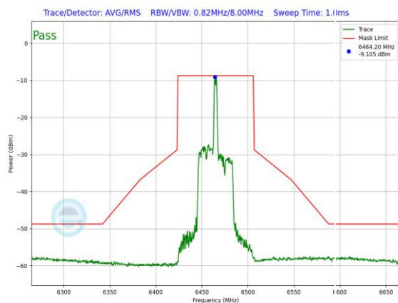
Plot 7-666. LPI In-Band Emission Plot Antenna WF8 (80MHz 802.11ax RU26 (UNII Band 6) – Ch. 103)
