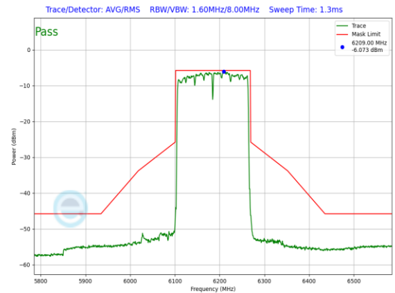
Plot 7-720. LPI In-Band Emission Plot Antenna WF7a (160MHz 802.11ax RU996x2 (UNII Band 5) – Ch. 47)
