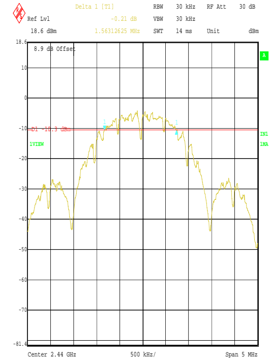
Title: Raymarine. Lifetag Man Overboard Detection System. Comment A: Base Station. Tx Minimum 6 dB Bandwidth (Middel Channel) Date: 11.APR.2006 15:32:22
