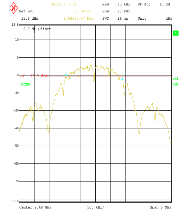
Title: Raymarine. Lifetag Man Overboard Detection System. Comment A: Base Station. Tx Minimum 6 dB Bandwidth (Top Channel) Date: 11.APR.2006 15:30:47
