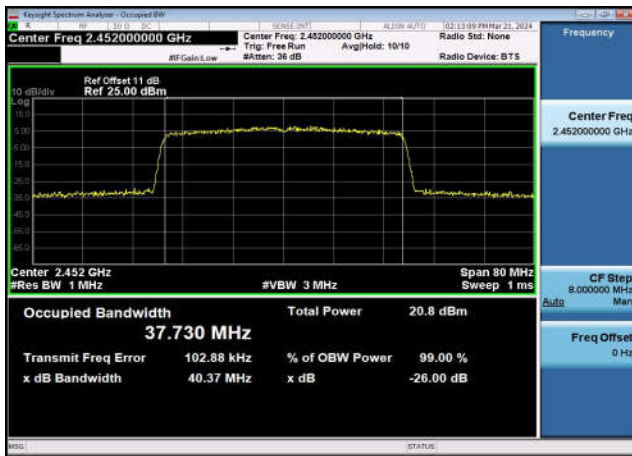
99% Bandwidth-802.11ax(40MHz),2452MHz ,Ant0
