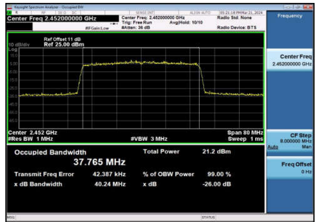
99% Bandwidth-802.11ax(40MHz),2452MHz ,Ant1
