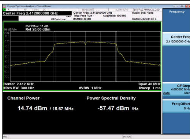
Output Power-802.11g,2437MHz,Ant0
