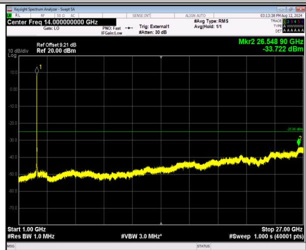
41-41-20MHz-10MHz-QPSK-QPSK-41391-41535-100RB#0 -50RB#0-1000~27000MHz-PASS
