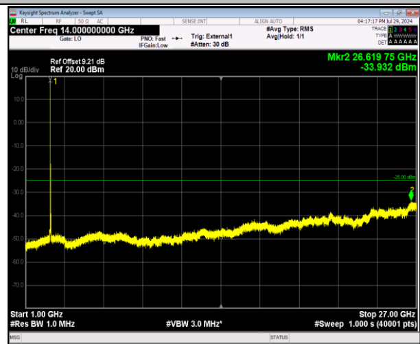
41-41-20MHz-10MHz-64QAM-64QAM-41391-41535-1RB#0 -0RB#0-1000~27000MHz-PASS
