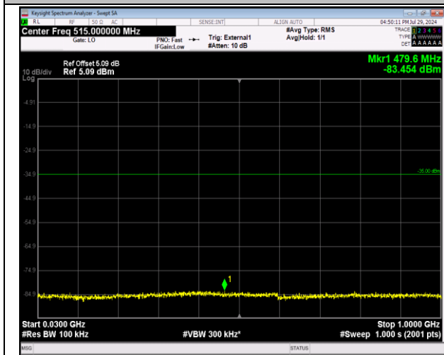
41-41-20MHz-20MHz-64QAM-64QAM-39750-39948-100 RB#0-100RB#0-30~1000MHz-PASS
