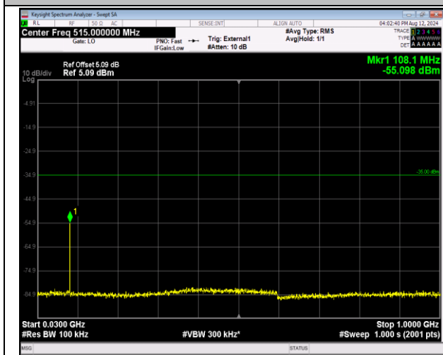
41-41-20MHz-20MHz-QPSK-QPSK-41292-41490-1RB#9 9-0RB#0-30~1000MHz-PASS
