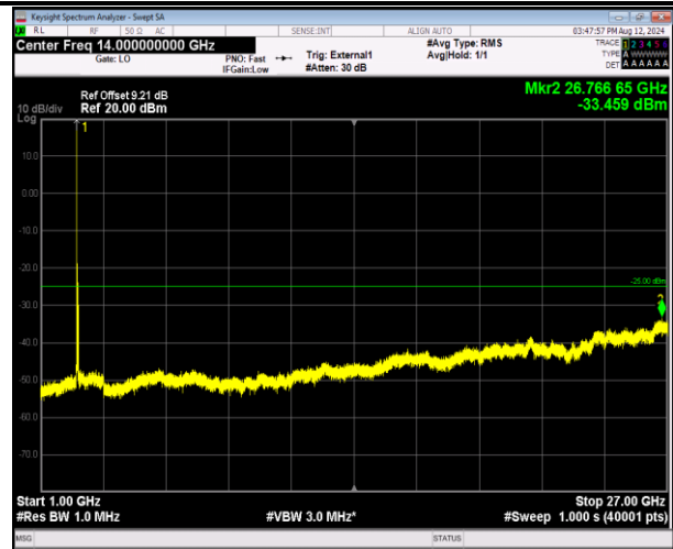
41-41-20MHz-20MHz-16QAM-16QAM-39750-39948-1RB#0 -ORB#0-1000~27000MHz-PASS
