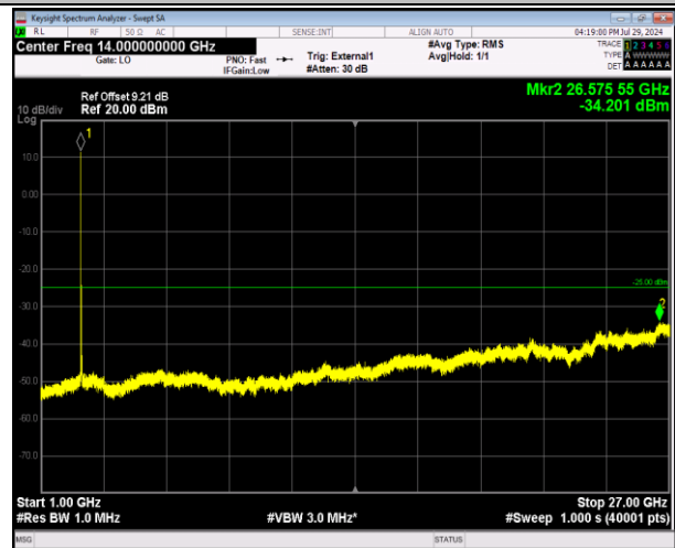
41-41-20MHz-10MHz-64QAM-64QAM-41391-41535-1RB#0 -1RB#49-1000~27000MHz-PASS
