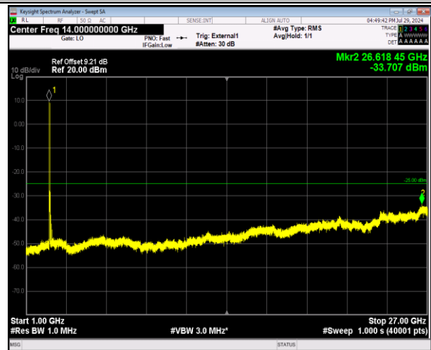
41-41-20MHz-20MHz-64QAM-64QAM-39750-39948-1RB#0 -1RB#99-1000~27000MHz-PASS
