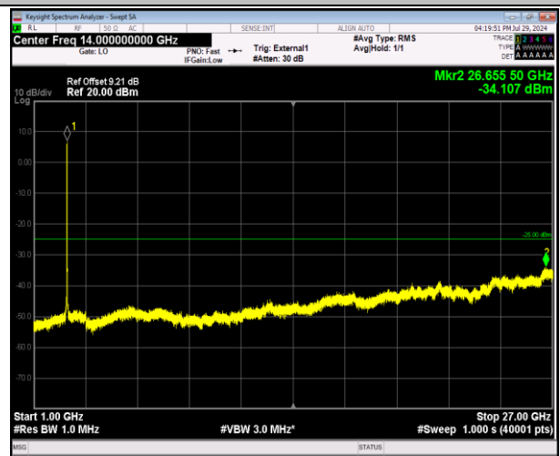
41-41-20MHz-10MHz-64QAM-64QAM-41391-41535-100RB #0-50RB#0-1000~27000MHz-PASS
