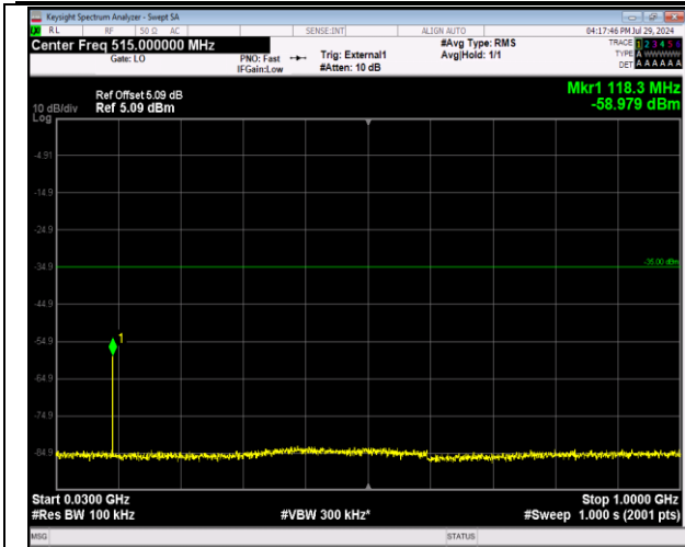
41-41-20MHz-10MHz-64QAM-64QAM-41391-41535-1RB #99-0RB#0-30~1000MHz-PASS
