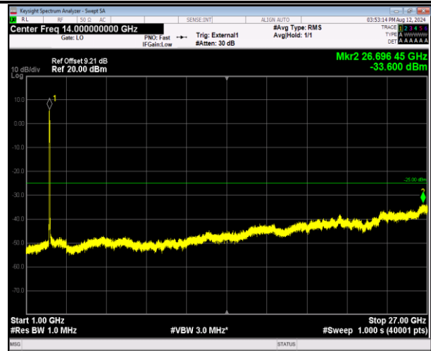
41-41-20MHz-20MHz-16QAM-16QAM-39750-39948-100RB #0-100RB#0-1000~27000MHz-PASS
