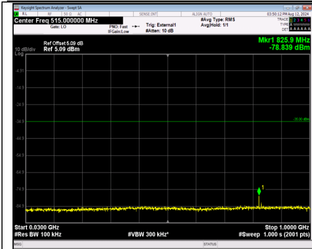
41-41-20MHz-20MHz-QPSK-QPSK-39750-39948-1RB#0 -1RB#99-30~1000MHz-PASS
