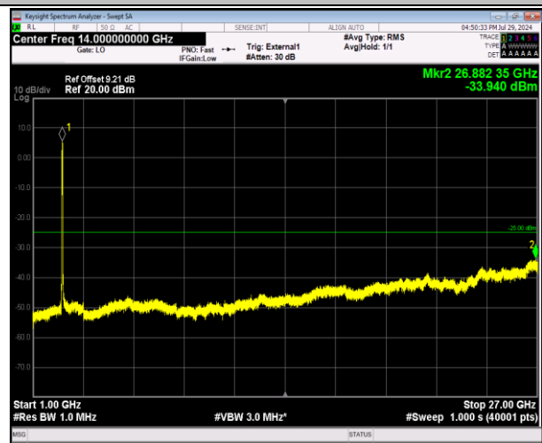
41-41-20MHz-20MHz-64QAM-64QAM-39750-39948-100RB #0-100RB#0-1000~27000MHz-PASS
