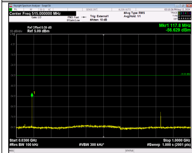
41-41-20MHz-10MHz-16QAM-16QAM-41391-41535-1RB #99-ORB#0-30~1000MHz-PASS
