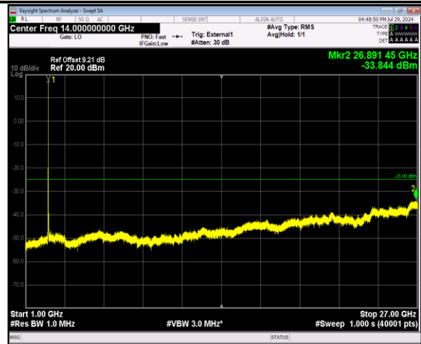
41-41-20MHz-20MHz-64QAM-64QAM-39750-39948-1RB#9 9-0RB#0-1000~27000MHz-PASS
