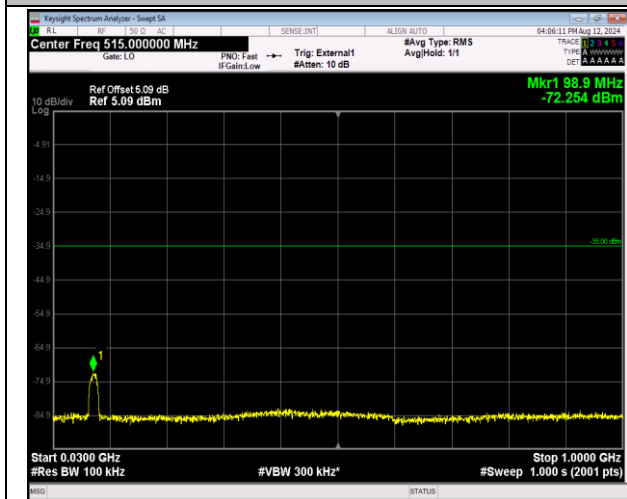
41-41-20MHz-20MHz-QPSK-QPSK-41292-41490-100RB #0-100RB#0-30~1000MHz-PASS
