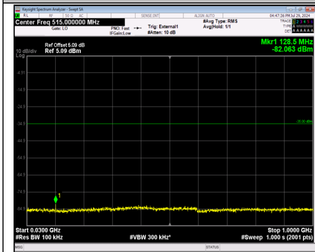
41-41-20MHz-20MHz-64QAM-64QAM-39750-39948-1RB #0-0RB#0-30~1000MHz-PASS
