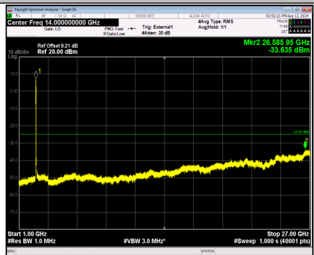
41-41-20MHz-20MHz-QPSK-QPSK-39750-39948-100RB#0 -100RB#0-1000~27000MHz-PASS
