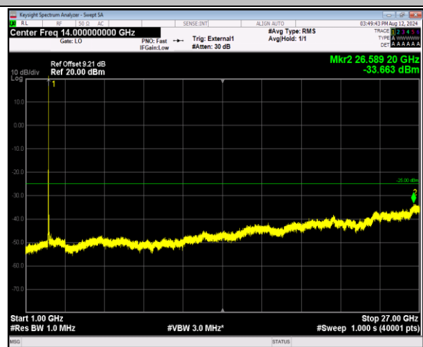
41-41-20MHz-20MHz-16QAM-16QAM-39750-39948-1RB#9 9-ORB#0-1000~27000MHz-PASS
