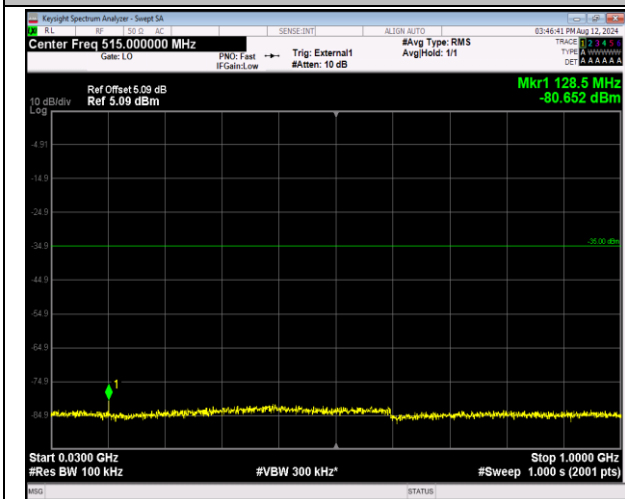
41-41-20MHz-20MHz-QPSK-QPSK-39750-39948-1RB#0 -0RB#0-30~1000MHz-PASS
