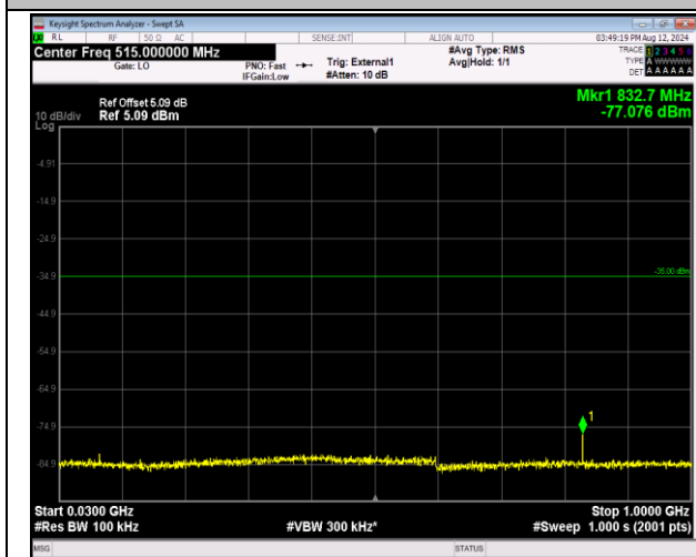
41-41-20MHz-20MHz-16QAM-16QAM-39750-39948-1RB #99-ORB#0-30~1000MHz-PASS
