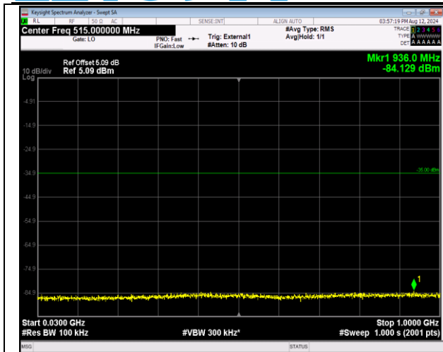
41-41-20MHz-20MHz-QPSK-QPSK-40521-40719-1RB#0 -1RB#99-30~1000MHz-PASS
