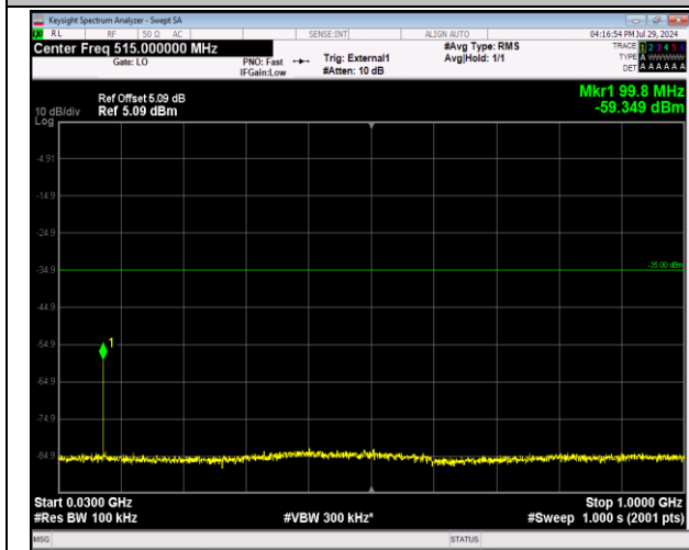
41-41-20MHz-10MHz-64QAM-64QAM-41391-41535-1RB #0-0RB#0-30~1000MHz-PASS
