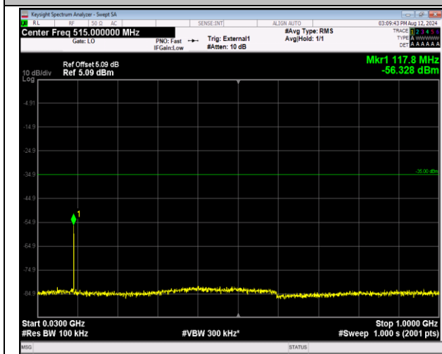
41-41-20MHz-10MHz-QPSK-QPSK-41391-41535-1RB#9 9-0RB#0-30~1000MHz-PASS
