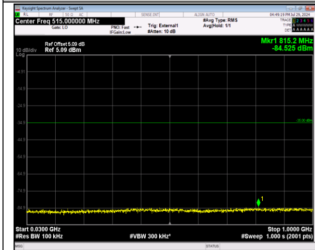
41-41-20MHz-20MHz-64QAM-64QAM-39750-39948-1RB #0-1RB#99-30~1000MHz-PASS
