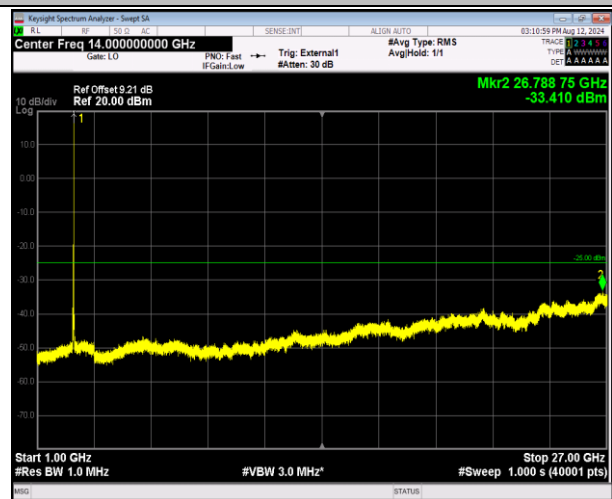
41-41-20MHz-10MHz-16QAM-16QAM-41391-41535-1RB#9 9-ORB#0-1000~27000MHz-PASS
