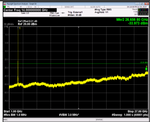
41-41-20MHz-10MHz-64QAM-64QAM-41391-41535-1RB#9 9-0RB#0-1000~27000MHz-PASS
