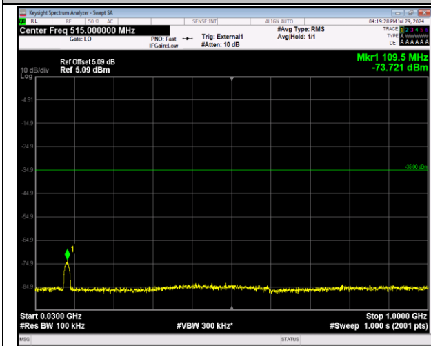
41-41-20MHz-10MHz-64QAM-64QAM-41391-41535-100RB RB#0-50RB#0-30~1000MHz-PASS
