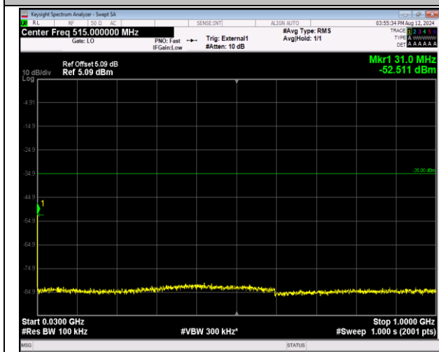
41-41-20MHz-20MHz-QPSK-QPSK-40521-40719-1RB#9 9-0RB#0-30~1000MHz-PASS
