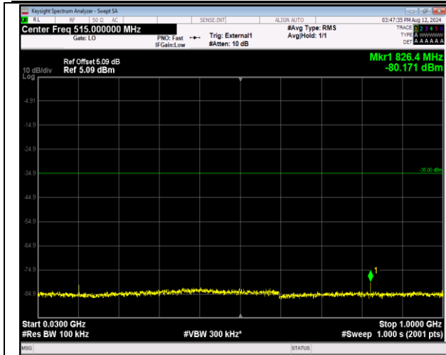
41-41-20MHz-20MHz-16QAM-16QAM-39750-39948-1RB #0-ORB#0-30~1000MHz-PASS
