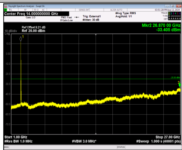
41-41-20MHz-20MHz-16QAM-16QAM-39750-39948-1RB#0 -1RB#99-1000~27000MHz-PASS
