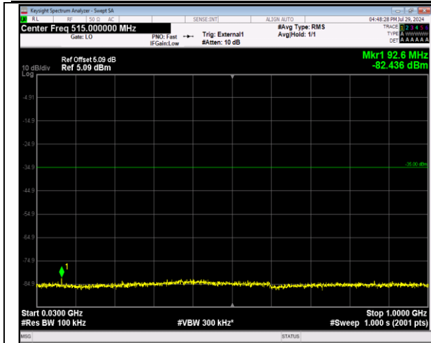
41-41-20MHz-20MHz-64QAM-64QAM-39750-39948-1RB #99-0RB#0-30~1000MHz-PASS
