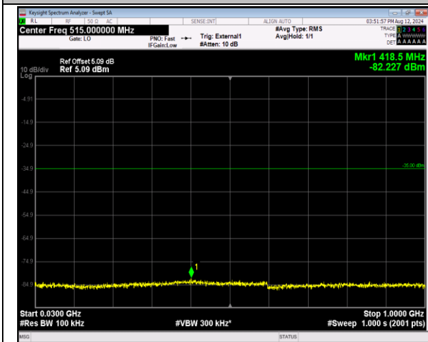
41-41-20MHz-20MHz-QPSK-QPSK-39750-39948-100RB #0-100RB#0-30~1000MHz-PASS
