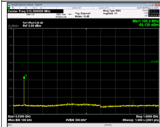
41-41-20MHz-10MHz-QPSK-QPSK-41391-41535-1RB#0 -0RB#0-30~1000MHz-PASS
