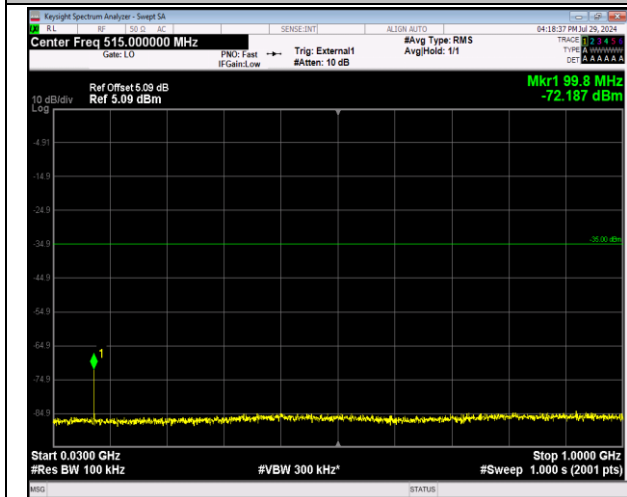
41-41-20MHz-10MHz-64QAM-64QAM-41391-41535-1RB #0-1RB#49-30~1000MHz-PASS
