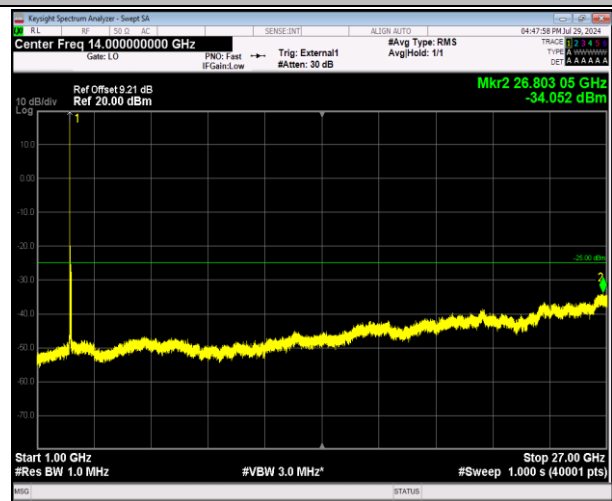
41-41-20MHz-20MHz-64QAM-64QAM-39750-39948-1RB#0 -0RB#0-1000~27000MHz-PASS
