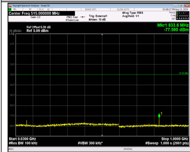
41-41-20MHz-20MHz-QPSK-QPSK-39750-39948-1RB#9 9-0RB#0-30~1000MHz-PASS
