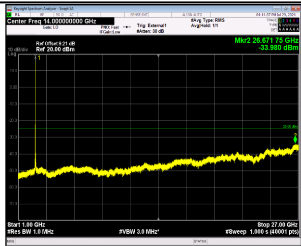
41-41-20MHz-10MHz-64QAM-64QAM-40571-40715-1RB#9 9-0RB#0-1000~27000MHz-PASS
