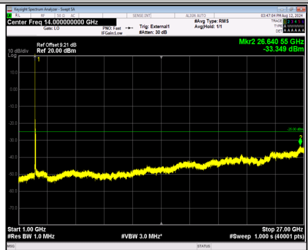
41-41-20MHz-20MHz-QPSK-QPSK-39750-39948-1RB#0-0 RB#0-1000~27000MHz-PASS
