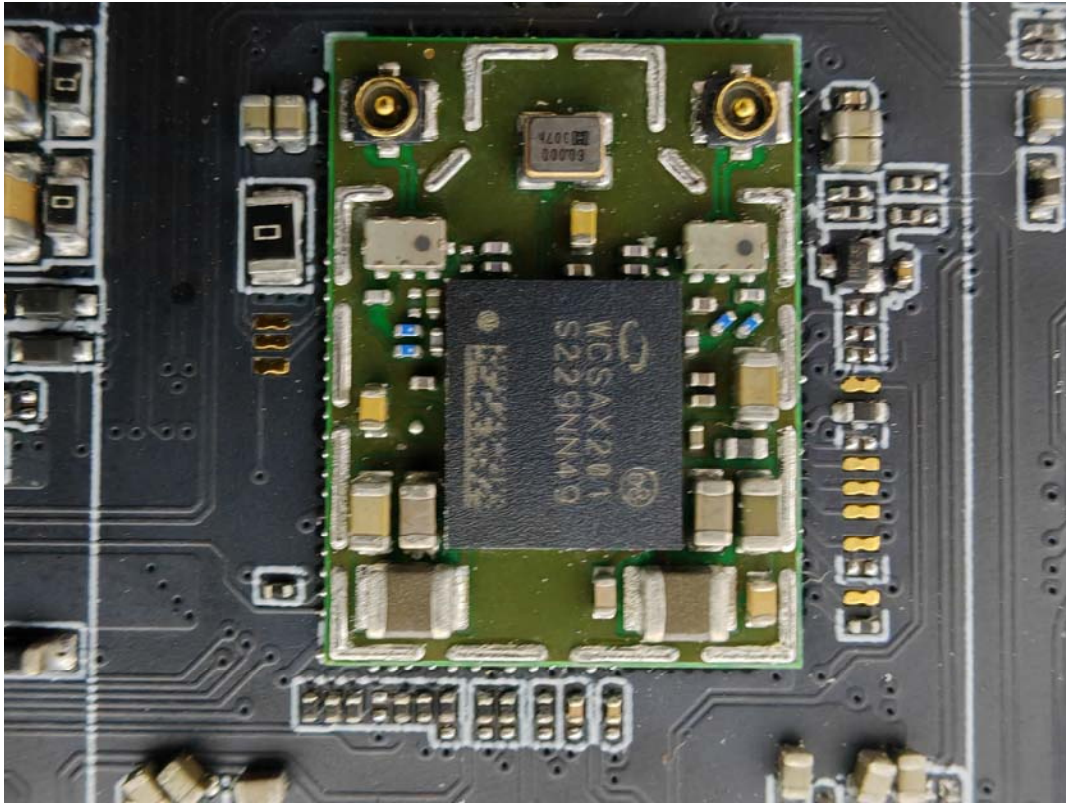
WLAN&BT Module unshielded
