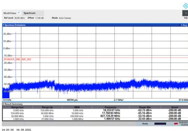
NB-IoT Band 2 CH-High 9kHz~27GHz
