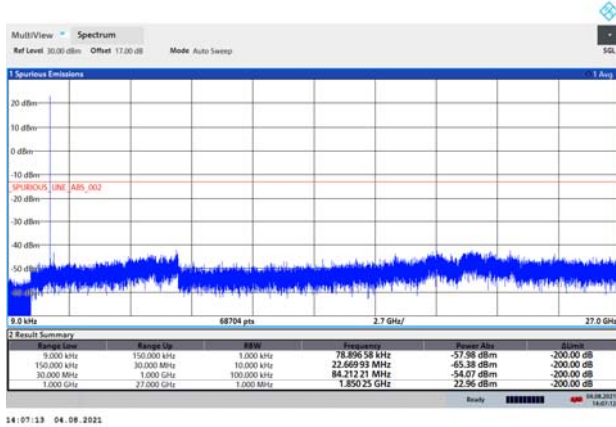
NB-IoT Band 2 CH-Middle 9kHz~27GHz
