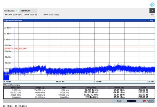
NB-IoT Band 25 CH-High 9kHz~27GHz
