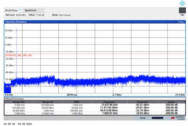
NB-IoT Band 25 CH-Middle 9kHz~27GHz
