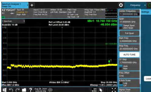
Band66-5MHz-QPSK-132647-1RB#0-3000~20000-PASS
