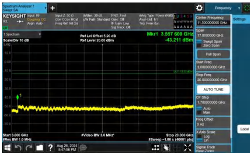
Band66-1.4MHz-QPSK-132665-1RB#0-3000~20000-PASS
