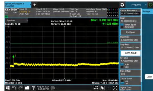
Band66-3MHz-QPSK-132322-1RB#14-3000~20000-PASS
