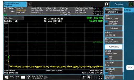
Band66-15MHz-QPSK-132047-1RB#0-0.15~30-PASS
