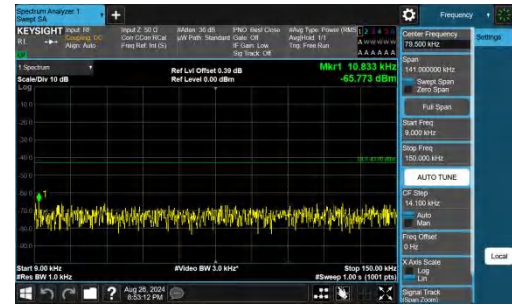
Band66-3MHz-QPSK-131987-1RB#14-0.009~0.15-PASS
