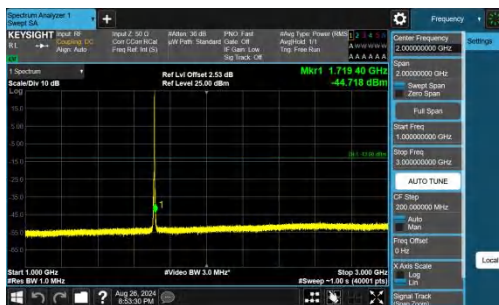
Band66-3MHz-QPSK-131987-1RB#14-1000~3000-PASS
