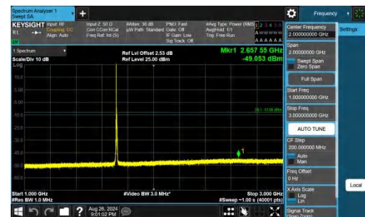
Band66-5MHz-QPSK-131997-1RB#0-1000~3000-PASS
