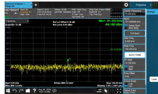
Band66-1.4MHz-QPSK-132665-1RB#5-0.009~0.15-PASS
