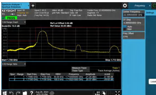
Band66-3MHz-QPSK-131987-1RB#0-PASS
