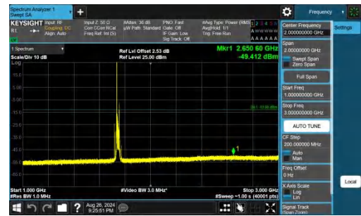
Band66-20MHz-QPSK-132322-1RB#0-1000~3000-PASS
