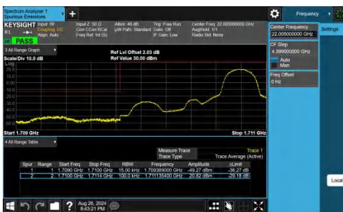
Band66-1.4MHz-QPSK-131979-1RB#5-PASS
