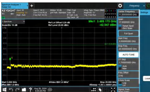
Band66-1.4MHz-QPSK-132322-1RB#0-3000~20000-PASS
