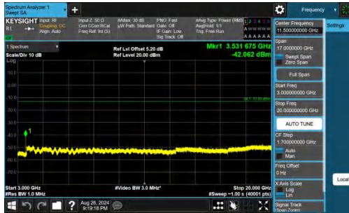
Band66-15MHz-QPSK-132597-1RB#0-3000~20000-PASS
