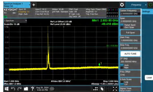
Band66-20MHz-QPSK-132072-1RB#0-1000~3000-PASS
