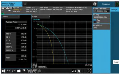
Band66-1.4MHz-QPSK-132322-6RB#0-PASS
