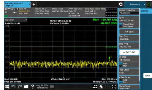
Band66-10MHz-QPSK-132622-1RB#49-0.009~0.15-PASS
