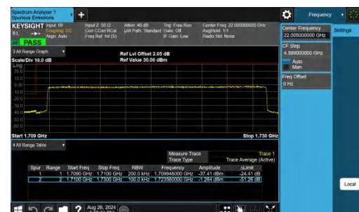
Band66-20MHz-QPSK-132072-100RB#0-PASS
