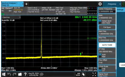
Band66-5MHz-QPSK-132647-1RB#24-1000~3000-PASS
