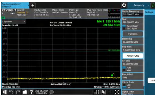
Band66-10MHz-QPSK-132022-1RB#0-30~1000-PASS
