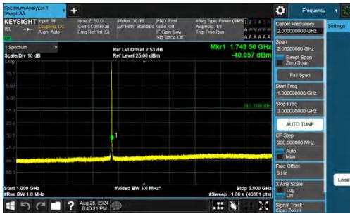
Band66-1.4MHz-QPSK-132322-1RB#5-1000~3000-PASS
