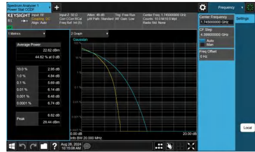
Band66-20MHz-16QAM-132322-27RB#0-PASS
