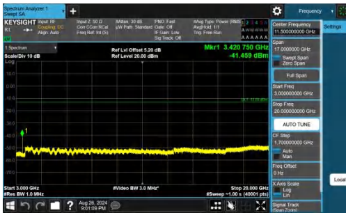
Band66-5MHz-QPSK-131997-1RB#0-3000~20000-PASS
