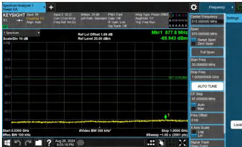
Band66-5MHz-QPSK-132647-1RB#0-30~1000-PASS
