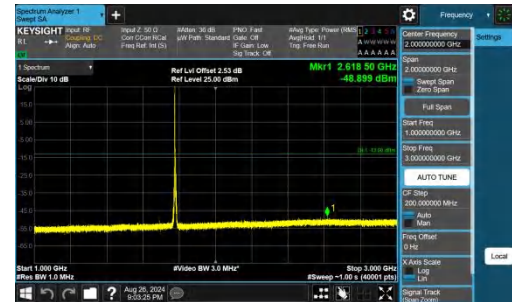
Band66-5MHz-QPSK-132647-1RB#0-1000~3000-PASS
