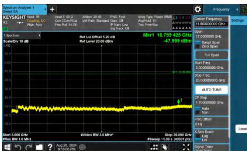
Band66-15MHz-QPSK-132322-1RB#0-3000~20000-PASS
