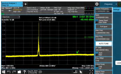
Band66-15MHz-QPSK-132322-1RB#74-1000~3000-PASS
