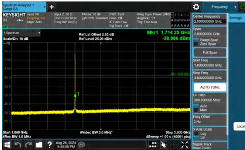
Band66-1.4MHz-QPSK-131979-1RB#5-1000~3000-PASS
