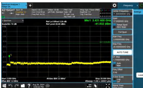
Band66-10MHz-QPSK-132022-1RB#0-3000~20000-PASS
