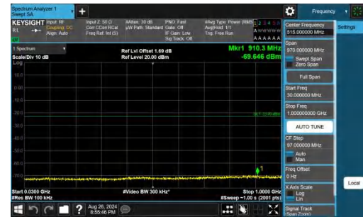
Band66-3MHz-QPSK-132657-1RB#14-30~1000-PASS
