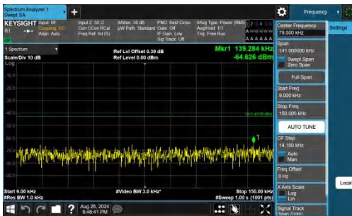
Band66-1.4MHz-QPSK-132665-1RB#0-0.009~0.15-PASS
