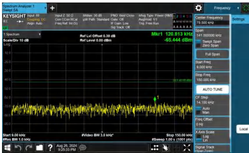
Band66-20MHz-QPSK-132322-1RB#0-0.009~0.15-PASS
