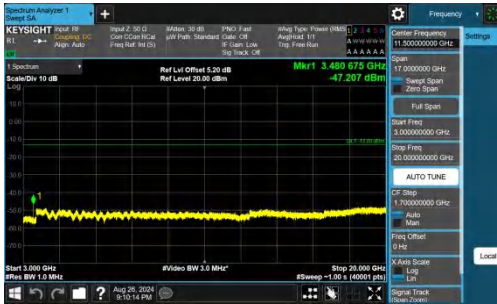
Band66-10MHz-QPSK-132322-1RB#0-3000~20000-PASS
