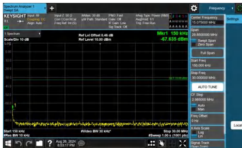
Band66-3MHz-QPSK-131987-1RB#14-0.15~30-PASS
