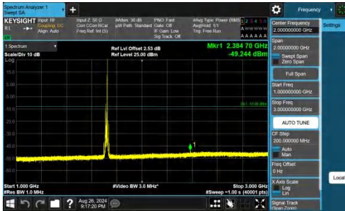
Band66-15MHz-QPSK-132047-1RB#74-1000~3000-PASS
