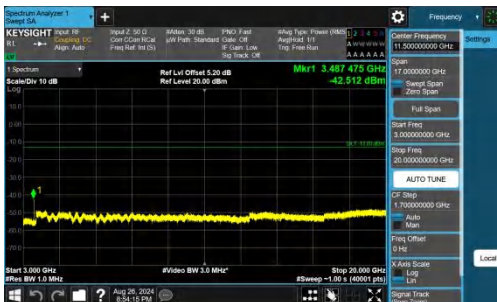
Band66-3MHz-QPSK-132322-1RB#0-3000~20000-PASS
