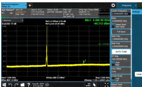
Band66-10MHz-QPSK-132622-1RB#49-1000~3000-PASS
