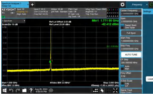
Band66-3MHz-QPSK-132657-1RB#14-1000~3000-PASS
