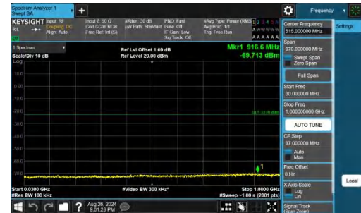
Band66-5MHz-QPSK-131997-1RB#24-30~1000-PASS
