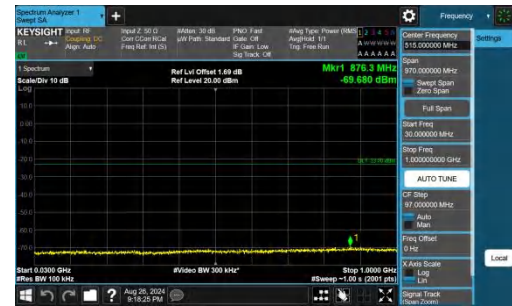
Band66-15MHz-QPSK-132322-1RB#74-30~1000-PASS
