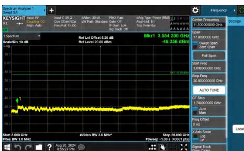
Band66-3MHz-QPSK-132657-1RB#0-3000~20000-PASS
