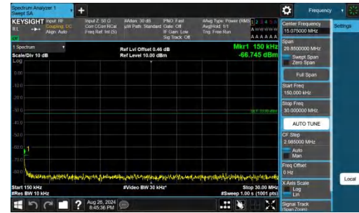
Band66-1.4MHz-QPSK-132322-1RB#0-0.15~30-PASS
