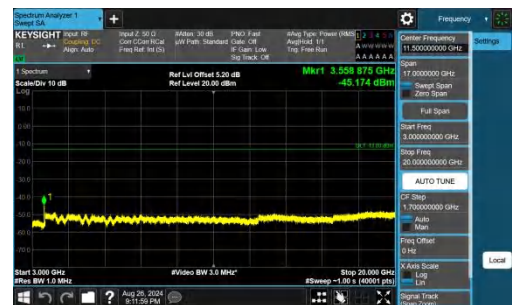
Band66-10MHz-QPSK-132622-1RB#49-3000~20000-PASS
