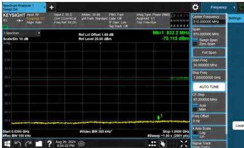
Band66-3MHz-QPSK-132322-1RB#0-30~1000-PASS
