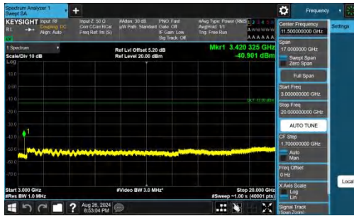
Band66-3MHz-QPSK-131987-1RB#0-3000~20000-PASS
