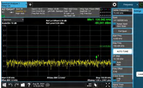
Band66-15MHz-QPSK-132047-1RB#0-0.009~0.15-PASS
