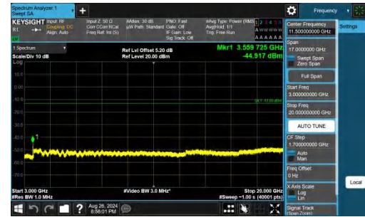
Band66-3MHz-QPSK-132657-1RB#14-3000~20000-PASS
