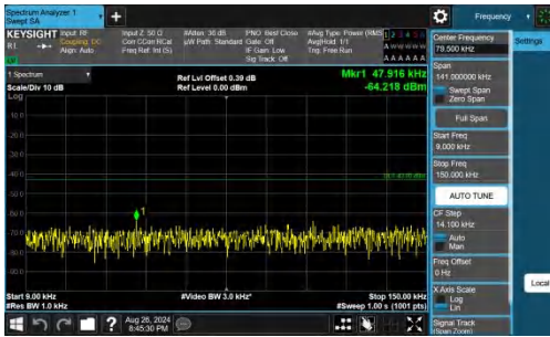
Band66-1.4MHz-QPSK-132322-1RB#0-0.009~0.15-PASS
