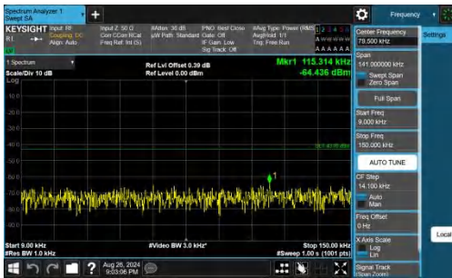
Band66-5MHz-QPSK-132647-1RB#0-0.009~0.15-PASS
