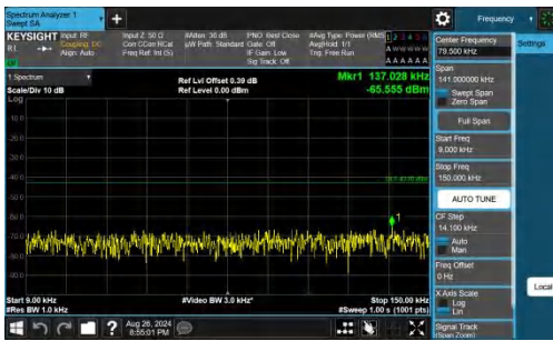
Band66-3MHz-QPSK-132657-1RB#0-0.009~0.15-PASS
