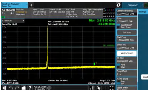
Band66-10MHz-QPSK-132322-1RB#49-1000~3000-PASS
