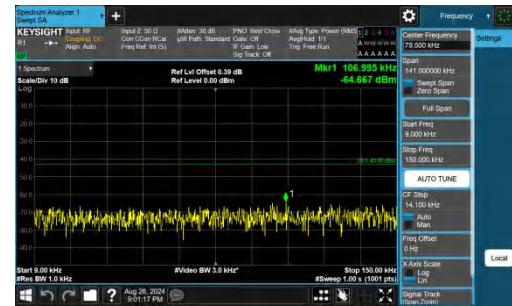
Band66-5MHz-QPSK-131997-1RB#24-0.009~0.15-PASS
