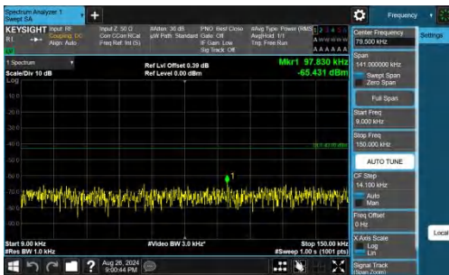
Band66-5MHz-QPSK-131997-1RB#0-0.009~0.15-PASS
