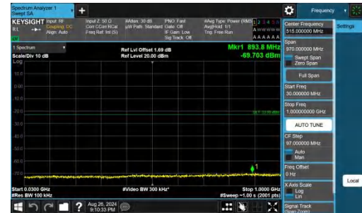
Band66-10MHz-QPSK-132322-1RB#49-30~1000-PASS
