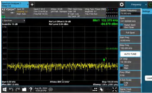
Band66-10MHz-QPSK-132022-1RB#0-0.009~0.15-PASS
