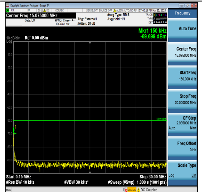
Band48-20MHz-QPSK-56640-1RB#0-0.15~30-PASS
