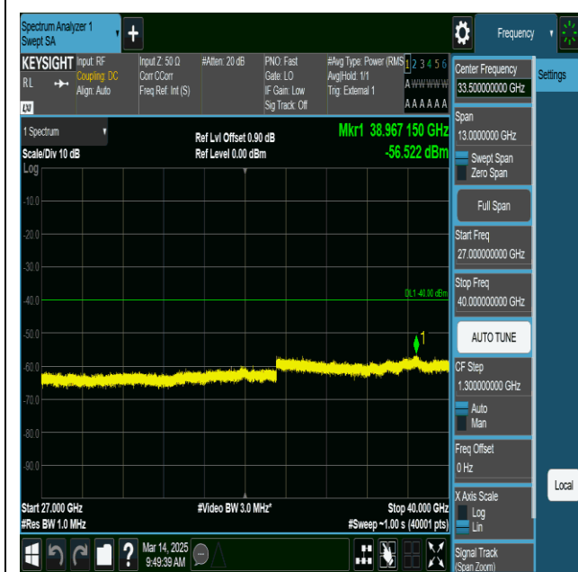
Band48-20MHz-QPSK-56640-1RB#0-27000~40000-PASS
