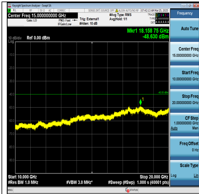
Band48-20MHz-QPSK-56640-1RB#0-10000~20000-PASS
