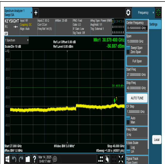
Band48-20MHz-QPSK-55990-1RB#0-27000~40000-PASS
