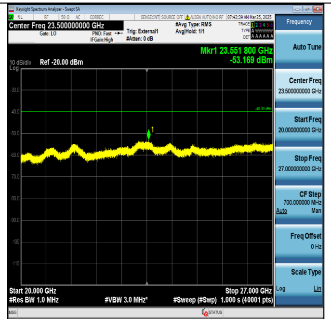
Band48-20MHz-QPSK-56640-1RB#0-20000~27000-PASS
