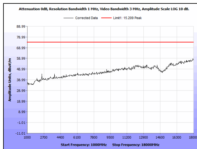
Plot 16. Radiated Spurious Emissions, High Channel, 1 GHz – 18 GHz, Peak
