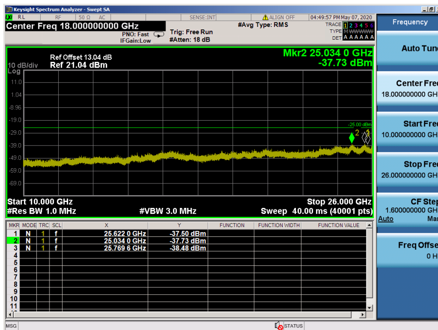
LTE Band 7 / 15 MHz / 64QAM - RB Size/Offset (75/0) – High Channel
