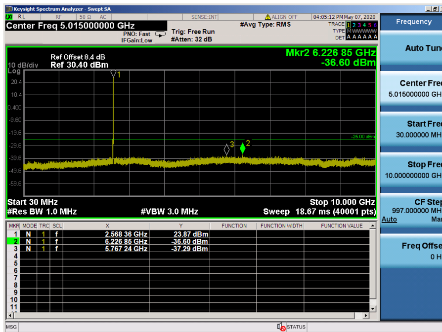
LTE Band 7 / 10 MHz / 64QAM - RB Size/Offset (25/25) – High Channel
