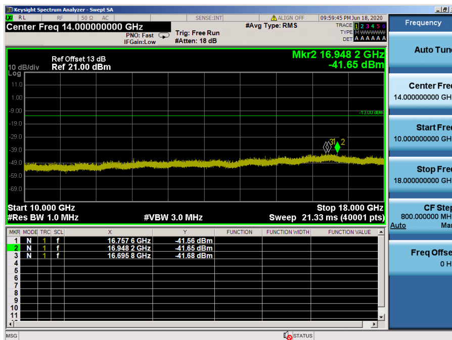
LTE Band 66, 4 / 3MHz / 16QAM - RB Size/Offset (15/0) – High Channel
