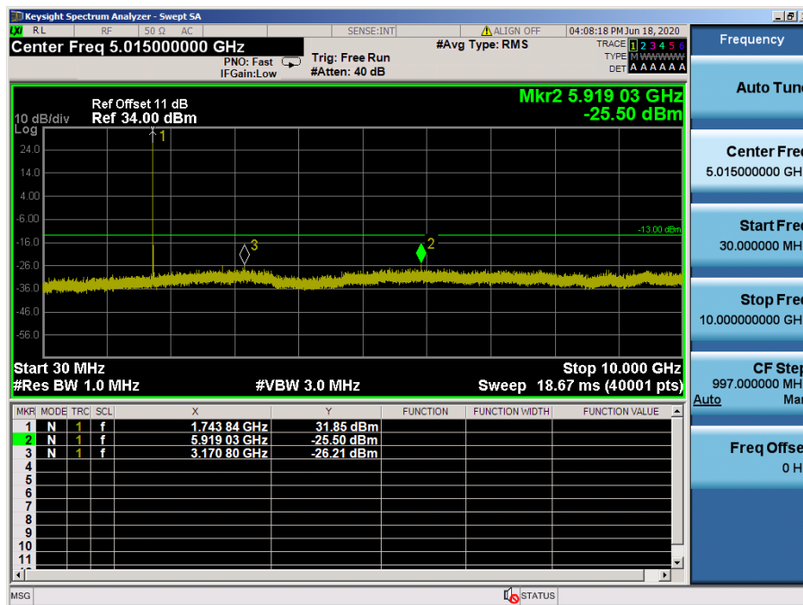
LTE Band 66, 4 / 3MHz / QPSK - RB Size/Offset (1/0) – Mid Channel
