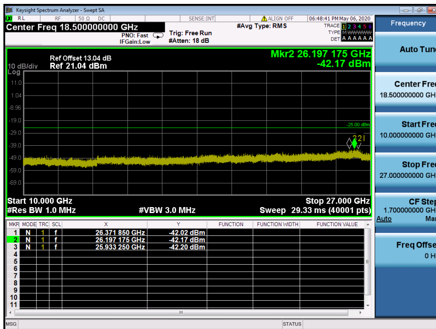
LTE Band 41 / 10 MHz / 16QAM - RB Size/Offset (50/0) – Low Channel
