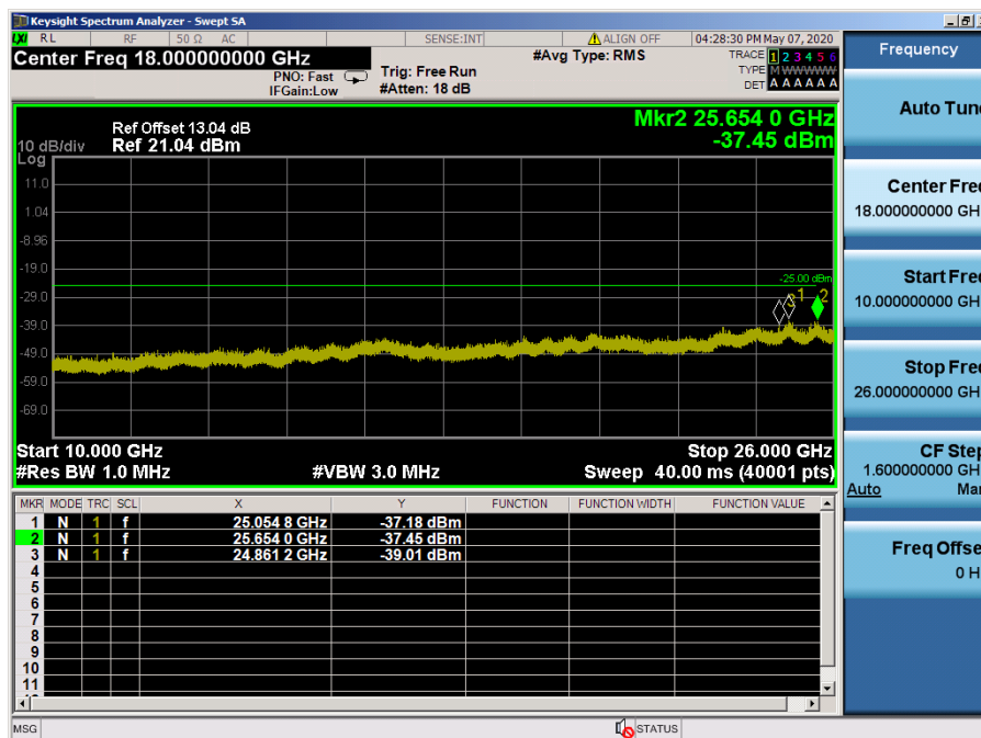
LTE Band 7 / 15 MHz / 64QAM - RB Size/Offset (1/74) – Mid Channel
