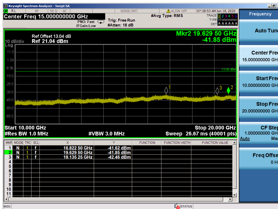
LTE Band 2 / 10 MHz / 64QAM - RB Size/Offset (1/25) – Low Channel
