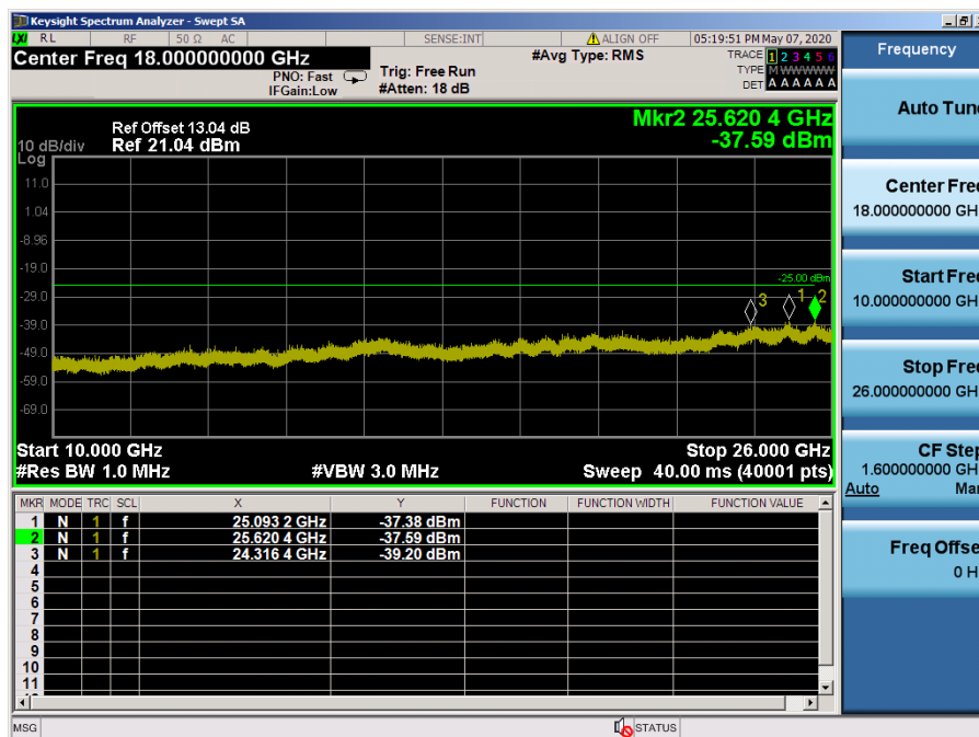
LTE Band 7 / 20 MHz / 64QAM - RB Size/Offset (100/0) – Mid Channel
