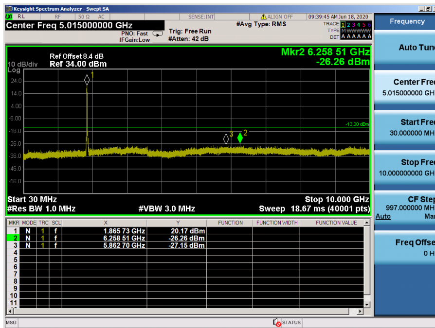
LTE Band 2 / 20 MHz / 64QAM - RB Size/Offset (100/0) – Low Channel
