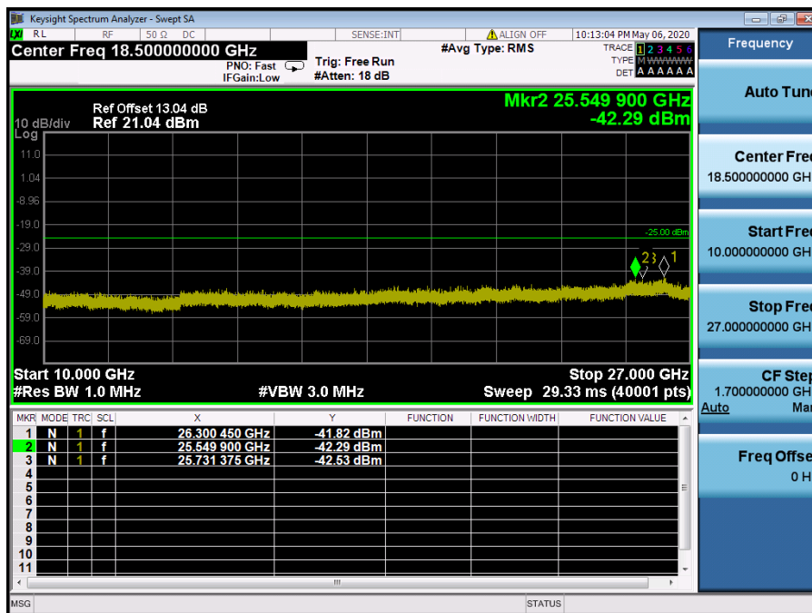
LTE Band 41 / 5 MHz / 64QAM - RB Size/Offset (12/6) – High Channel
