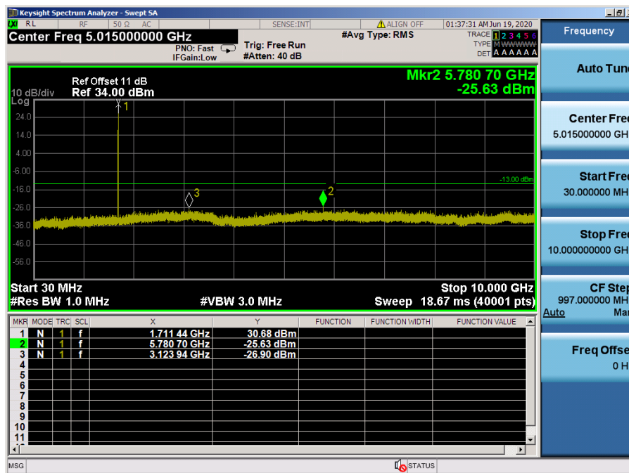
LTE Band 66, 4 / 1.4 MHz / 64QAM - RB Size/Offset (1/5) – Low Channel
