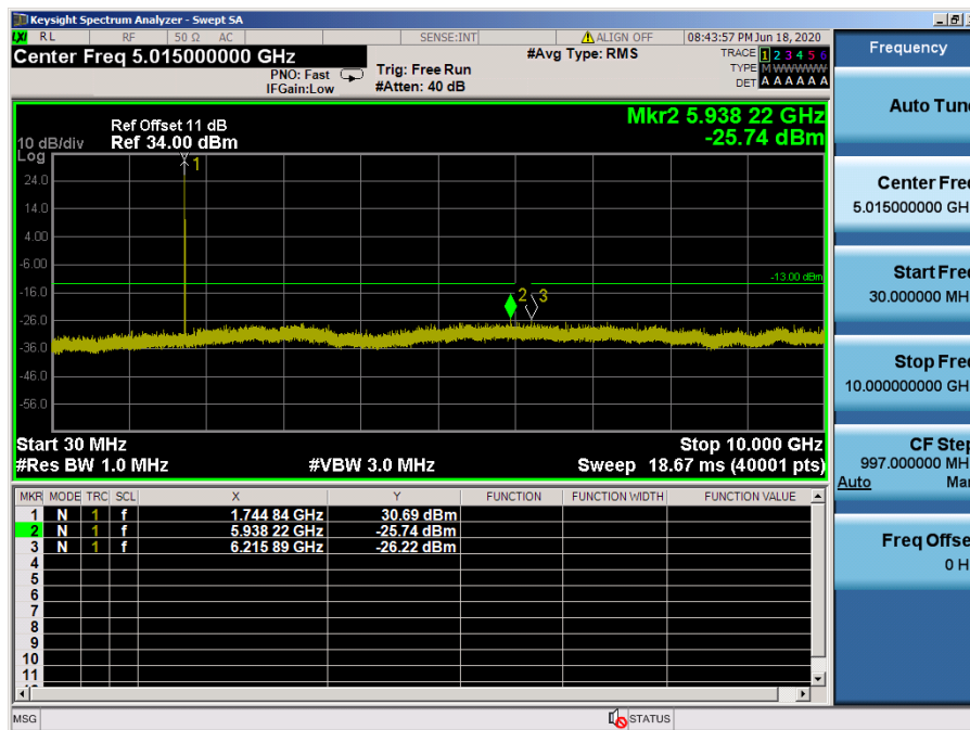
LTE Band 66, 4 / 1.4 MHz / 16QAM - RB Size/Offset (6/0) – Mid Channel
