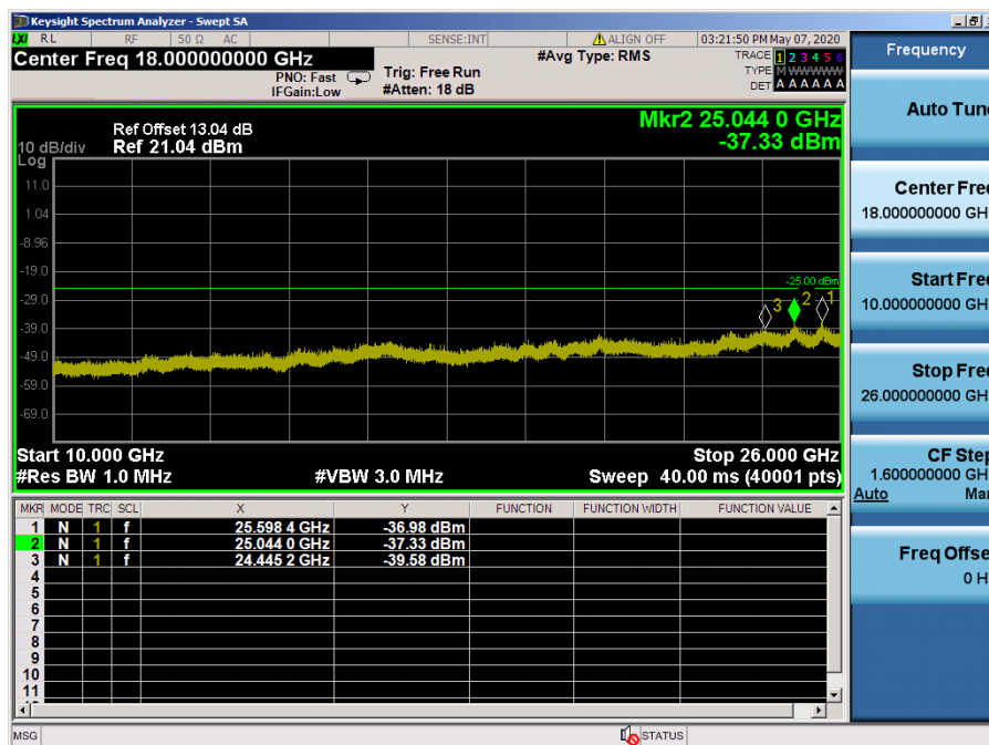
LTE Band 7 / 5 MHz / 64QAM - RB Size/Offset (12/0) – High Channel
