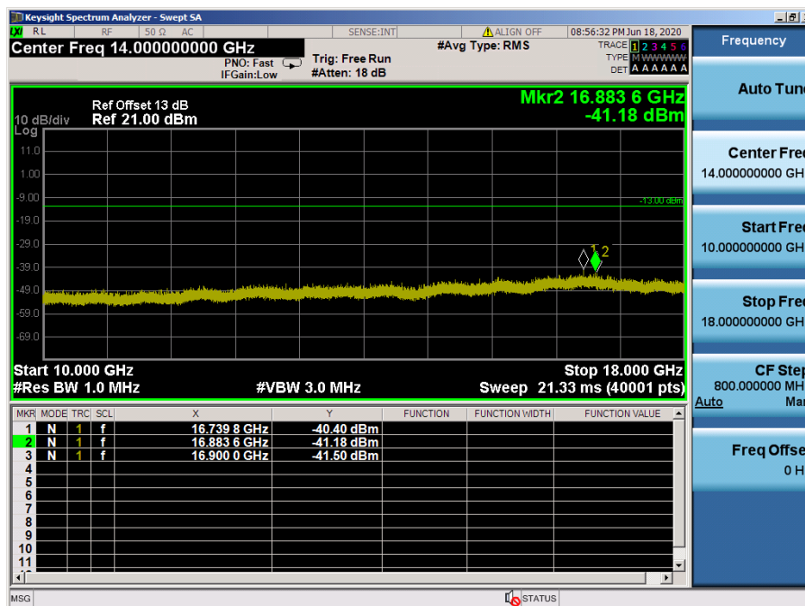
LTE Band 66, 4 / 1.4 MHz / 16QAM - RB Size/Offset (3/0) – High Channel
