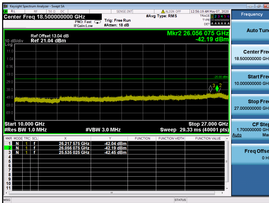
LTE Band 41 / 20 MHz / 64QAM - RB Size/Offset (1/50) – High Channel
