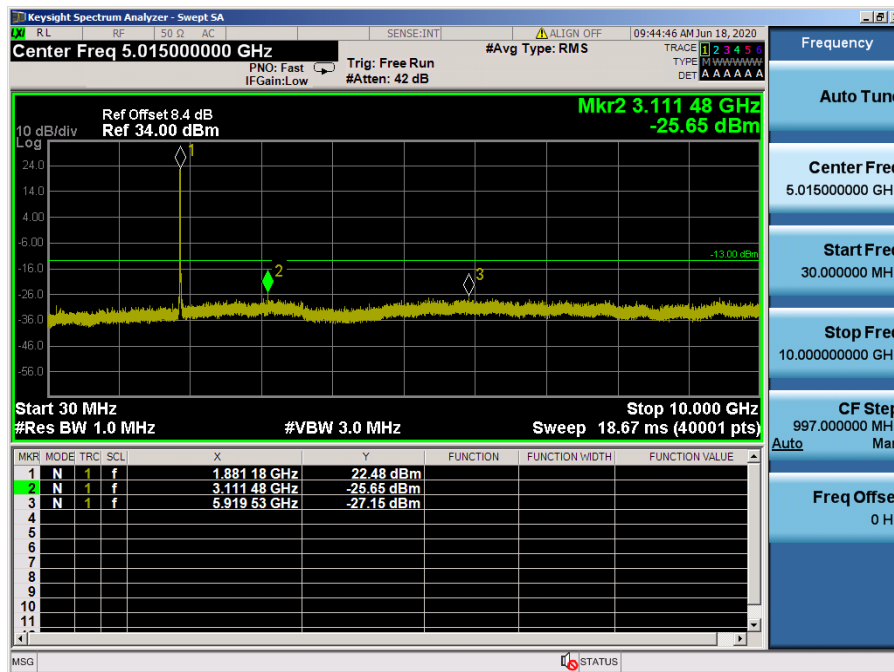
LTE Band 2 / 20 MHz / 64QAM - RB Size/Offset (50/50) – Mid Channel
