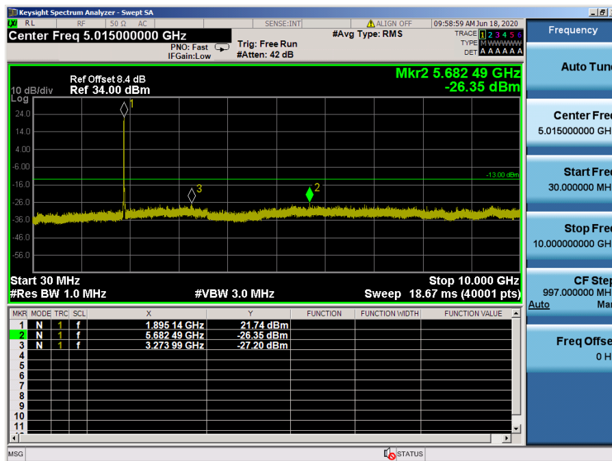
LTE Band 2 / 20 MHz / 64QAM - RB Size/Offset (50/0) – High Channel
