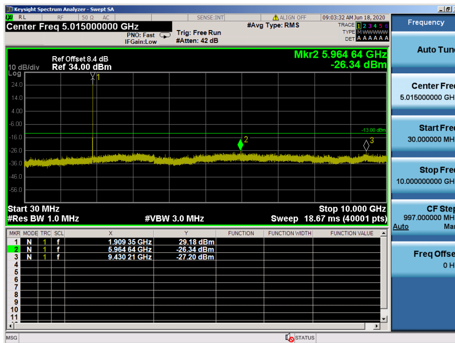
LTE Band 2 / 15 MHz / 64QAM - RB Size/Offset (1/74) – High Channel
