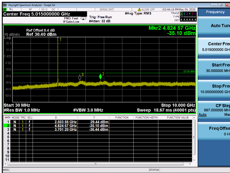
LTE Band 41 / 15 MHz / QPSK - RB Size/Offset (1/36) – Low Channel
