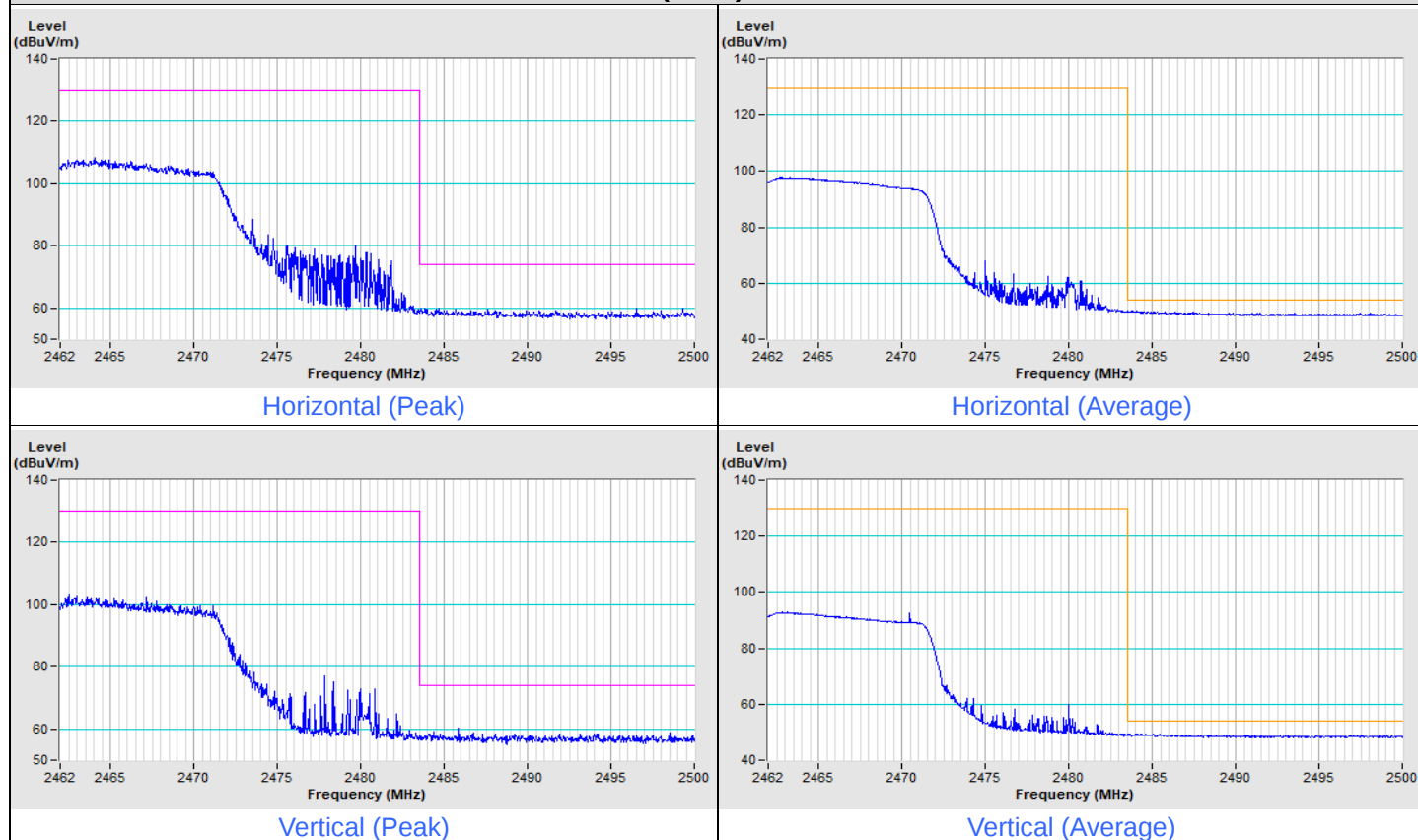
802.11ax (HE20) Channel 11
