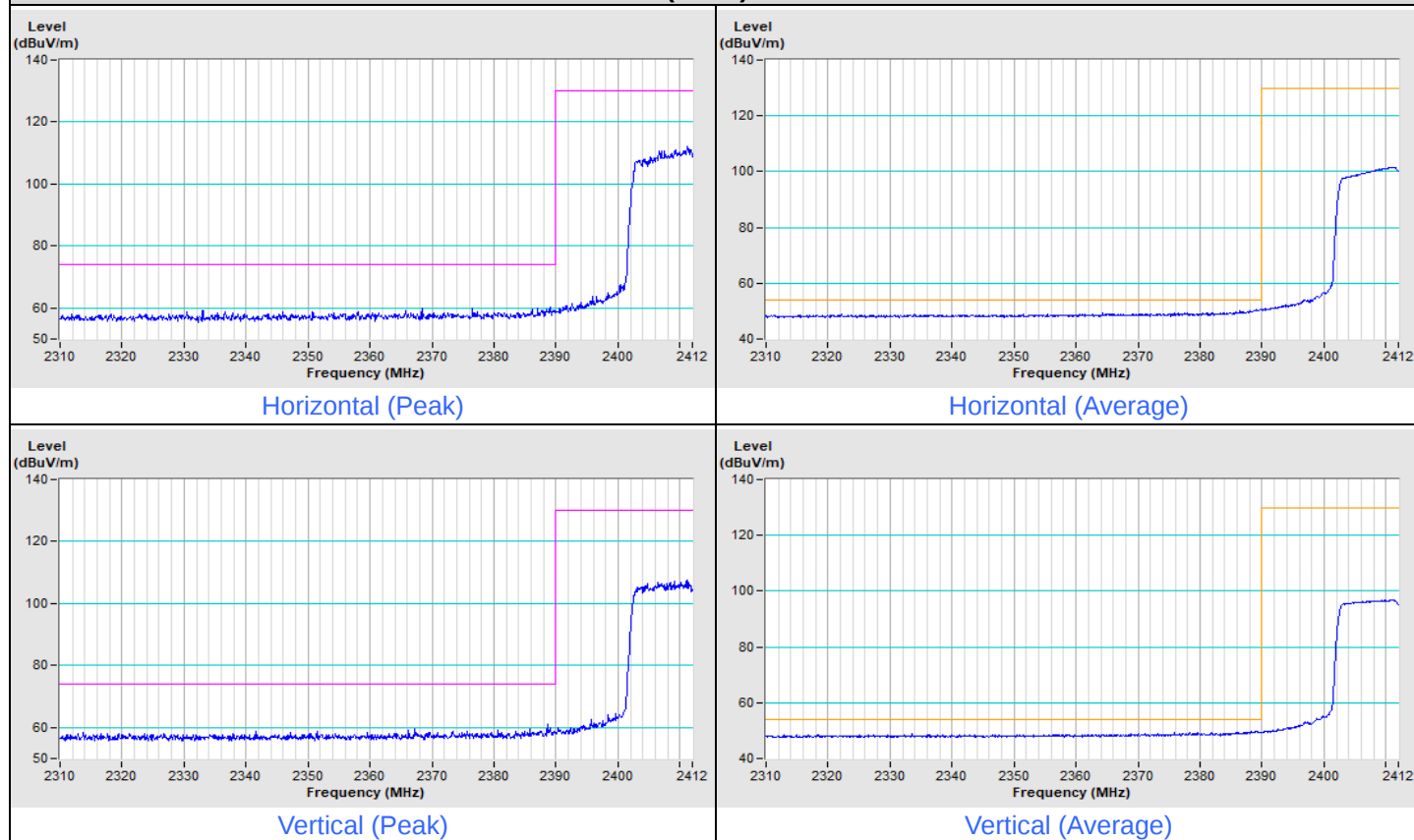
802.11ax (HE20) Channel 1
