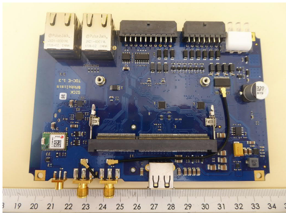
Main PCB, top view, WLAN / WPAN module removed
