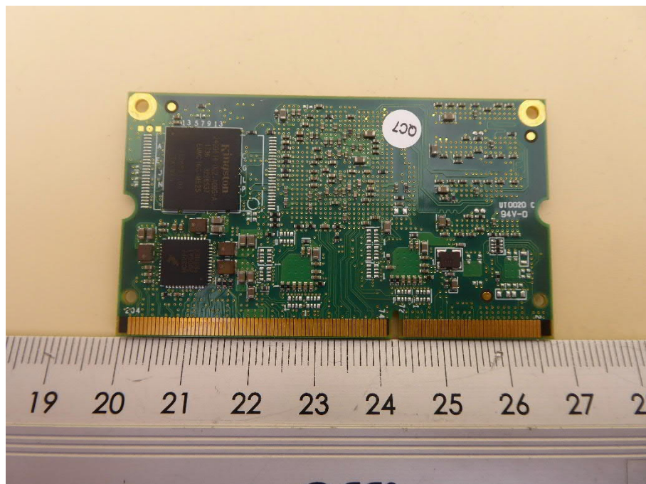
WLAN / WPAN module PCB, bottom view
