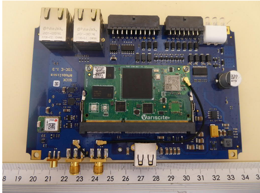
Main PCB, top view
