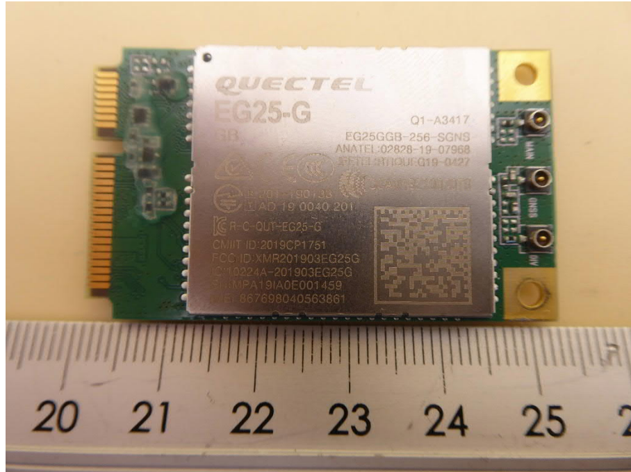
Cellular module PCB, top view
