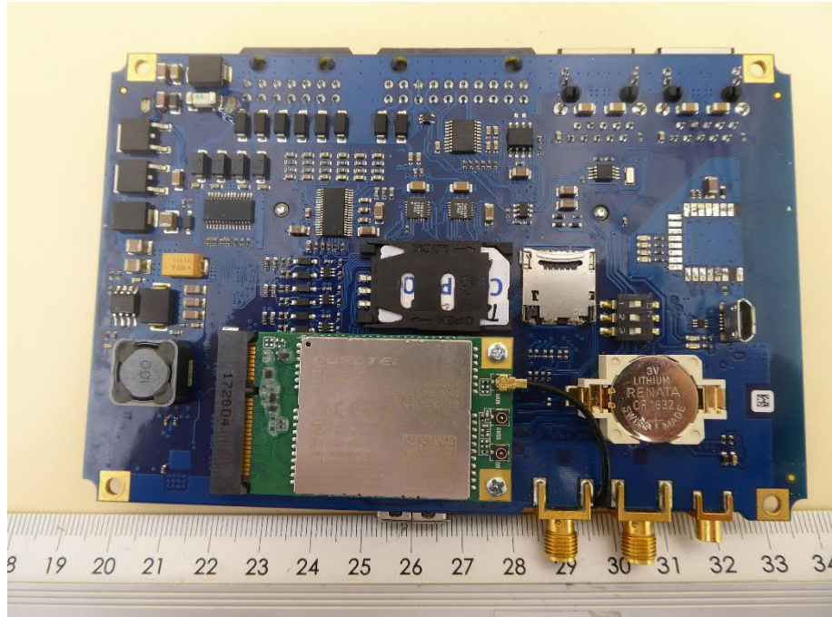
Main PCB, bottom view
