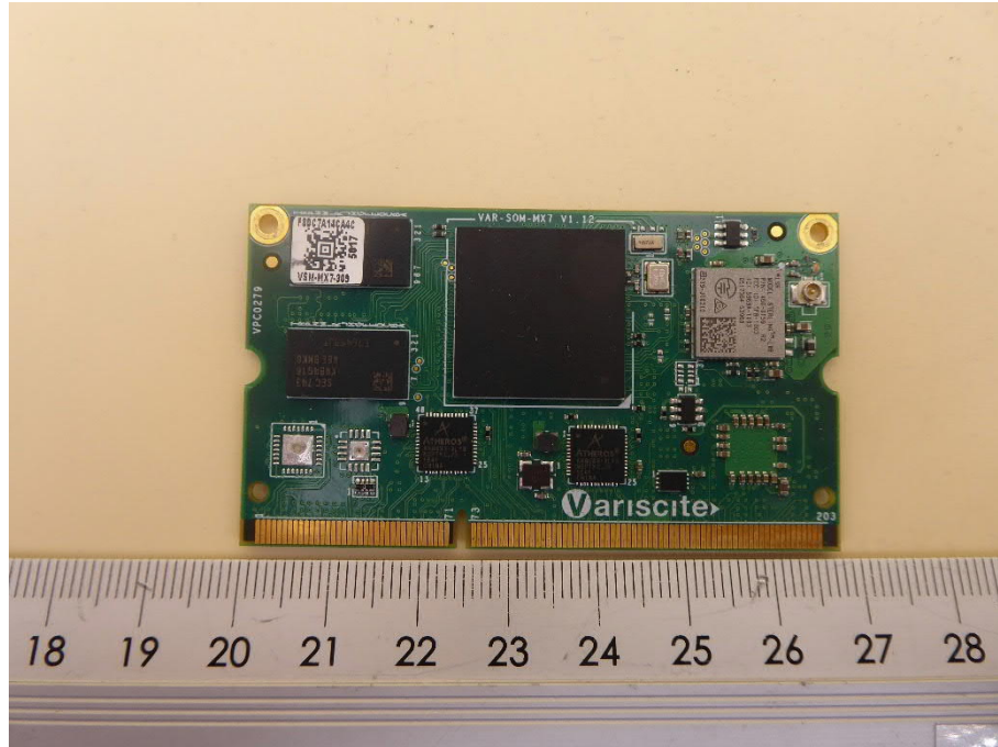
WLAN / WPAN module PCB, top view
