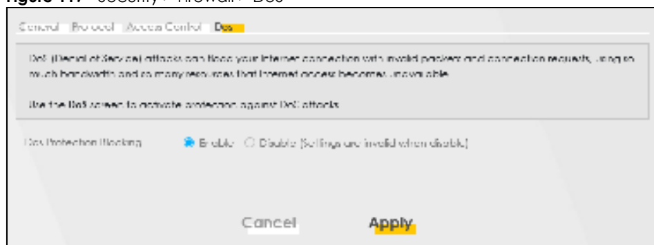
Figure 117 Security &gt; Firewall &gt; DoS
