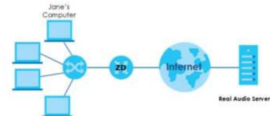
Figure 97 Trigger Port Forwarding Process: Example
