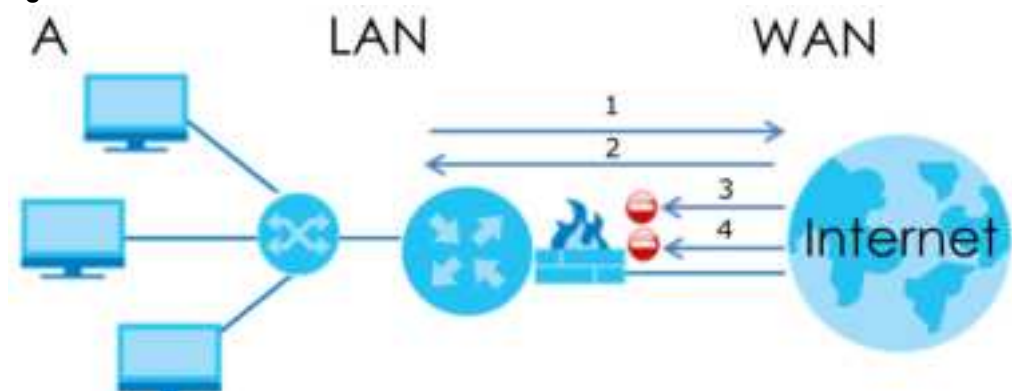
Figure 111 Default Firewall Action
