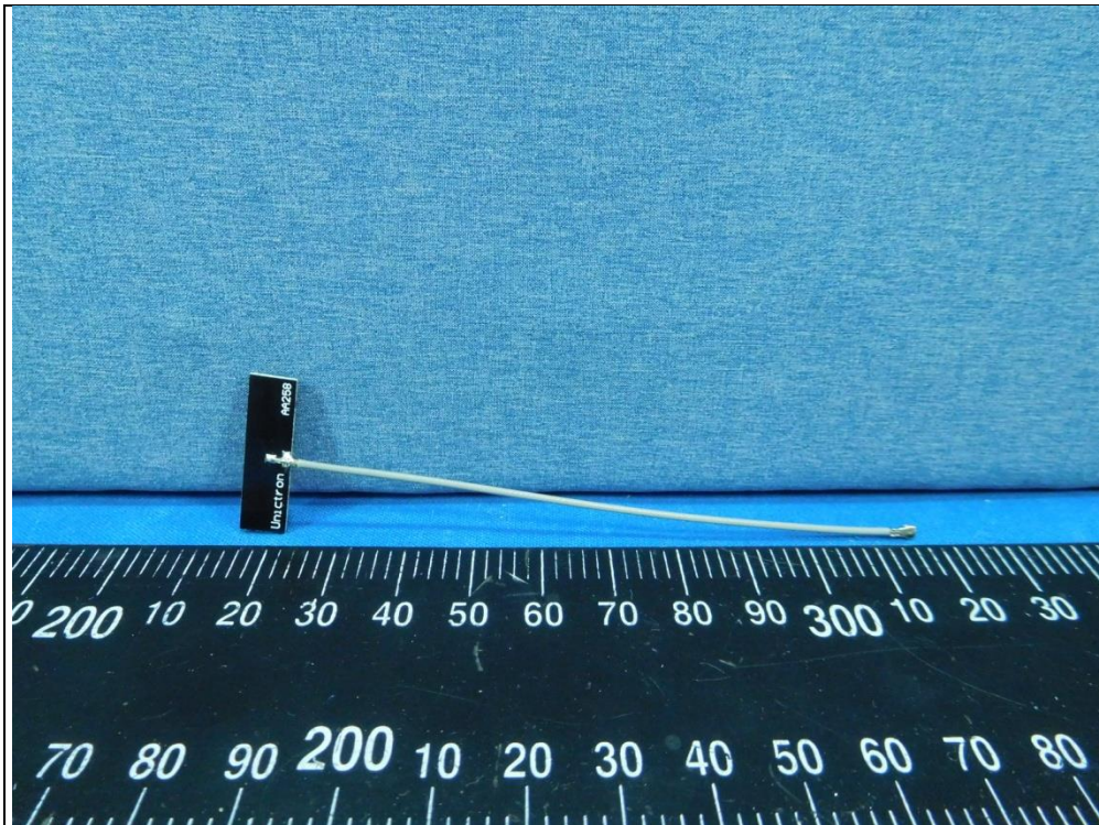
PCB Antenna (Brand: Unicttron / Model: H2B1PC1A1C175L)
