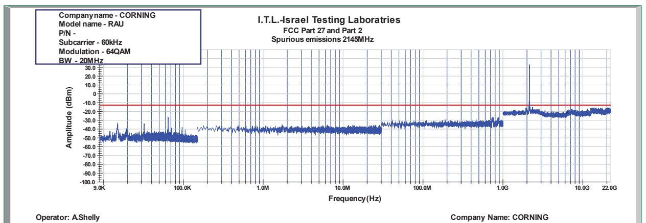
Figure 898: Spurious Emissions at Antenna Terminal 64QAM 20MHz B.W.; 2145.0MHz, 60kHz
