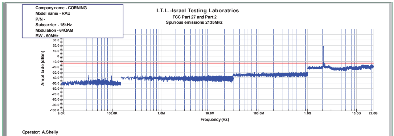
Figure 918: Spurious Emissions at Antenna Terminal 64QAM 50MHz B.W.; 2135.0MHz, 15kHz
