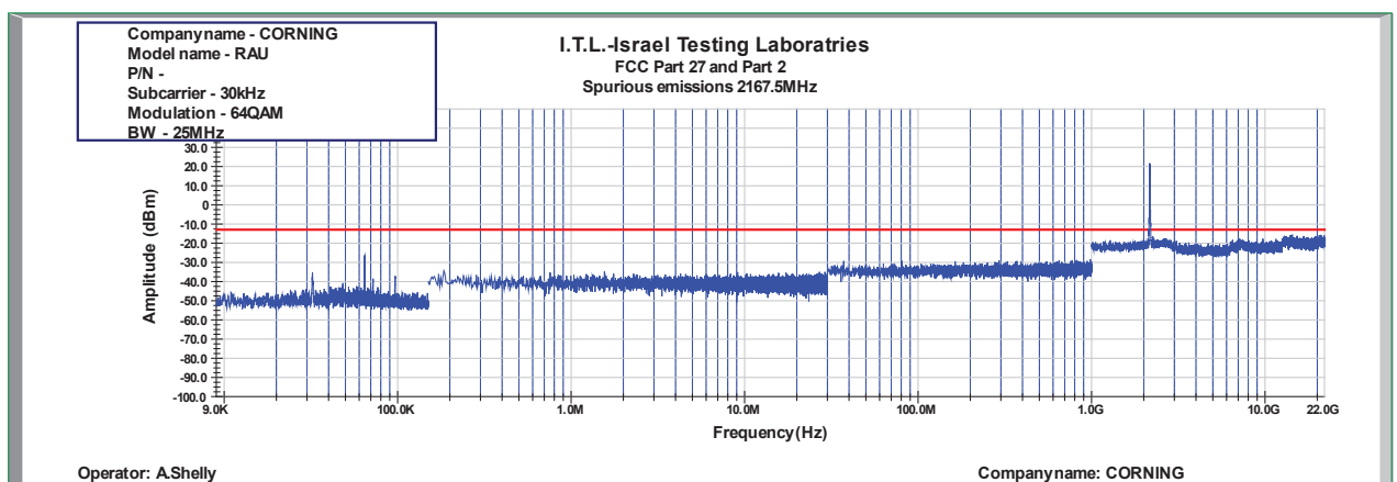
Figure 905: Spurious Emissions at Antenna Terminal 64QAM 25MHz B.W.; 2167.5MHz, 30kHz
