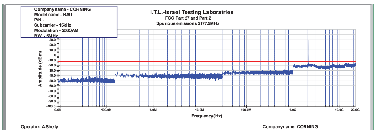
Figure 935: Spurious Emissions at Antenna Terminal 256QAM 5MHz B.W.; 2177.5MHz, 15kHz
