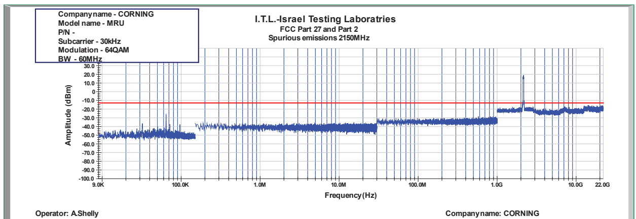
Figure 929: Spurious Emissions at Antenna Terminal 64QAM 60MHz B.W.; 2150.0MHz, 30kHz
