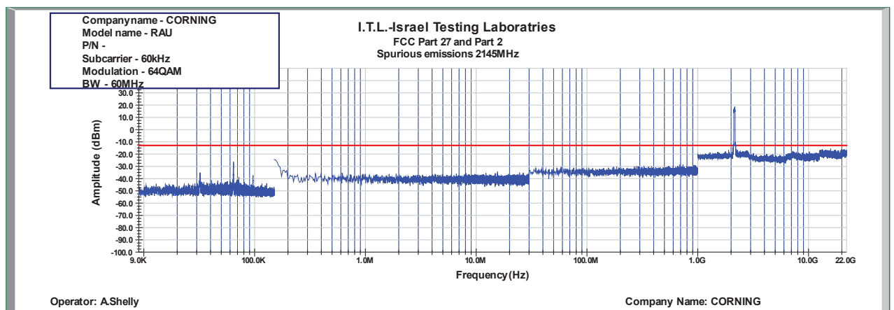
Figure 931: Spurious Emissions at Antenna Terminal 64QAM 60MHz B.W.; 2145.0MHz, 60kHz
