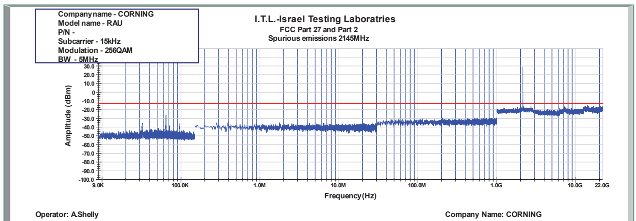
Figure 934: Spurious Emissions at Antenna Terminal 256QAM 5MHz B.W.; 2145.0MHz, 15kHz
