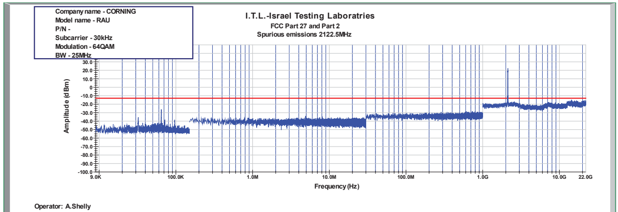
Figure 903: Spurious Emissions at Antenna Terminal 64QAM 25MHz B.W.; 2122.5MHz, 30kHz
