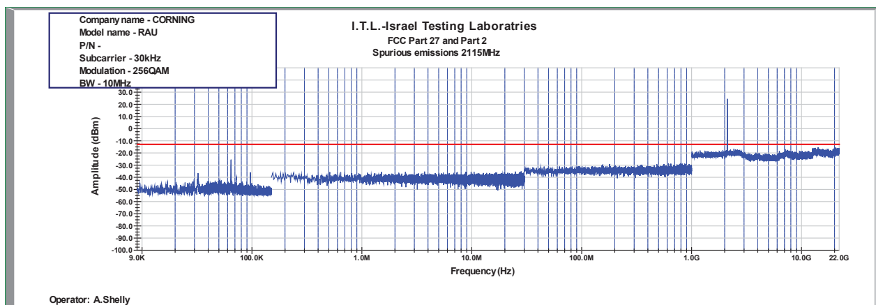
Figure 942: Spurious Emissions at Antenna Terminal 256QAM 10MHz B.W.; 2115.0MHz, 30kHz
