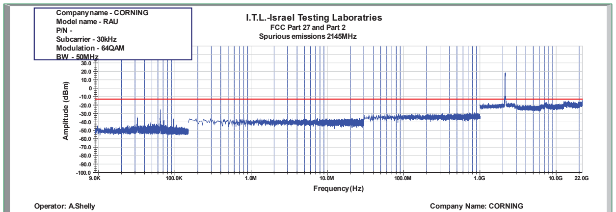
Figure 922: Spurious Emissions at Antenna Terminal 64QAM 50MHz B.W.; 2145.0MHz, 30kHz
