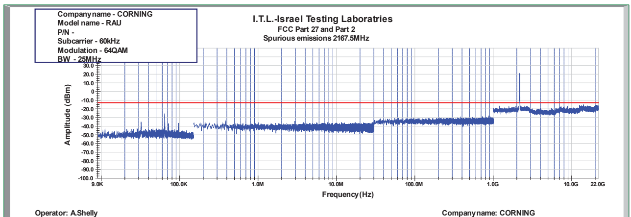
Figure 908: Spurious Emissions at Antenna Terminal 64QAM 25MHz B.W.; 2167.5MHz, 60kHz
