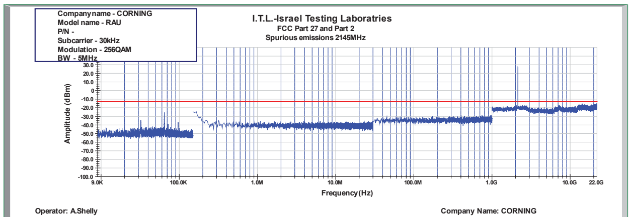
Figure 937: Spurious Emissions at Antenna Terminal 256QAM 5MHz B.W.; 2145.0MHz, 30kHz
