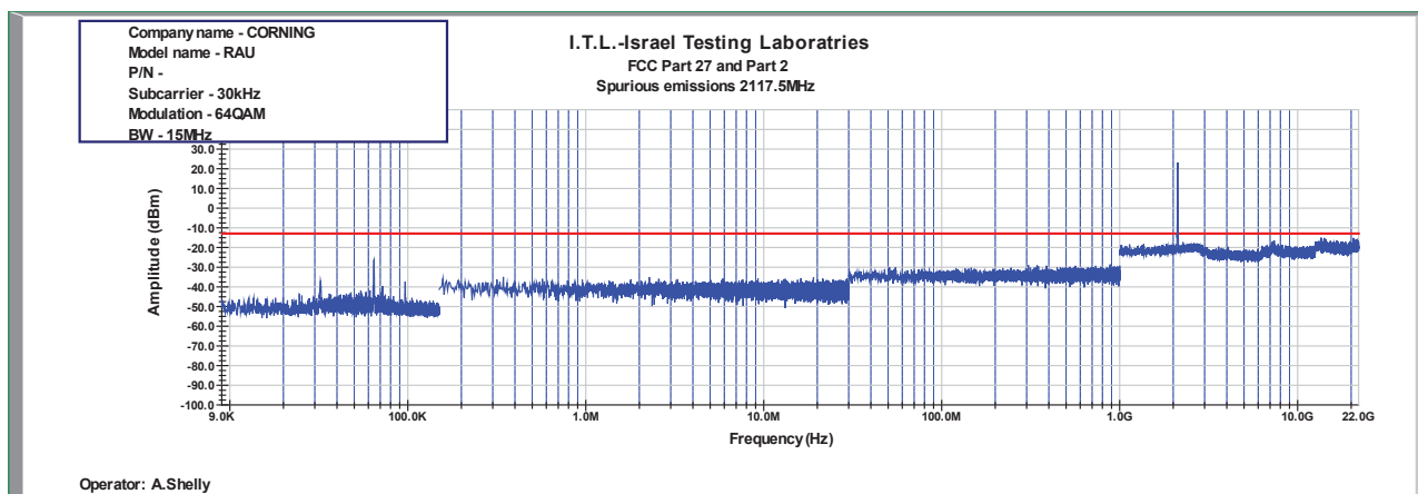
Figure 885: Spurious Emissions at Antenna Terminal 64QAM 15MHz B.W.; 2117.5MHz, 30kHz
