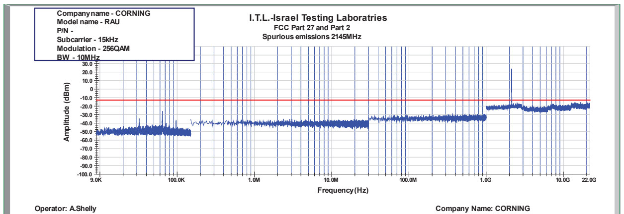
Figure 940: Spurious Emissions at Antenna Terminal 256QAM 10MHz B.W.; 2145.0MHz, 15kHz
