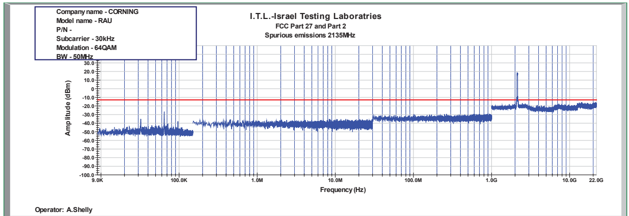
Figure 921: Spurious Emissions at Antenna Terminal 64QAM 50MHz B.W.; 2135.0MHz, 30kHz
