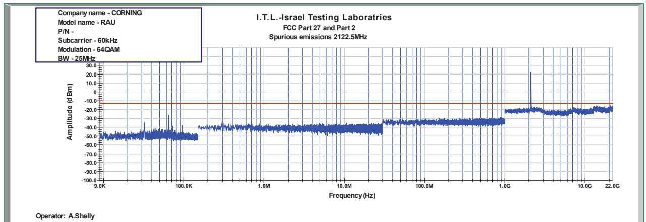
Figure 906: Spurious Emissions at Antenna Terminal 64QAM 25MHz B.W.; 2122.5MHz, 60kHz
