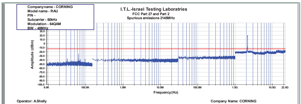
Figure 916: Spurious Emissions at Antenna Terminal 64QAM 40MHz B.W.; 2145.0MHz, 60kHz
