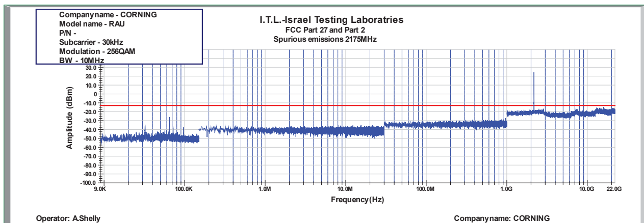
Figure 944: Spurious Emissions at Antenna Terminal 256QAM 10MHz B.W.; 2175.0MHz, 30kHz
