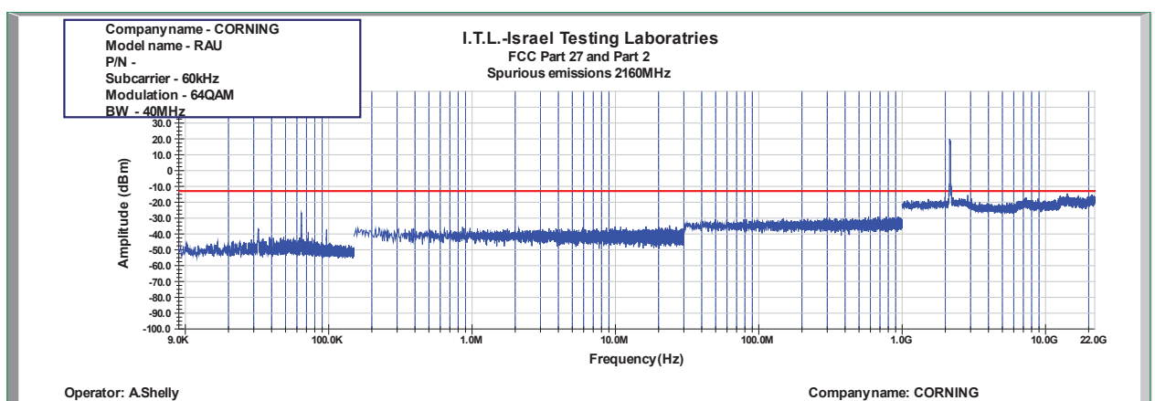
Figure 917: Spurious Emissions at Antenna Terminal 64QAM 40MHz B.W.; 2160.0MHz, 60kHz
