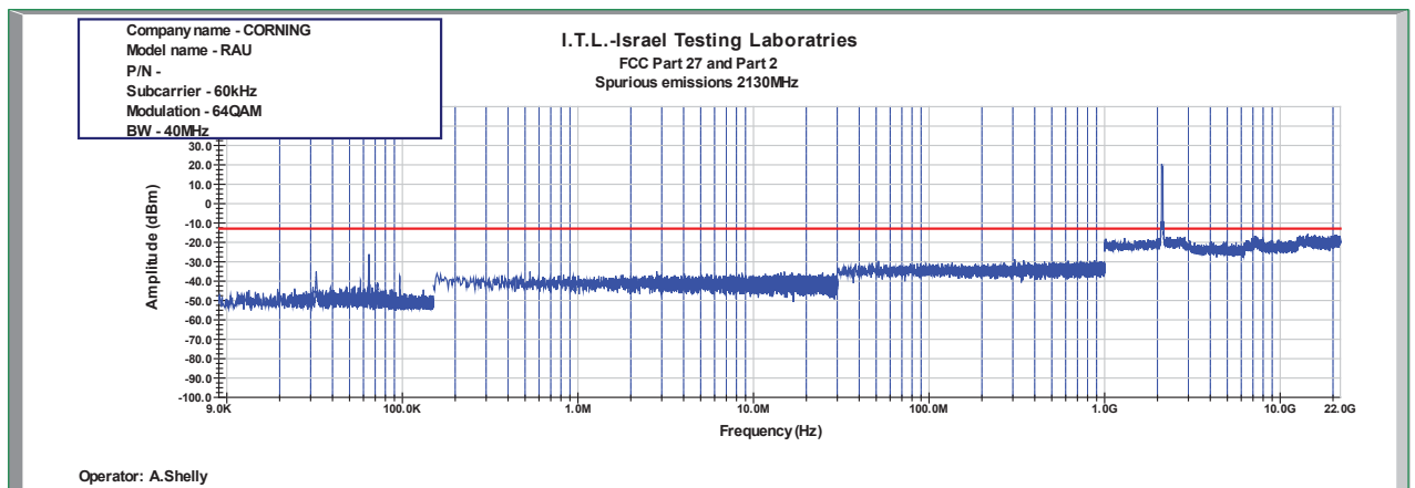
Figure 915: Spurious Emissions at Antenna Terminal 64QAM 40MHz B.W.; 2130.0MHz, 60kHz
