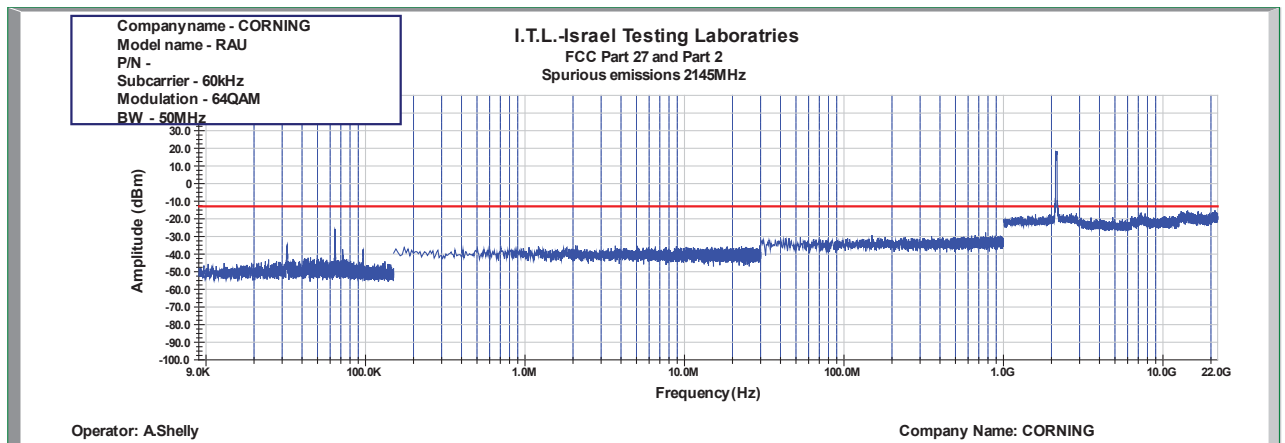
Figure 925: Spurious Emissions at Antenna Terminal 64QAM 50MHz B.W.; 2145.0MHz, 60kHz
