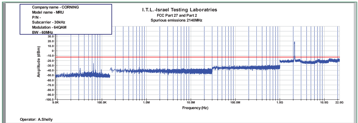
Figure 927: Spurious Emissions at Antenna Terminal 64QAM 60MHz B.W.; 2140.0MHz, 30kHz
