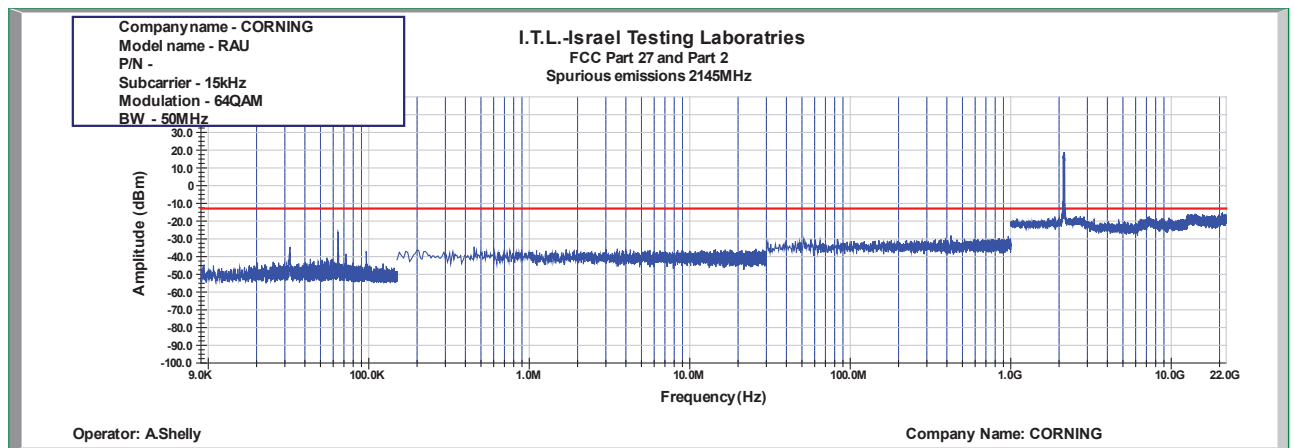
Figure 919: Spurious Emissions at Antenna Terminal 64QAM 50MHz B.W.; 2145.0MHz, 15kHz
