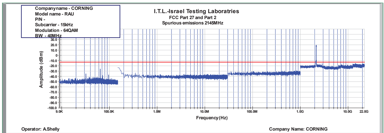
Figure 910: Spurious Emissions at Antenna Terminal 64QAM 40MHz B.W.; 2145.0MHz, 15kHz
