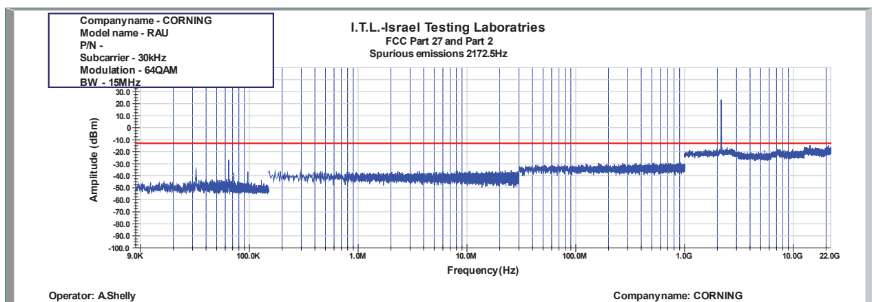
Figure 890: Spurious Emissions at Antenna Terminal 64QAM 15MHz B.W.; 2172.5MHz, 30kHz
