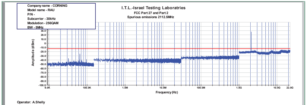
Figure 936: Spurious Emissions at Antenna Terminal 256QAM 5MHz B.W.; 2112.5MHz, 30kHz
