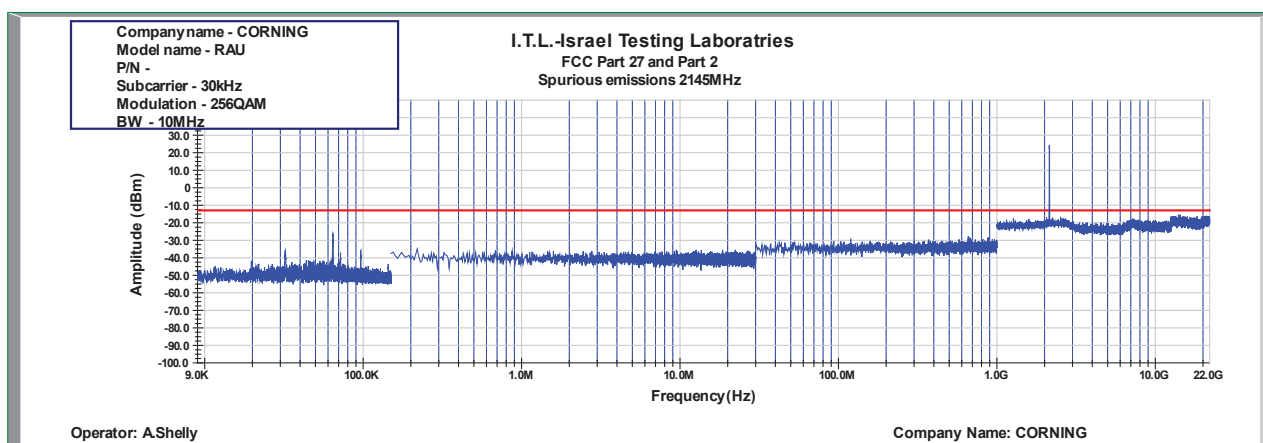
Figure 943: Spurious Emissions at Antenna Terminal 256QAM 10MHz B.W.; 2145.0MHz, 30kHz
