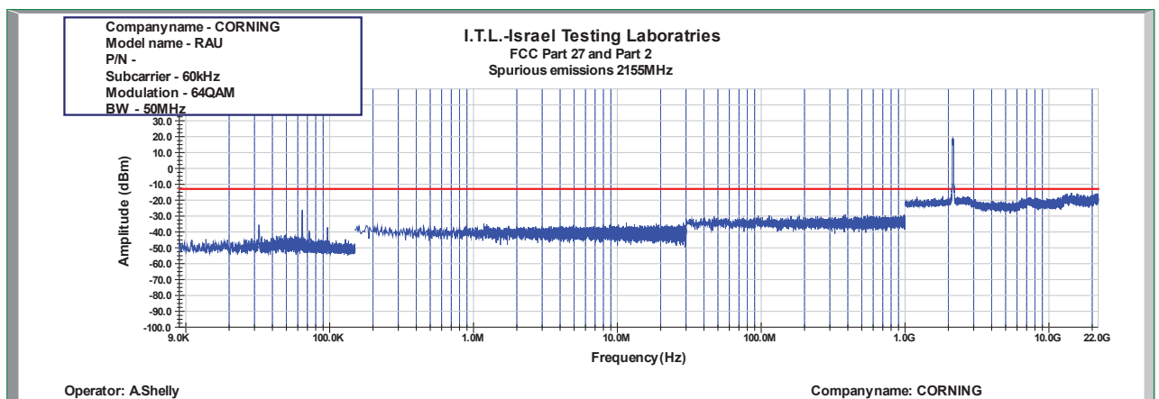
Figure 926: Spurious Emissions at Antenna Terminal 64QAM 50MHz B.W.; 2155.0MHz, 60kHz
