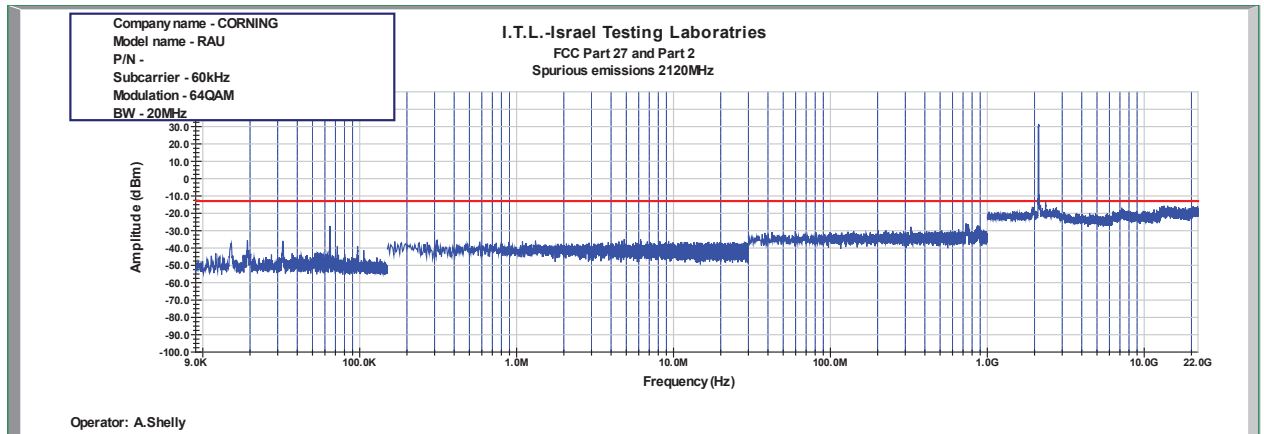
Figure 897: Spurious Emissions at Antenna Terminal 64QAM 20MHz B.W.; 2120.0MHz, 60kHz
