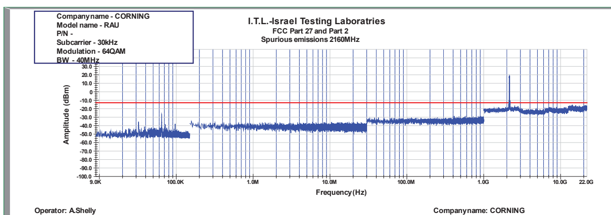
Figure 914: Spurious Emissions at Antenna Terminal 64QAM 40MHz B.W.; 2160.0MHz, 30kHz
