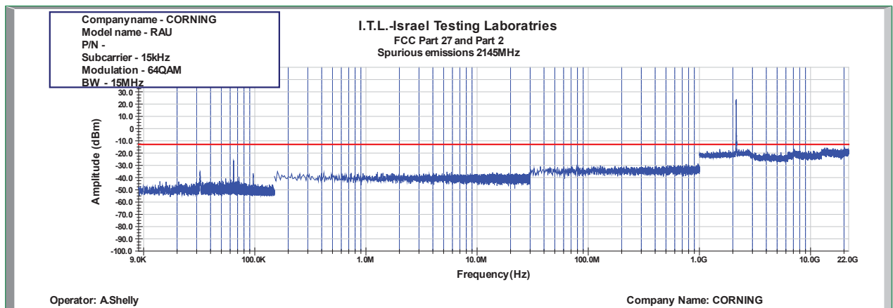
Figure 883: Spurious Emissions at Antenna Terminal 64QAM 15MHz B.W.; 2145.0MHz, 15kHz
