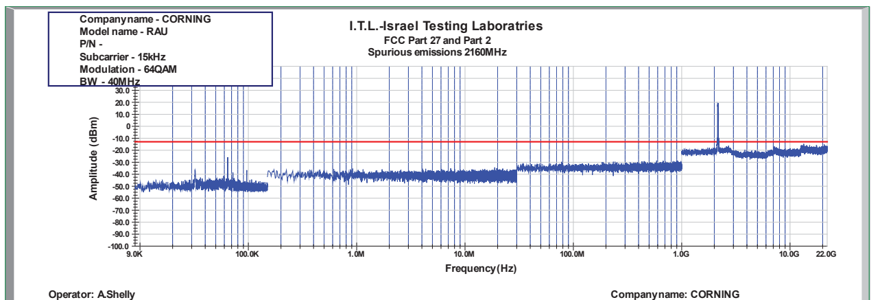
Figure 911: Spurious Emissions at Antenna Terminal 64QAM 40MHz B.W.; 2160.0MHz, 15kHz
