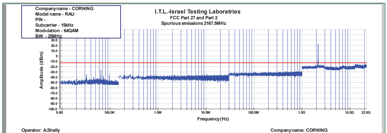
Figure 902: Spurious Emissions at Antenna Terminal 64QAM 25MHz B.W.; 2167.5MHz, 15kHz
