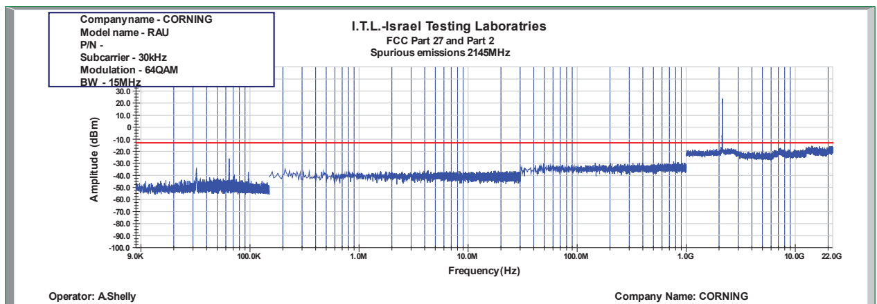
Figure 889: Spurious Emissions at Antenna Terminal 64QAM 15MHz B.W.; 2145.0MHz, 30kHz
