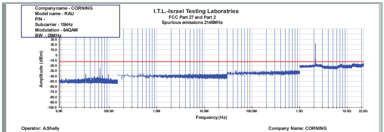
Figure 901: Spurious Emissions at Antenna Terminal 64QAM 25MHz B.W.; 2145.0MHz, 15kHz
