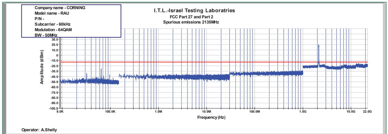
Figure 924: Spurious Emissions at Antenna Terminal 64QAM 50MHz B.W.; 2135.0MHz, 60kHz
