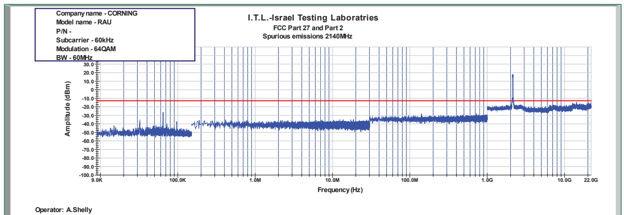
Figure 930: Spurious Emissions at Antenna Terminal 64QAM 60MHz B.W.; 2140.0MHz, 60kHz
