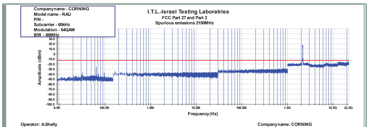
Figure 932: Spurious Emissions at Antenna Terminal 64QAM 60MHz B.W.; 2150.0MHz, 60kHz
