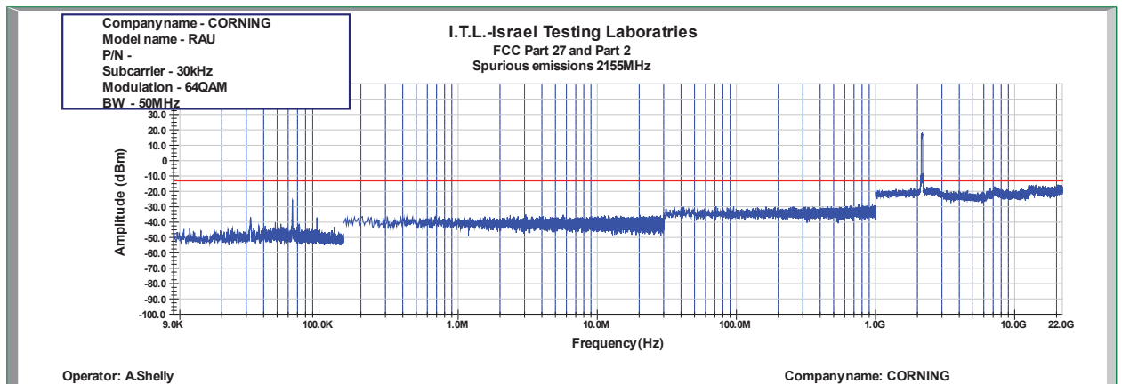
Figure 923: Spurious Emissions at Antenna Terminal 64QAM 50MHz B.W.; 2155.0MHz, 30kHz
