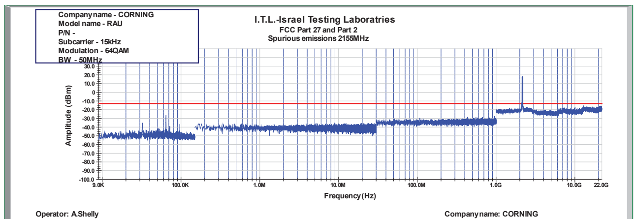
Figure 920: Spurious Emissions at Antenna Terminal 64QAM 50MHz B.W.; 2155.0MHz, 15kHz
