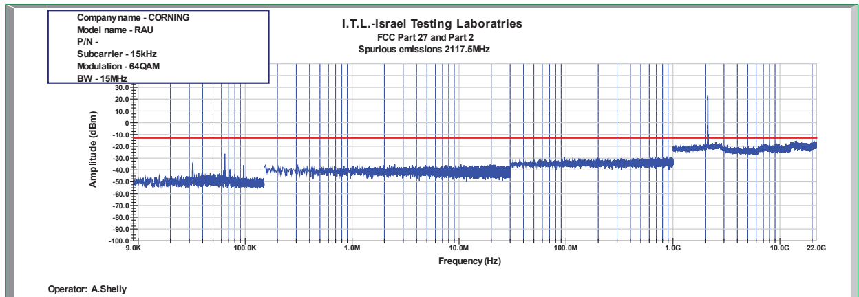
Figure 882: Spurious Emissions at Antenna Terminal 64QAM 15MHz B.W.; 2117.5MHz, 15kHz
