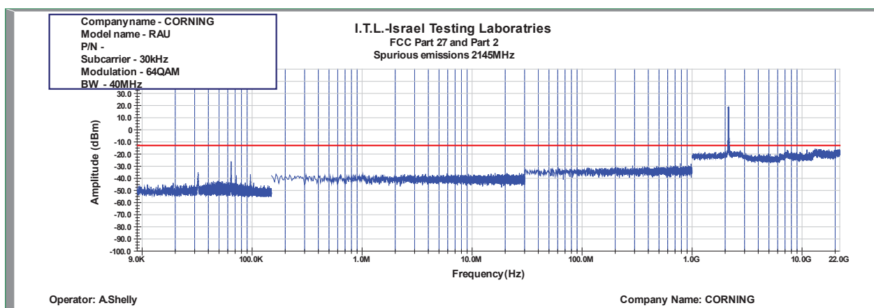
Figure 913: Spurious Emissions at Antenna Terminal 64QAM 40MHz B.W.; 2145.0MHz, 30kHz
