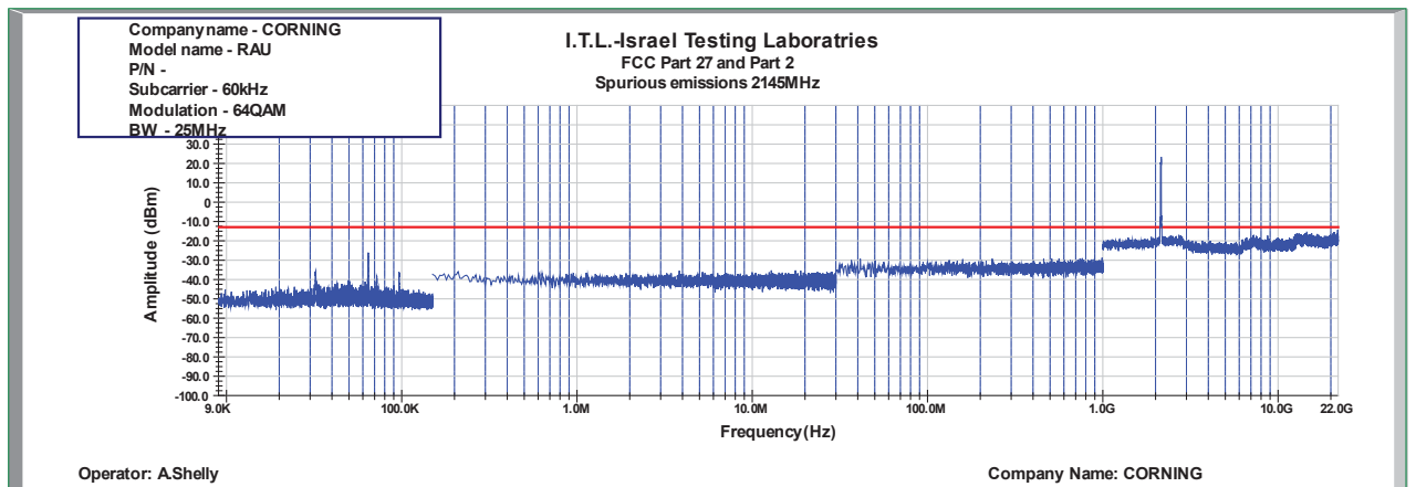
Figure 907: Spurious Emissions at Antenna Terminal 64QAM 25MHz B.W.; 2145.0MHz, 60kHz
