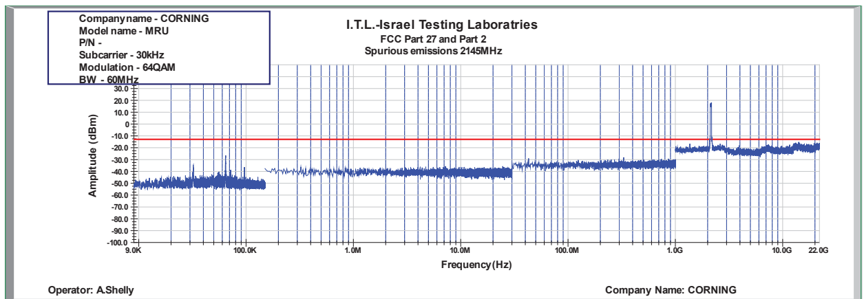
Figure 928: Spurious Emissions at Antenna Terminal 64QAM 60MHz B.W.; 2145.0MHz, 30kHz
