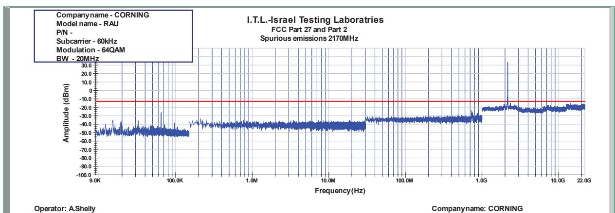
Figure 899: Spurious Emissions at Antenna Terminal 64QAM 20MHz B.W.; 2170.0MHz, 60kHz
