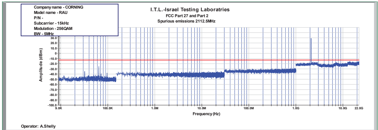
Figure 933: Spurious Emissions at Antenna Terminal 256QAM 5MHz B.W.; 2112.5MHz, 15kHz
