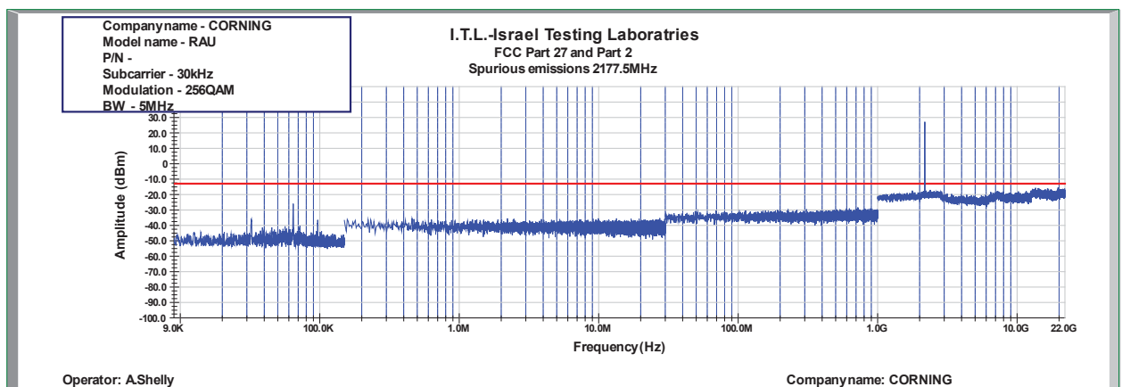
Figure 938: Spurious Emissions at Antenna Terminal 256QAM 5MHz B.W.; 2177.5MHz, 30kHz
