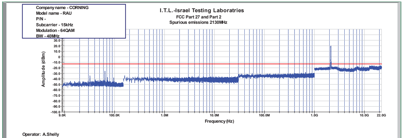
Figure 909: Spurious Emissions at Antenna Terminal 64QAM 40MHz B.W.; 2130.0MHz, 15kHz
