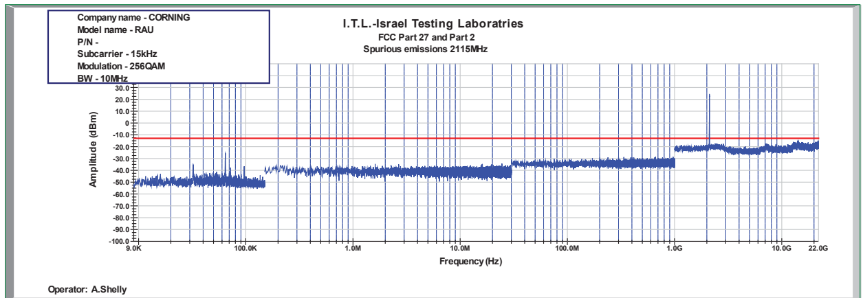
Figure 939: Spurious Emissions at Antenna Terminal 256QAM 10MHz B.W.; 2115.0MHz, 15kHz
