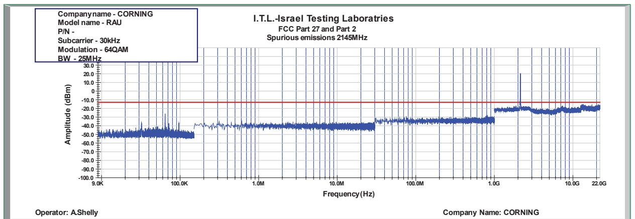
Figure 904: Spurious Emissions at Antenna Terminal 64QAM 25MHz B.W.; 2145.0MHz, 30kHz
