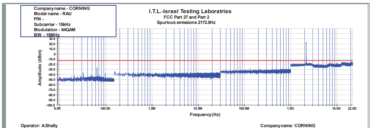
Figure 884: Spurious Emissions at Antenna Terminal 64QAM 15MHz B.W.; 2172.5MHz, 15kHz
