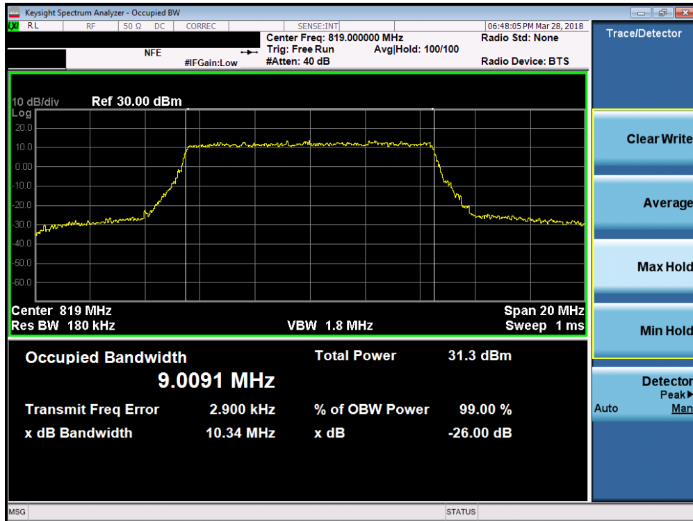
Plot 7-13. Occupied Bandwidth Plot (LTE Band 26 - 10MHz 64-QAM – RB Size 50)
