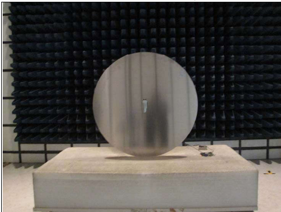
LTE Band 4, 12, 13, 26 Radiated Emission Test below 1GHz
