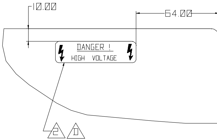
VIEW C
