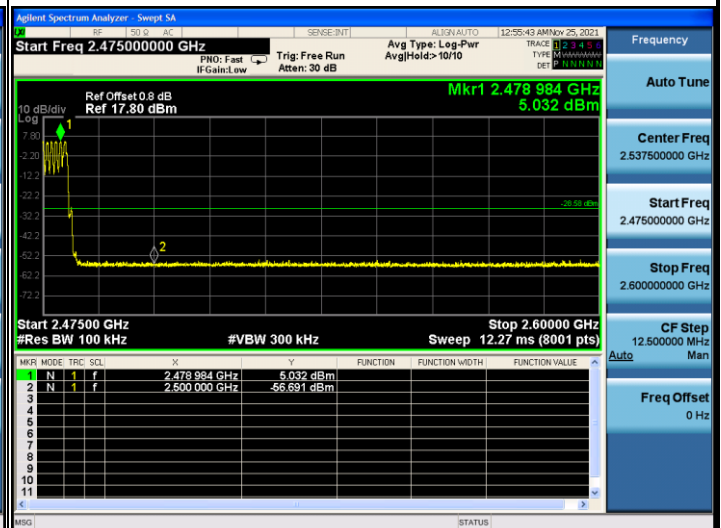
Mode 4 (2DH5-1)
