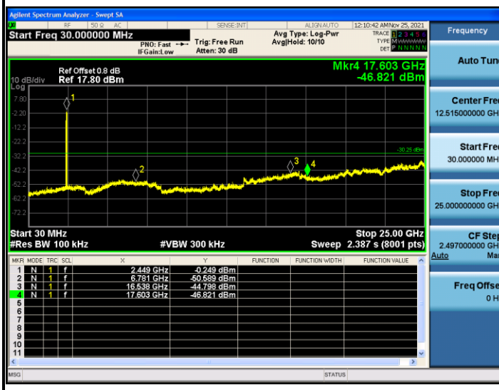
Mode 4 (2DH5-1)
