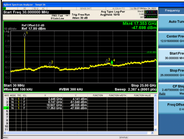
Mode 4 (2DH5-1)
