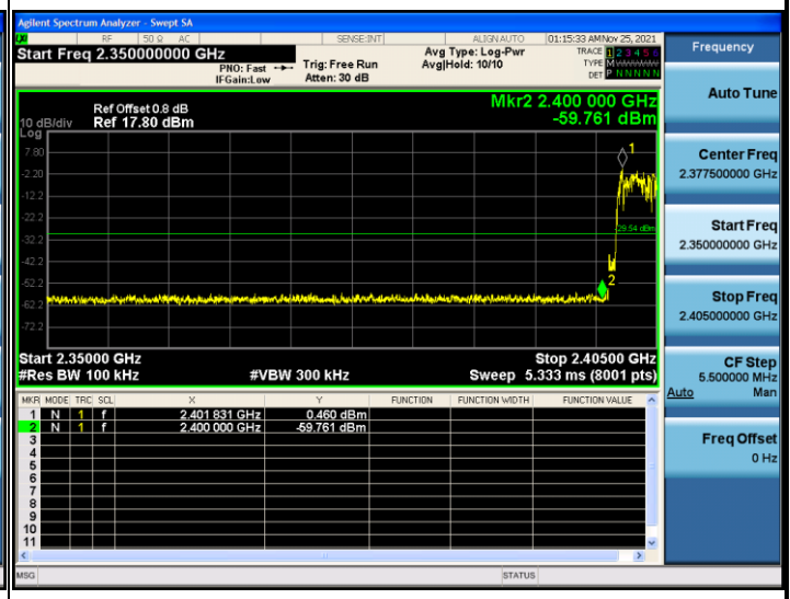
Mode 4 (2DH5-1)
