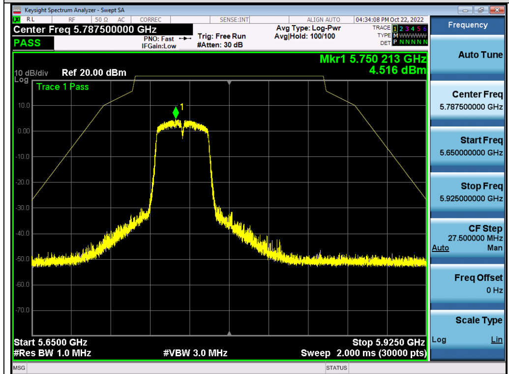
Test_Graph_802.11n40_ANT2_5755_MCS0_Frequency Band3
