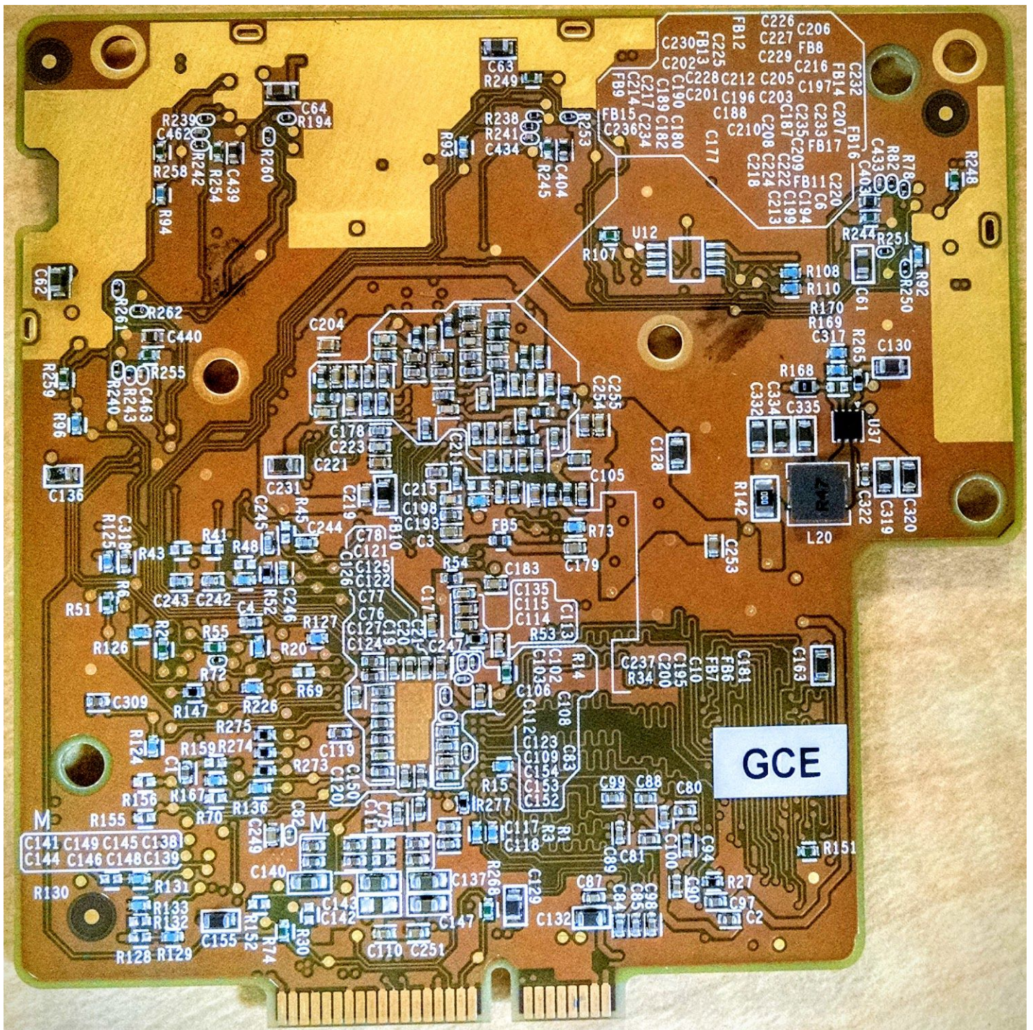
5GHz WiFi module - bottom view
