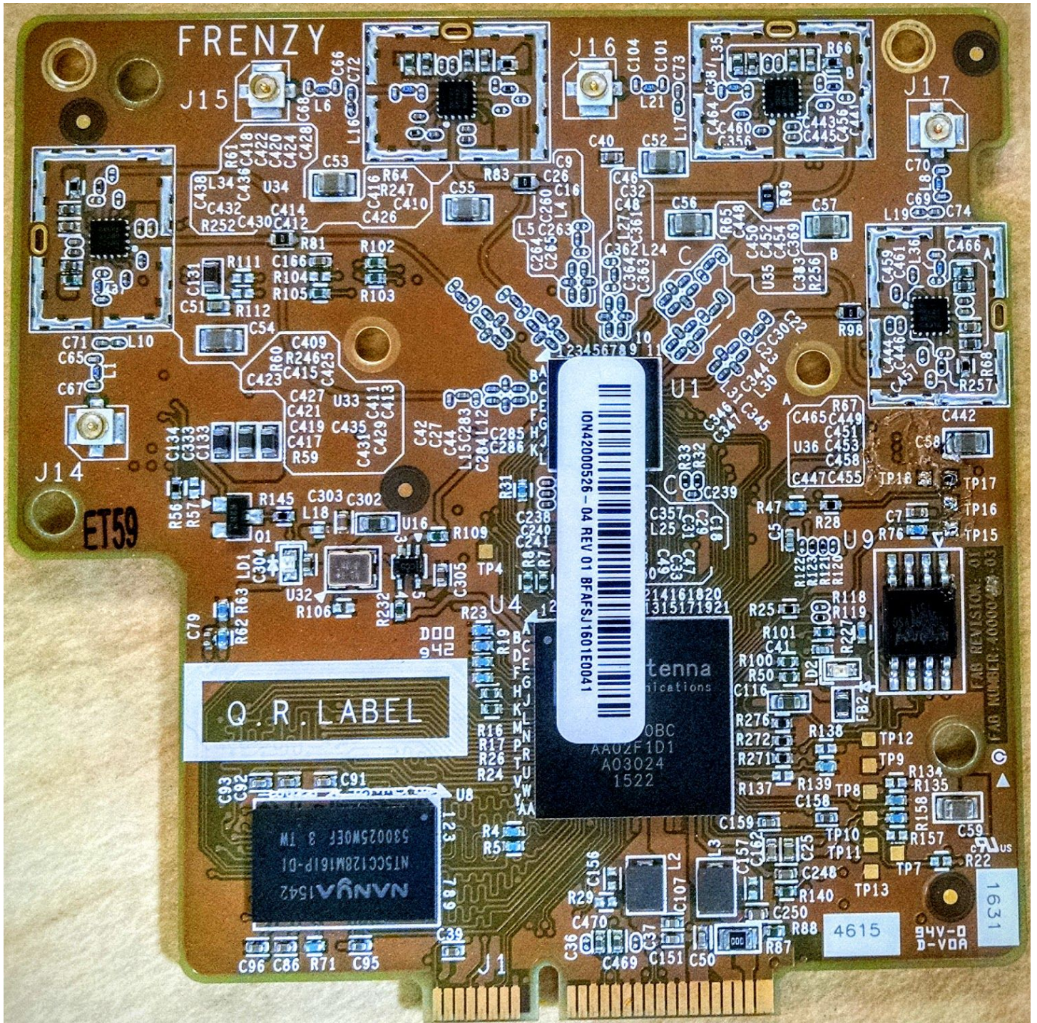
5GHz WiFi module - top view
