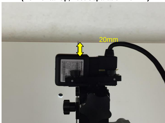
(Vertical Front, Test Separation 20 mm)
