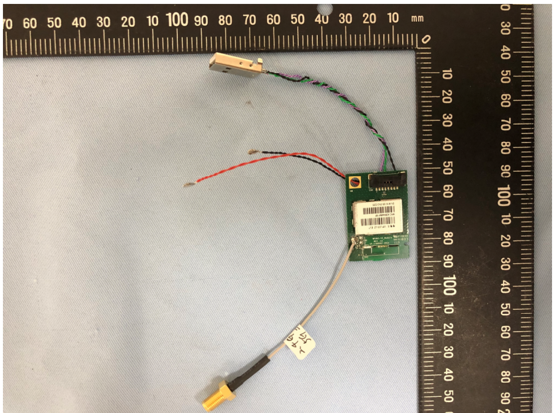
Conducted tested sample
