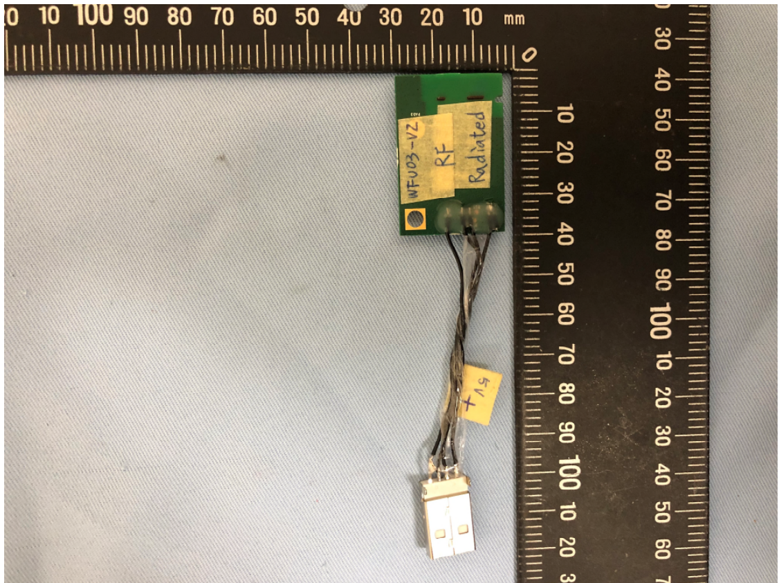
Radiated tested sample
